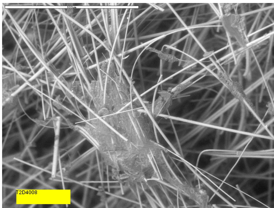
Figure J-8. Test-2 Day-4 SEM image, overview of a new area of dry sample #1 (T2D4008).
