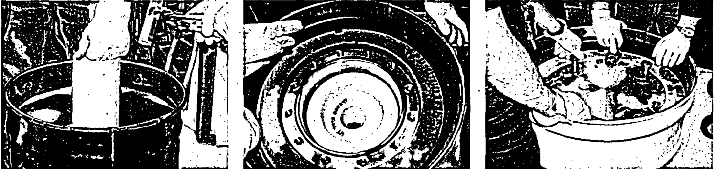
Figure 2: Source Recovery Project Personnel Remove a Sealed Radiological Source and Repackage It Into a WIPP-Acceptable Disposal Drum
