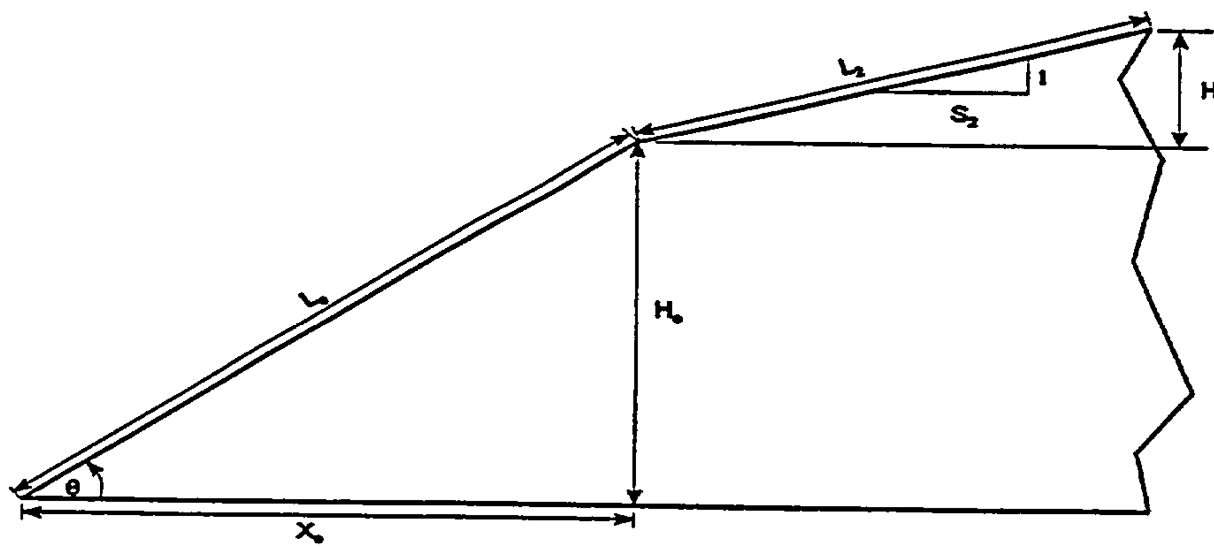
Type 2 Embankment
