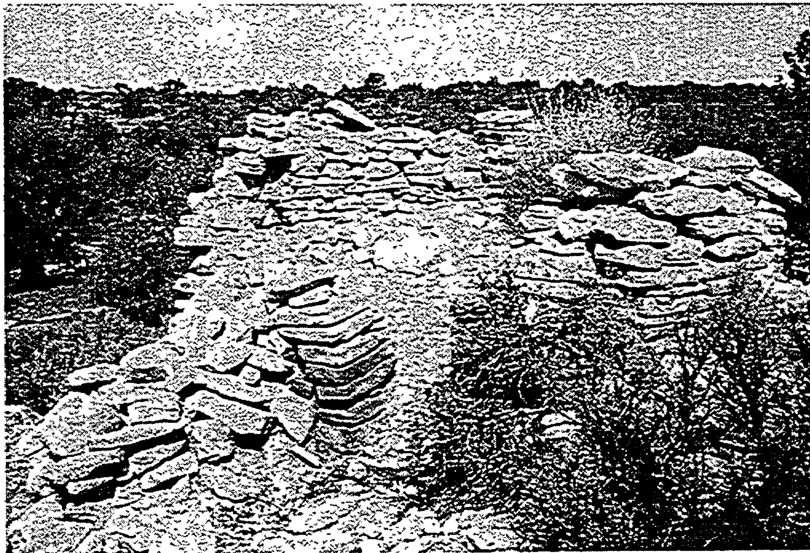
Figure D-3. Sandstone ruin near Durango, Colorado.
