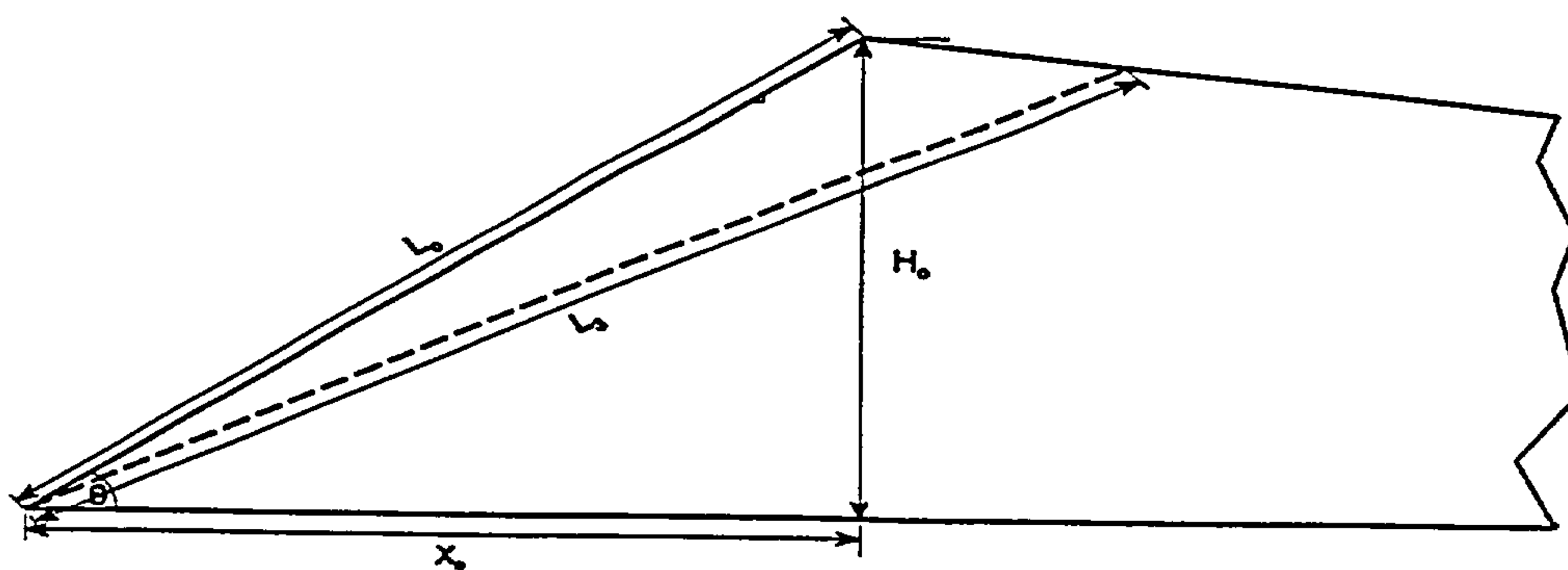
Type 3 Embankment
