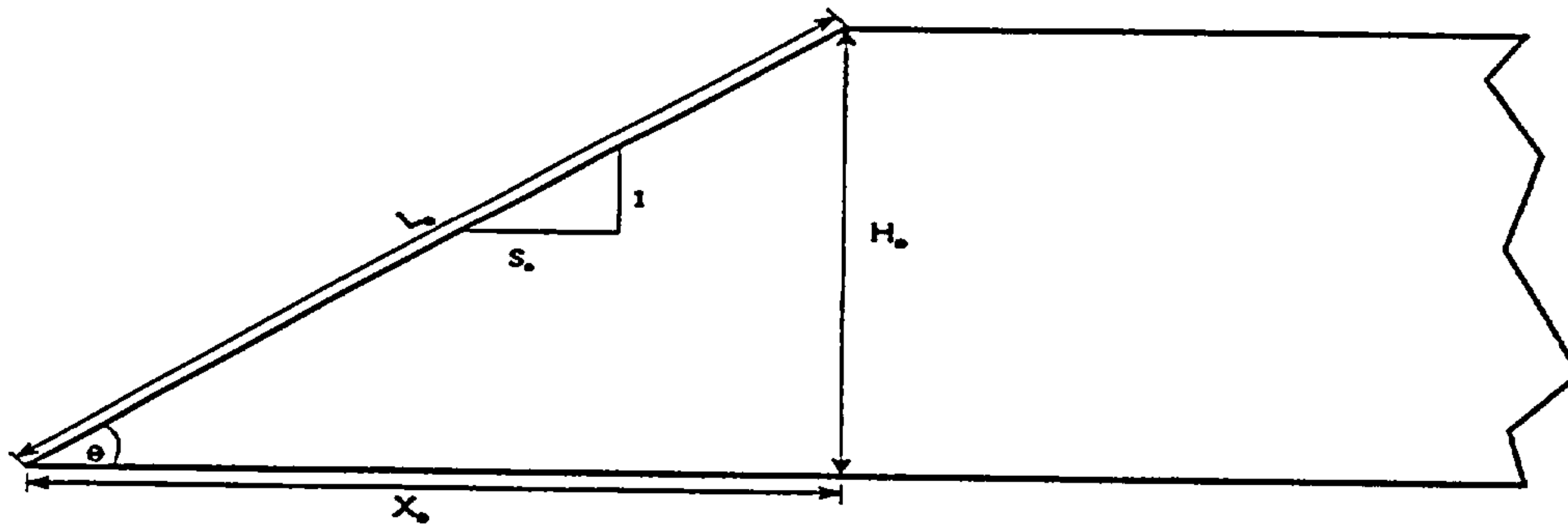
Type 1 Embankment
