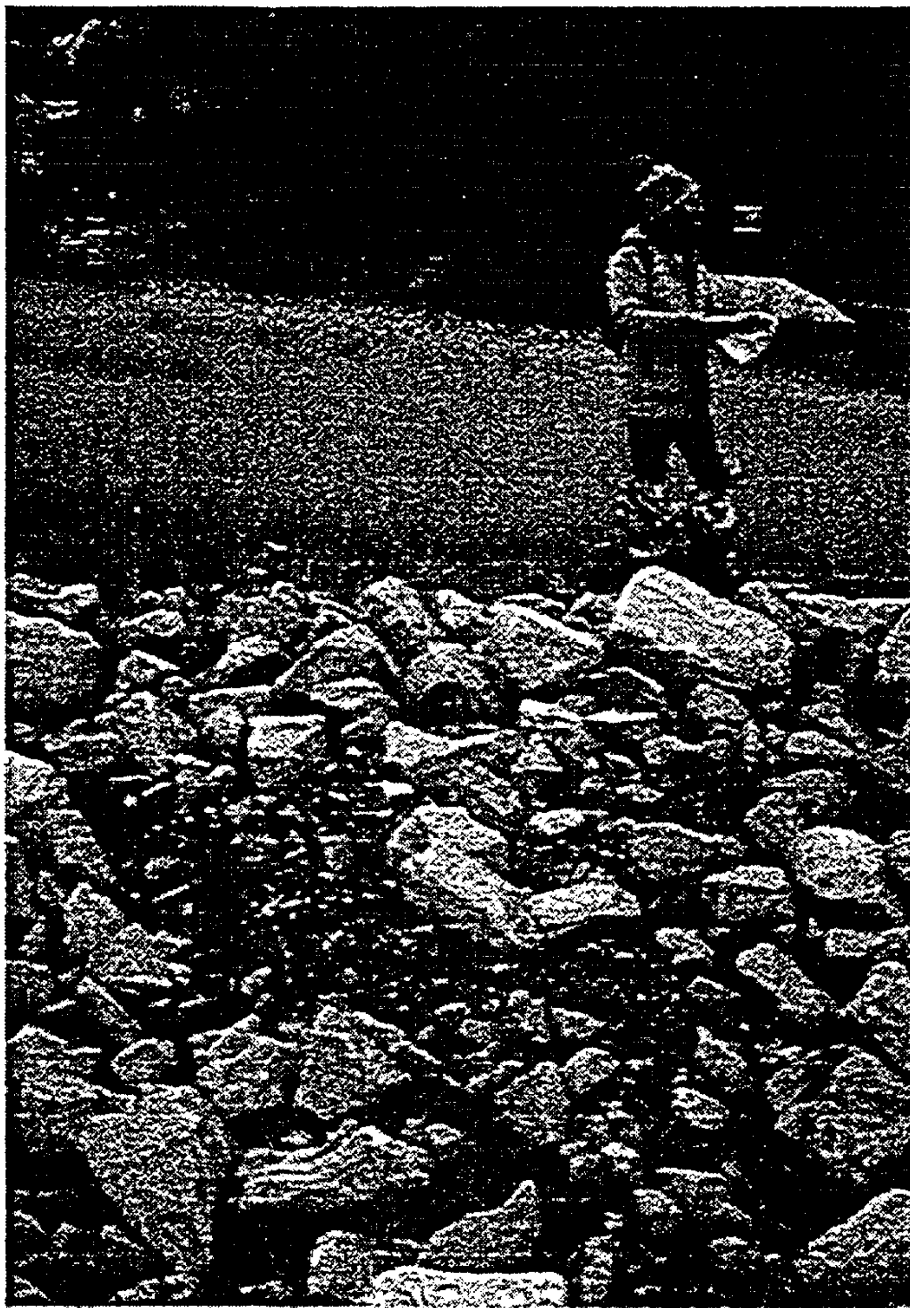
Figure F-1. Poorly-placed riprap.
