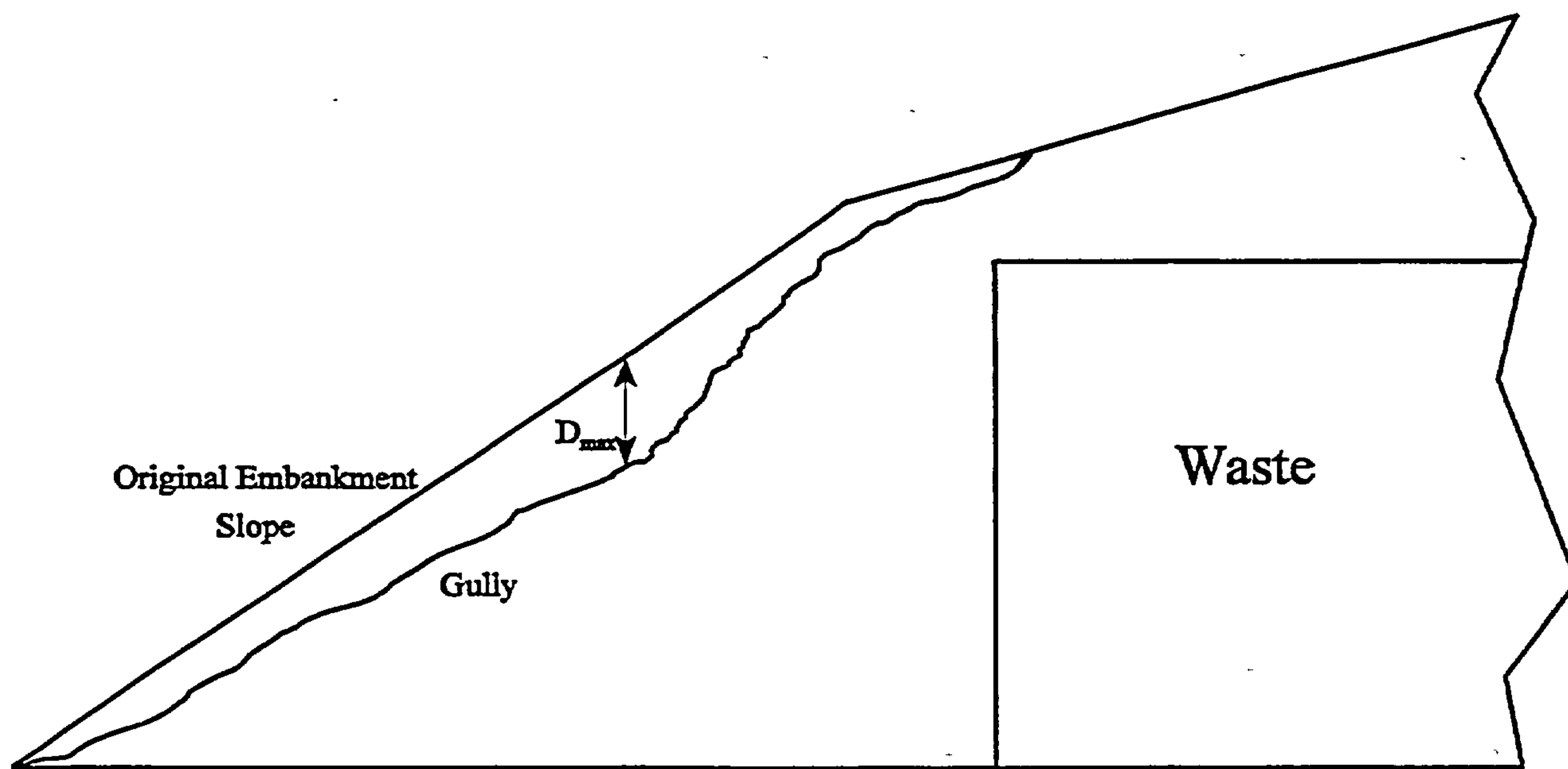
Figure B-5. Schematic of typical waste impoundment.
