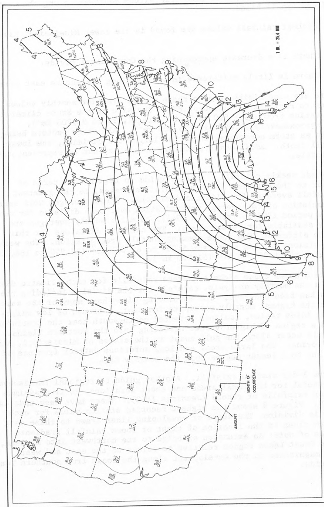
Figure 8. ---Envelope of greatest average weekly precipitation (in.) for State climatic divisions (1906-35).
