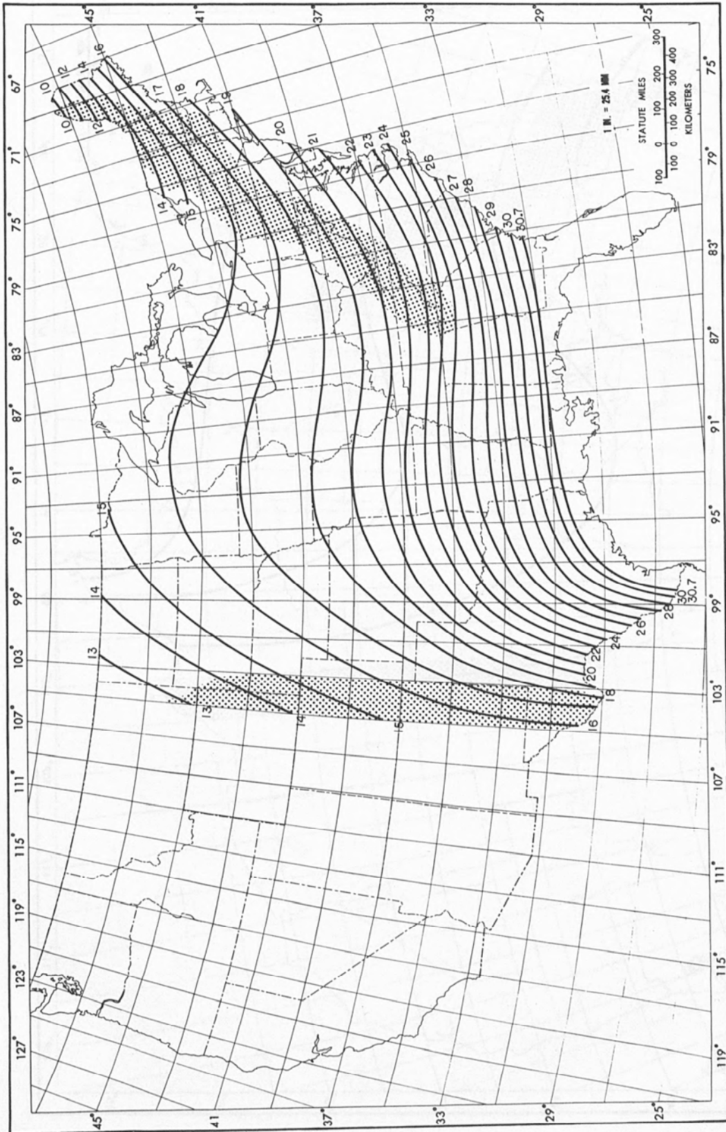
Figure 37.--All-season PMP (in.) for 72 hr 5,000 mi 2 (12,950 km 2 ).
