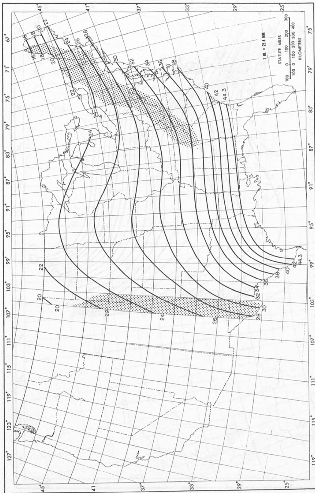
Figure 26.--All-season PMP (in.) for 48 hr 200 mi 2 (518 km 2 ).
