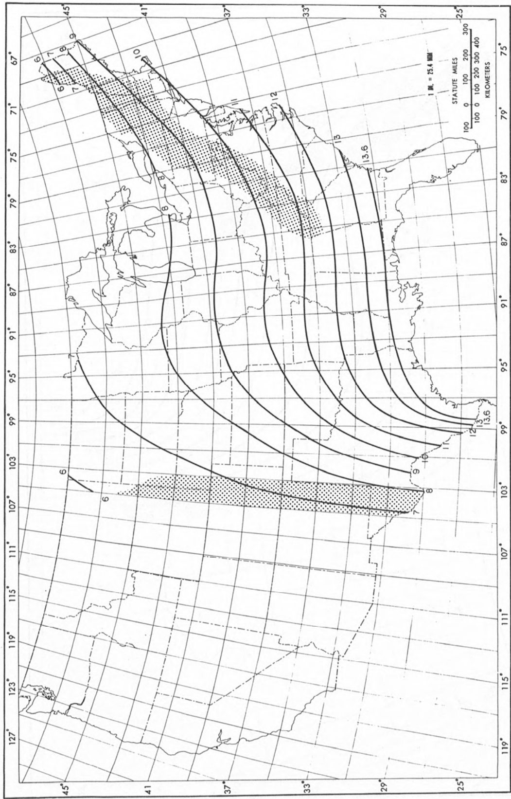
Figure 45.--All-season FMP (in.) for 24 hr 20,000 mi 2 (51,800 km 2 ).
