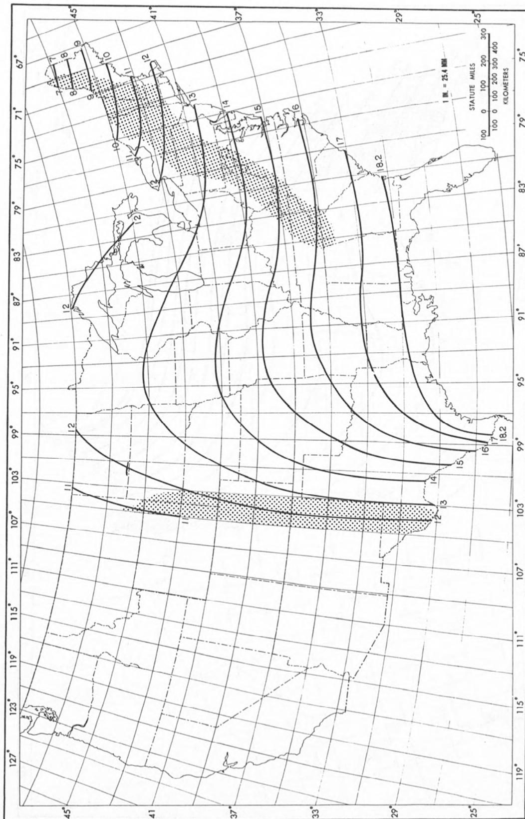
Figure 28.--All-season PMP (in.) for 6 hr 1,000 mi 2 (2,590 km 2 ).
