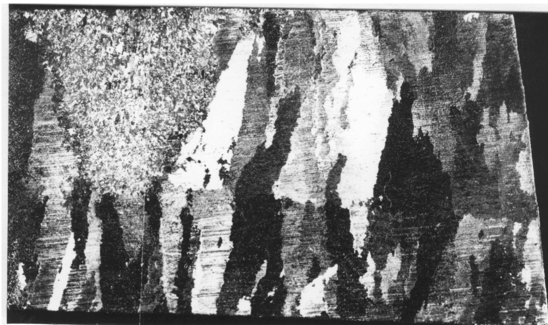
Figure 3. Microstructure along axial section of Loop B main shutoff valve from the Shippingport reactor. A repair weld is also seen on the outer diameter of the valve.
