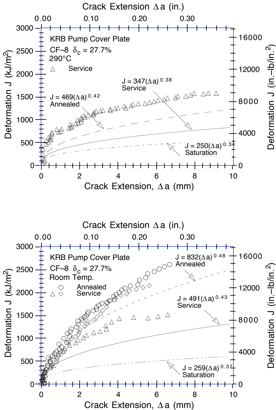
Figure 38. Estimated and measured fracture toughness J - R curve for the KRB pump cover plate in the annealed or unaged condition, after service, and at saturation. (Dashed, solid, and chain-dot lines are the estimated power-law J - R curves for annealed, service-aged, and fully embrittled or aged material, respectively.)
