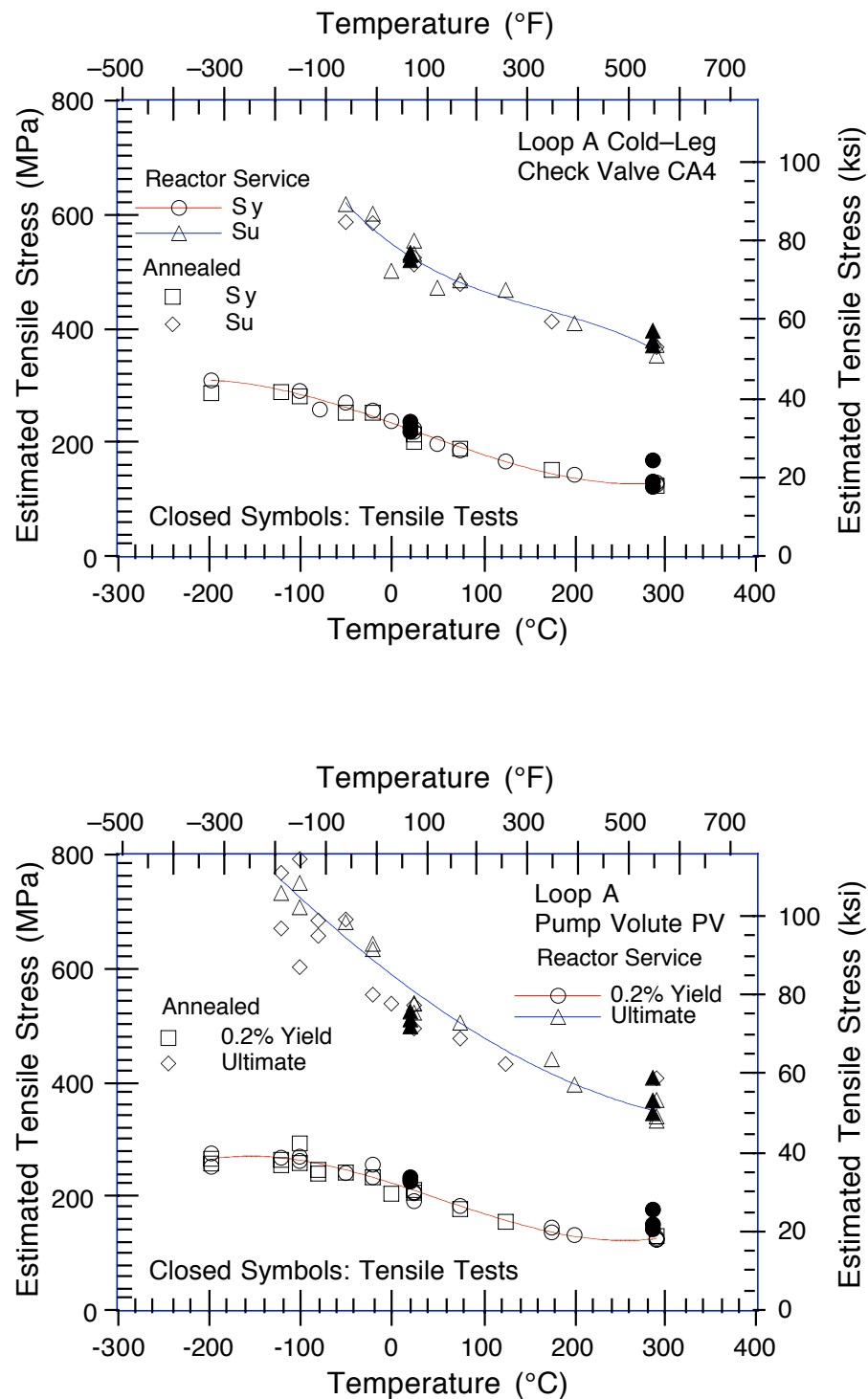
Figure 14. Yield and ultimate stresses estimated from Charpy-impact data and obtained from tensile tests for cold-leg check valve and pump volute, and estimated tensile stresses of annealed materials
