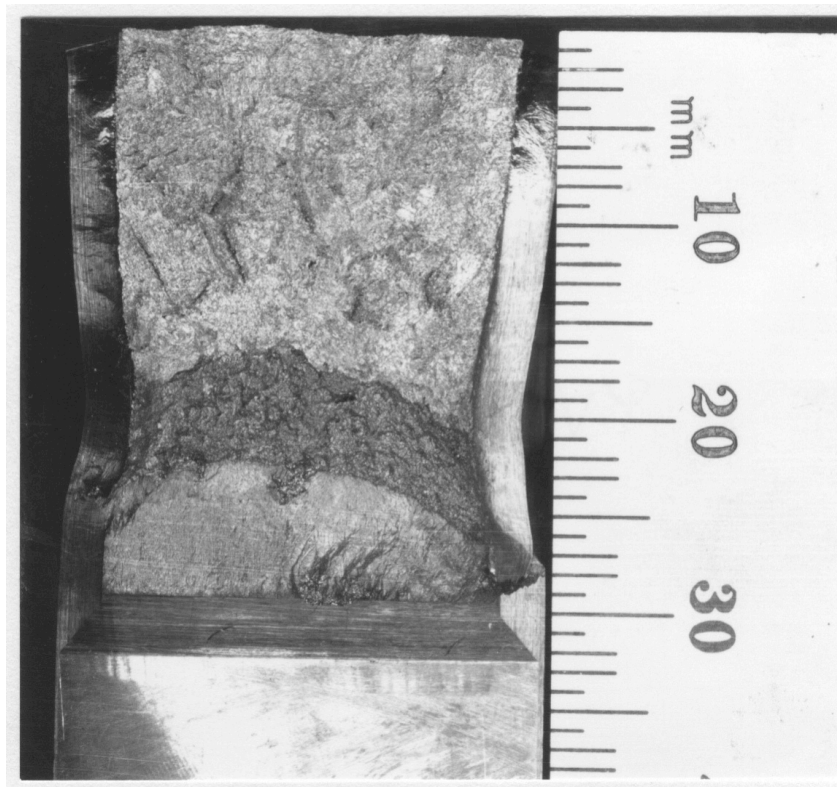
Figure C-44. Fracture surface of pump volute PV tested at 290°C after 13 y of service at 264°C
