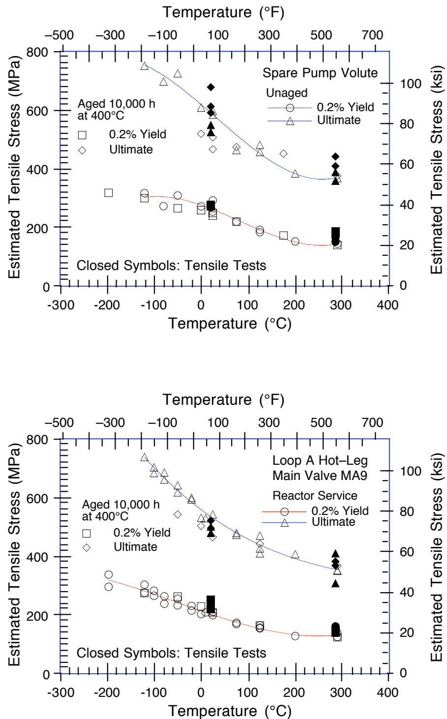
Figure 16. Yield and ultimate stresses estimated from Charpy-impact data and obtained from tensile tests for spare pump volute and hot-leg main valve before and after aging for 10,000 h at 400°C
