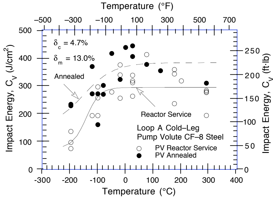
Figure 12. Charpy transition curves for Loop A pump volute after 13 y of service at 264°C. (Solid and dashed lines represent best-fit curves for service-aged and annealed materials, respectively.)
