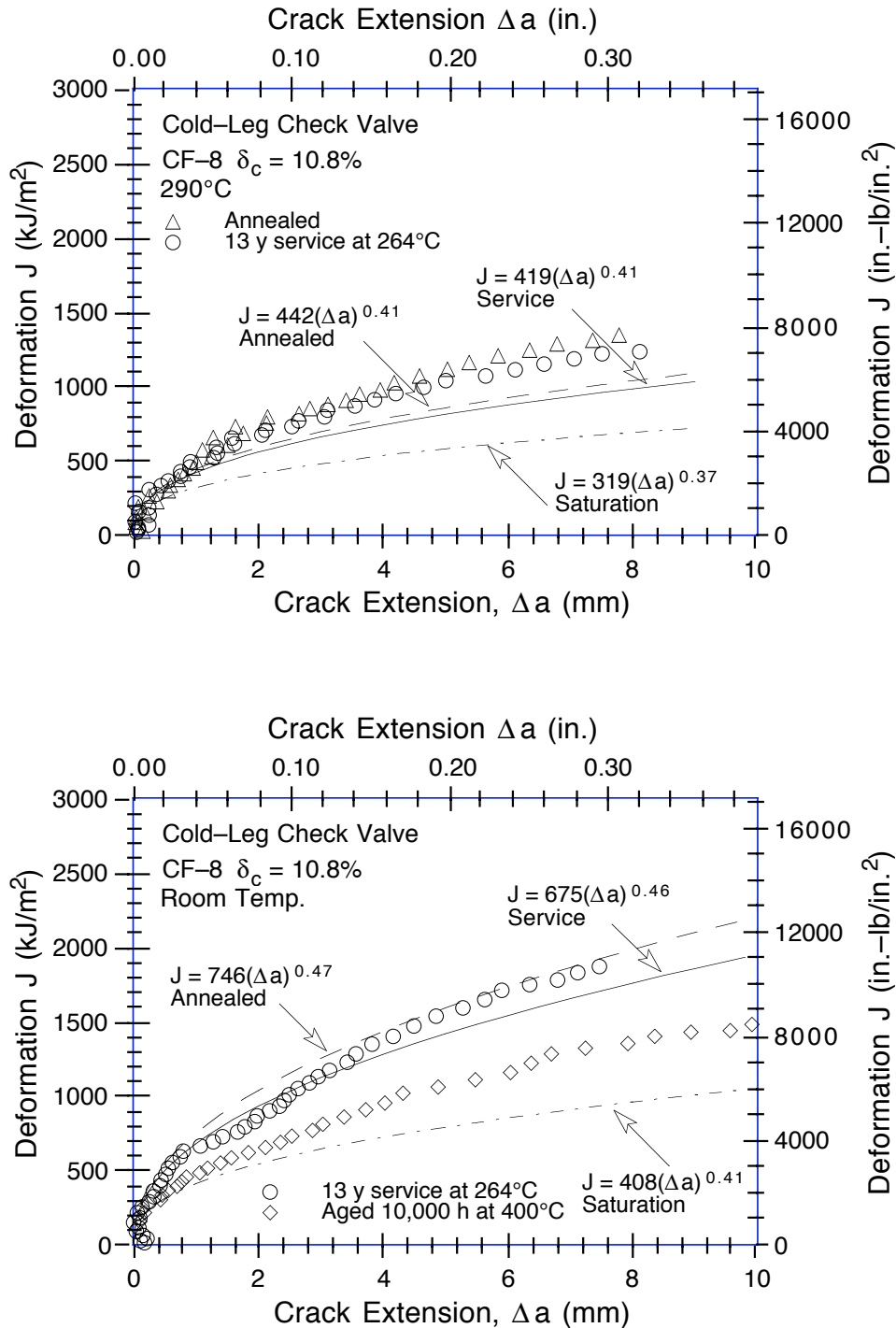
Figure 25. Estimated and measured fracture toughness J - R curves for the cold-leg check valve in the annealed, 13-y service at 264°C, and fully embrittled or saturation condition. (Dashed, solid, and chain-dot lines are the best-fit power-law J - R curves for annealed, service-aged, and laboratory-aged materials, respectively.)
