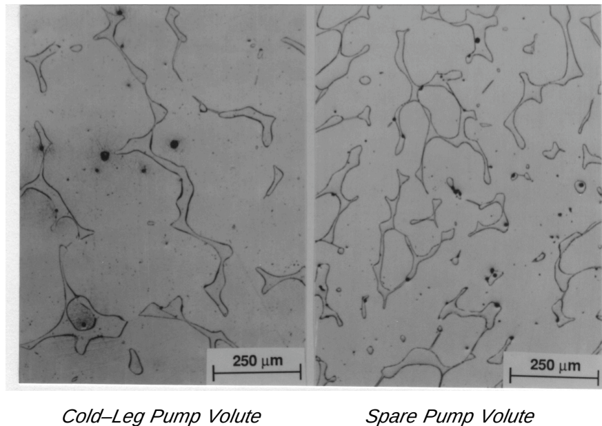
Figure 7. Ferrite morphology of cast materials from the cold-leg and spare pump volutes from the Shippingport reactor
