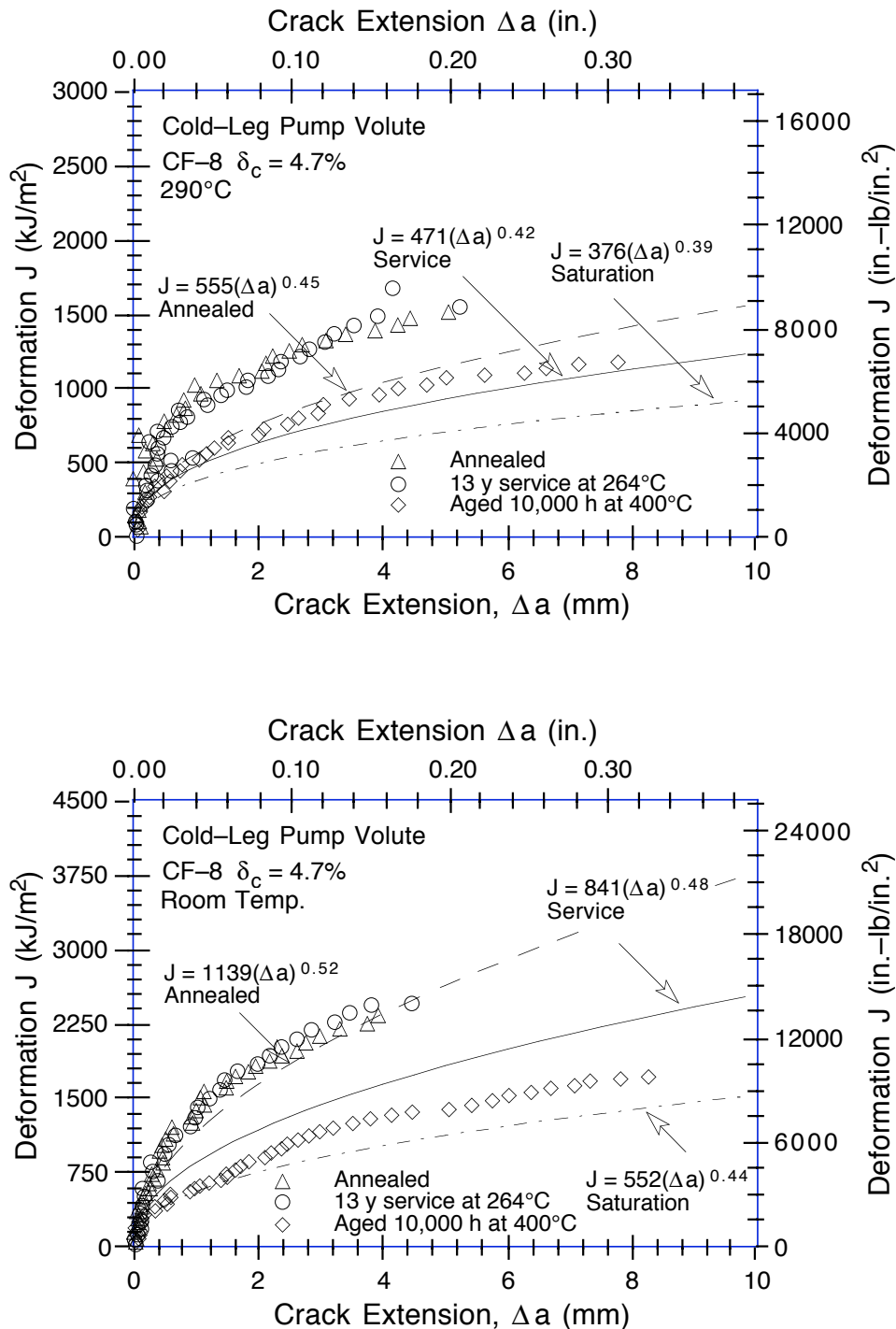
Figure 27. Estimated and measured fracture toughness J - R curves for the cold-leg pump volute in the annealed, 13-y service at 264°C, and fully embrittled or saturation condition. (Dashed, solid, and chain-dot lines are the best-fit power-law J - R curves for annealed, service-aged, and laboratory-aged materials, respectively.)
