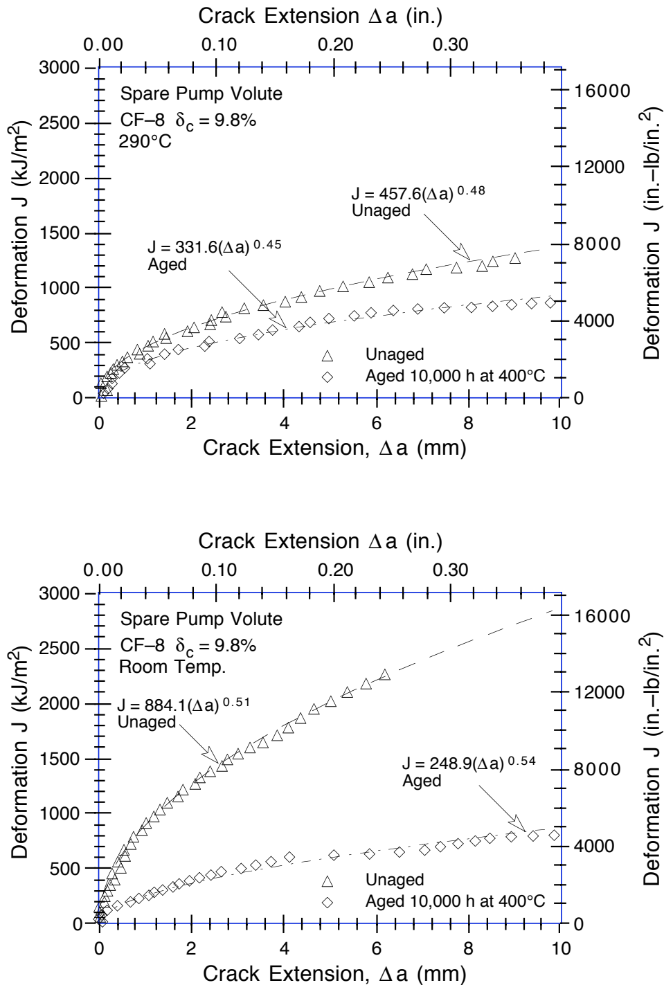
Figure 20. Fracture toughness J - R curves at room temperature and 290°C for unaged and laboratory-aged material from the spare pump volute. (Dashed and chain-dot lines are the best-fit power-law J - R curves for the unaged and laboratory-aged materials, respectively.)
