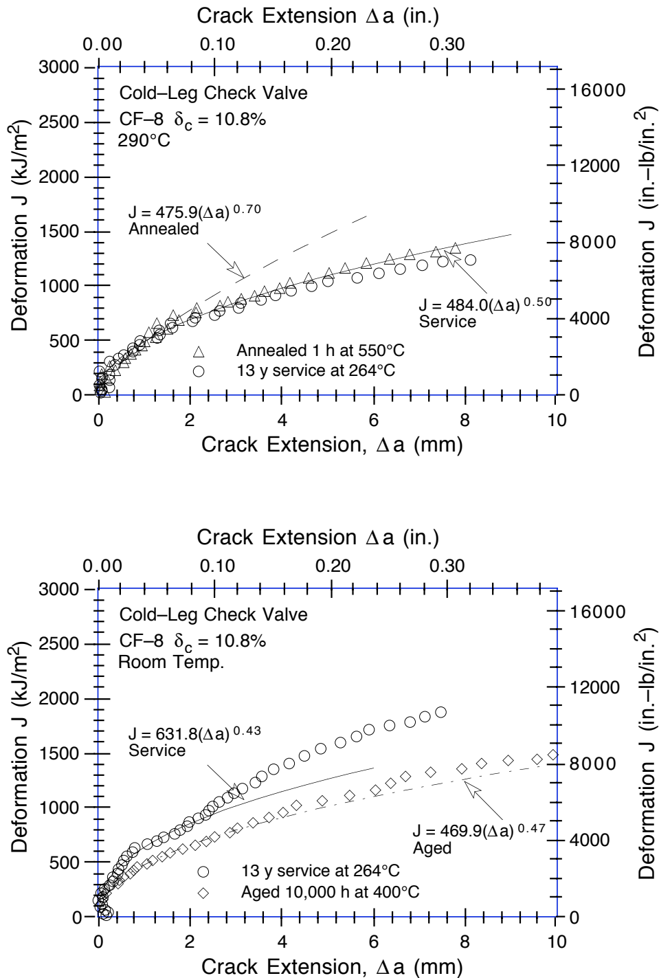
Figure 17. Fracture toughness J - R curves at room temperature and 290°C for annealed, service-aged, and laboratory-aged material from the cold-leg check valve. (Dashed, solid, and chain-dot lines are the best-fit power-law J - R curves for the annealed, service-aged, and laboratory-aged materials, respectively.)
