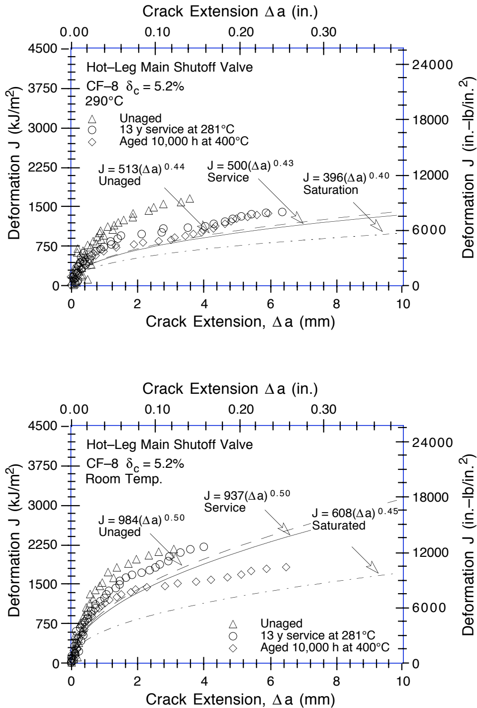
Figure 26. Estimated and measured fracture toughness J - R curves for the hot-leg main shutoff valve in essentially unaged, 13-y service at 281°C, and fully embrittled or saturation condition. (Dashed, solid, and chain-dot lines are the best-fit power-law J - R curves for unaged, service-aged, and laboratory-aged materials, respectively.)
