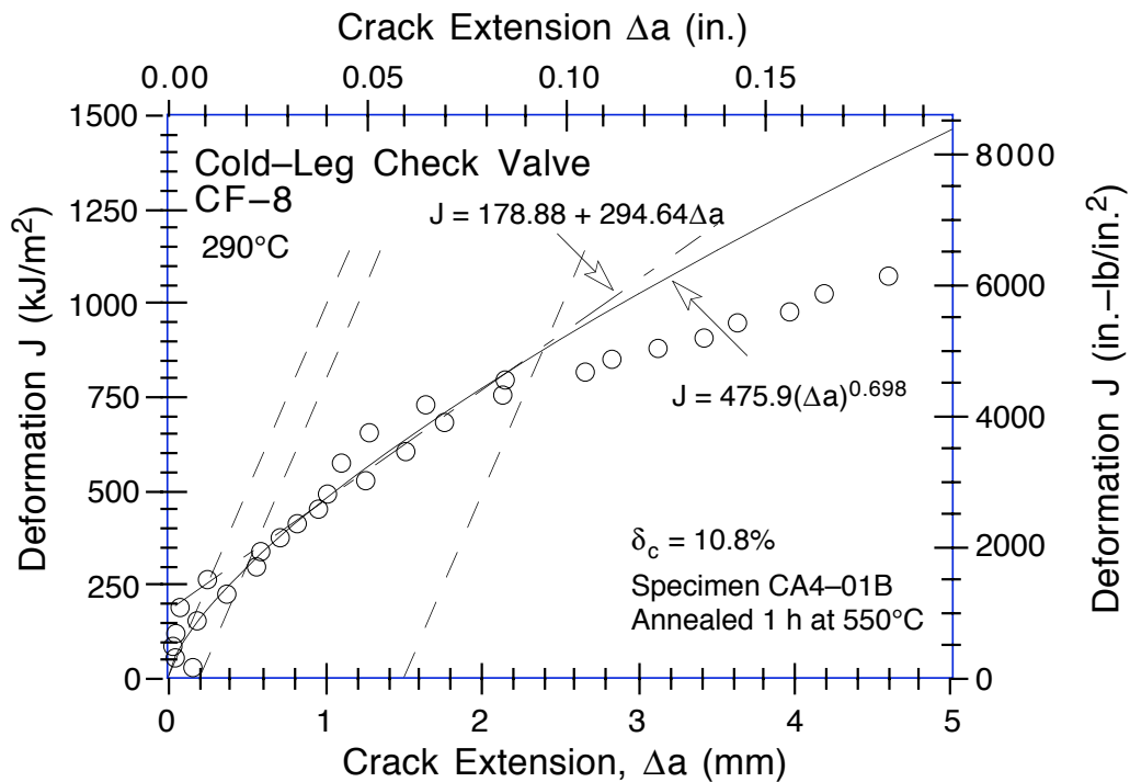
Figure C-9. Deformation J - R Curve at 290^{\circ}\text{C} for material from the cold-leg check valve CA4 annealed for 1 h at 550^{\circ}\text{C} and water quenched
