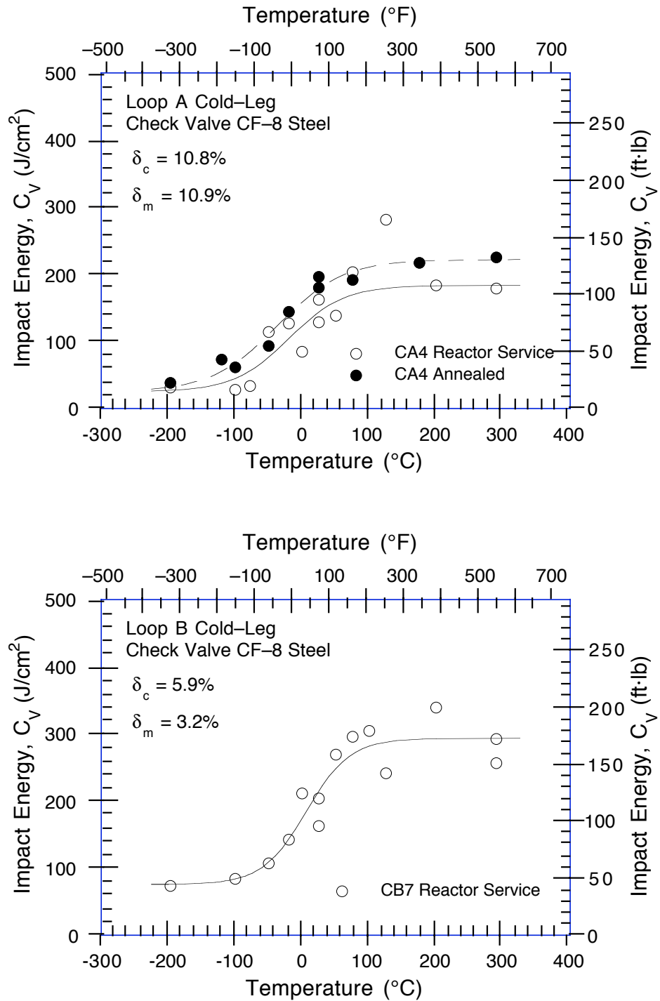
Figure 10. Charpy transition curves for Loop A and B cold-leg check valves after 13 y of service at 264°C. (Solid and dashed lines represent best-fit curves for service-aged and annealed materials, respectively.)
