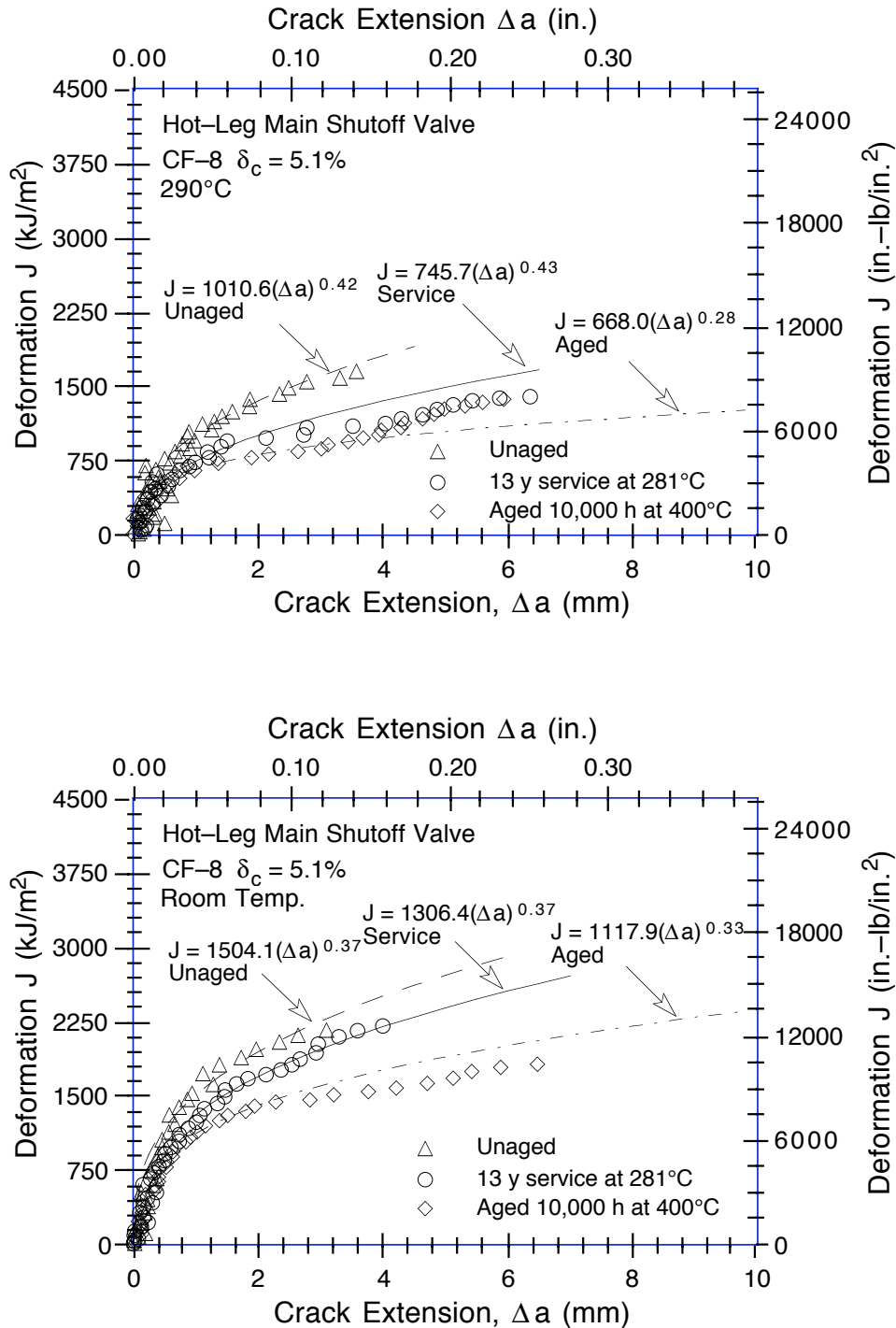
Figure 18. Fracture toughness J - R curves at room temperature and 290°C for unaged, service-aged, and laboratory-aged material from the hot-leg main shutoff valve. (Dashed, solid, and chain-dot lines are the best-fit power-law J - R curves for the unaged, service-aged, and laboratory-aged materials, respectively.)
