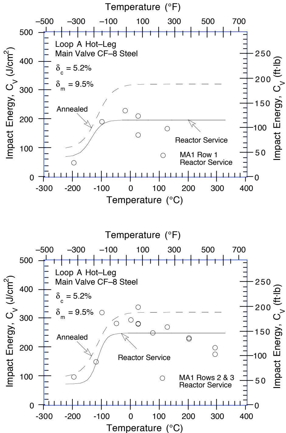
Figure 11. Charpy transition curves for Loop A hot-leg main shutoff valve after 13 y of service at 281°C. Row 1 corresponds to inner 15-mm region and rows 2 and 3 represent 15- to 50-mm region of the valve body. (Solid and dashed lines are best-fit curves.)
