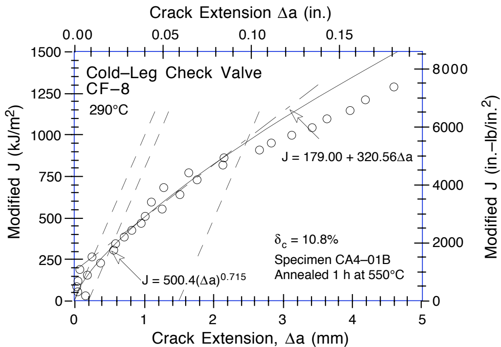
Figure C-10. Modified J - R Curve at 290^{\circ}\text{C} for material from the cold-leg check valve CA4 annealed for 1 h at 550^{\circ}\text{C} and water quenched
