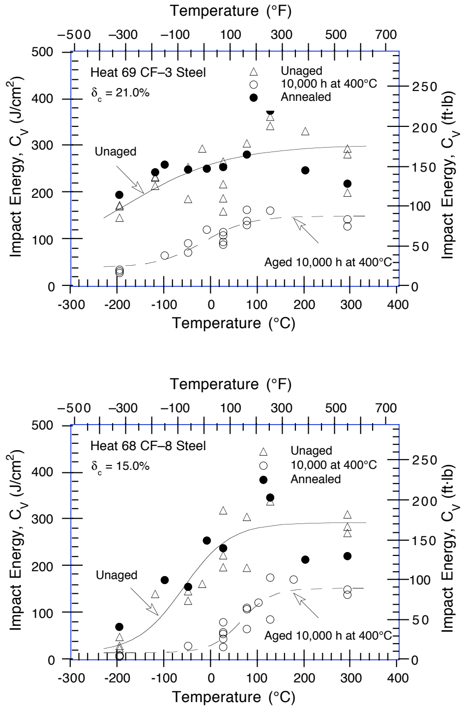
Figure 8. Effect of annealing for 1 h at 550°C and then water quenching on Charpy-transition curves for laboratory-aged Heats 69, 68, and 75, and service-aged KRB pump cover plate. The dashed lines and open circles represent the transition curve before the annealing treatment. (Solid and dashed lines are best-fit curves.)
