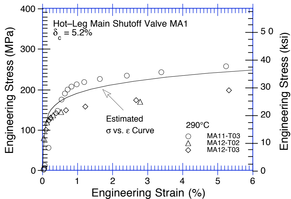
Figure 30. Estimated and measured tensile stress-vs.-strain curves at room temperature and 290°C for the hot-leg main shutoff valve after service for \approx 13 y at 281°C
