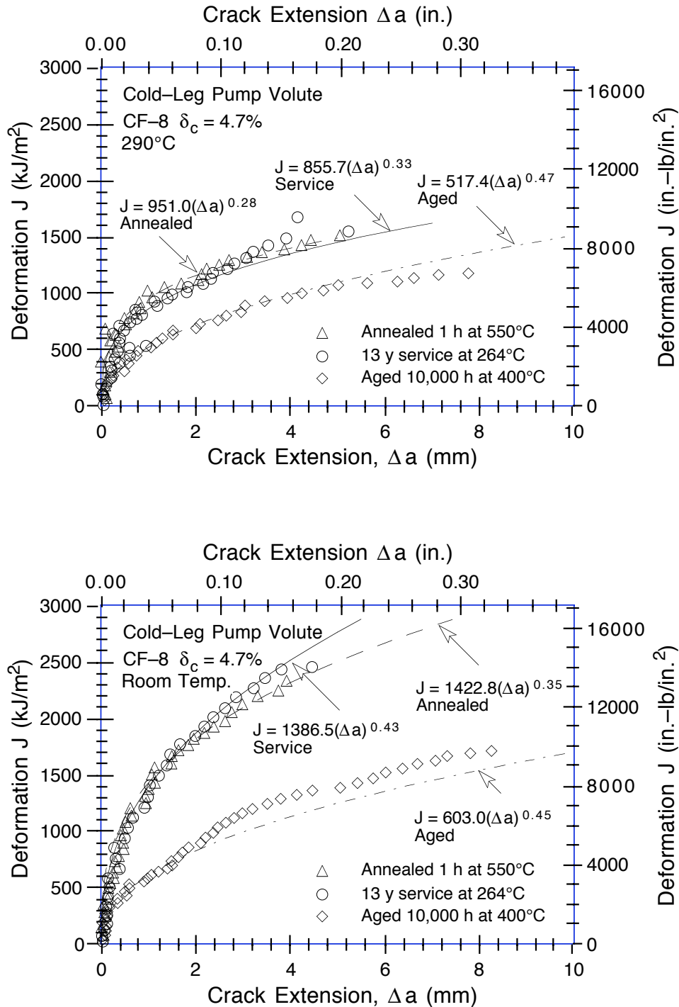
Figure 19. Fracture toughness J - R curves at room temperature and 290°C for annealed, service-aged, and laboratory-aged material from the cold-leg pump volute. (Dashed, solid, and chain-dot lines are the best-fit power-law J - R curves for the annealed, service-aged, and laboratory-aged materials, respectively.)
