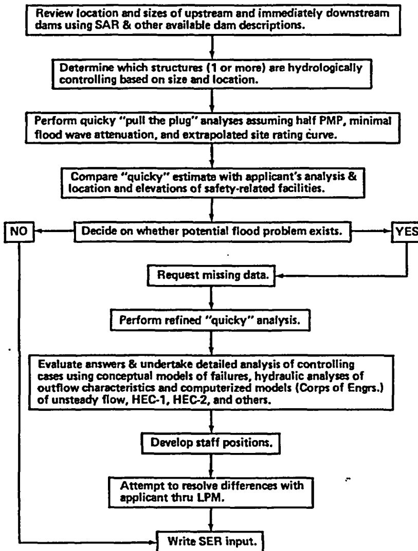
Figure 2.4.4-1 Standard Review Plan Section 2.4.4 Seismically - Induced Floods
