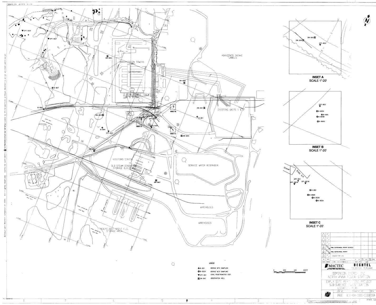
Figure 2.5-4B-1 Sub-Surface Investigation Location Plan
