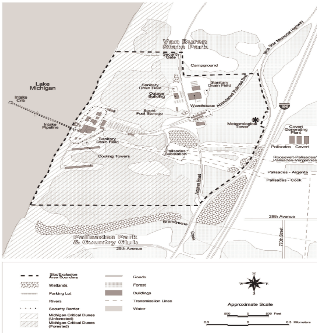
FIGURE 2.1-3 SITE MAP
