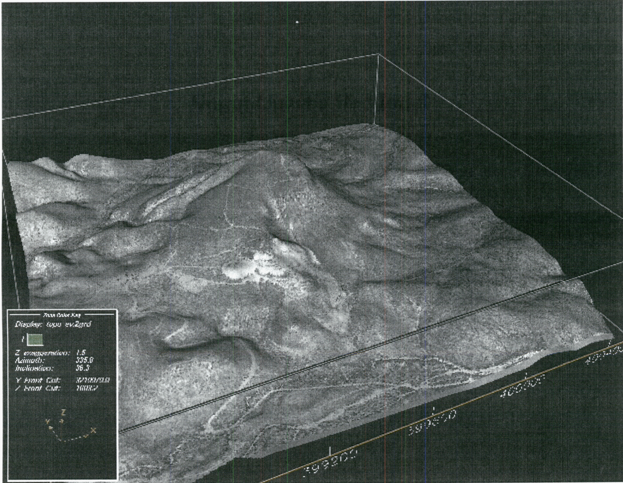
Drape of Air Photo on EarthVision 3D Surface SW-NE View Across Cuesta and Mine
