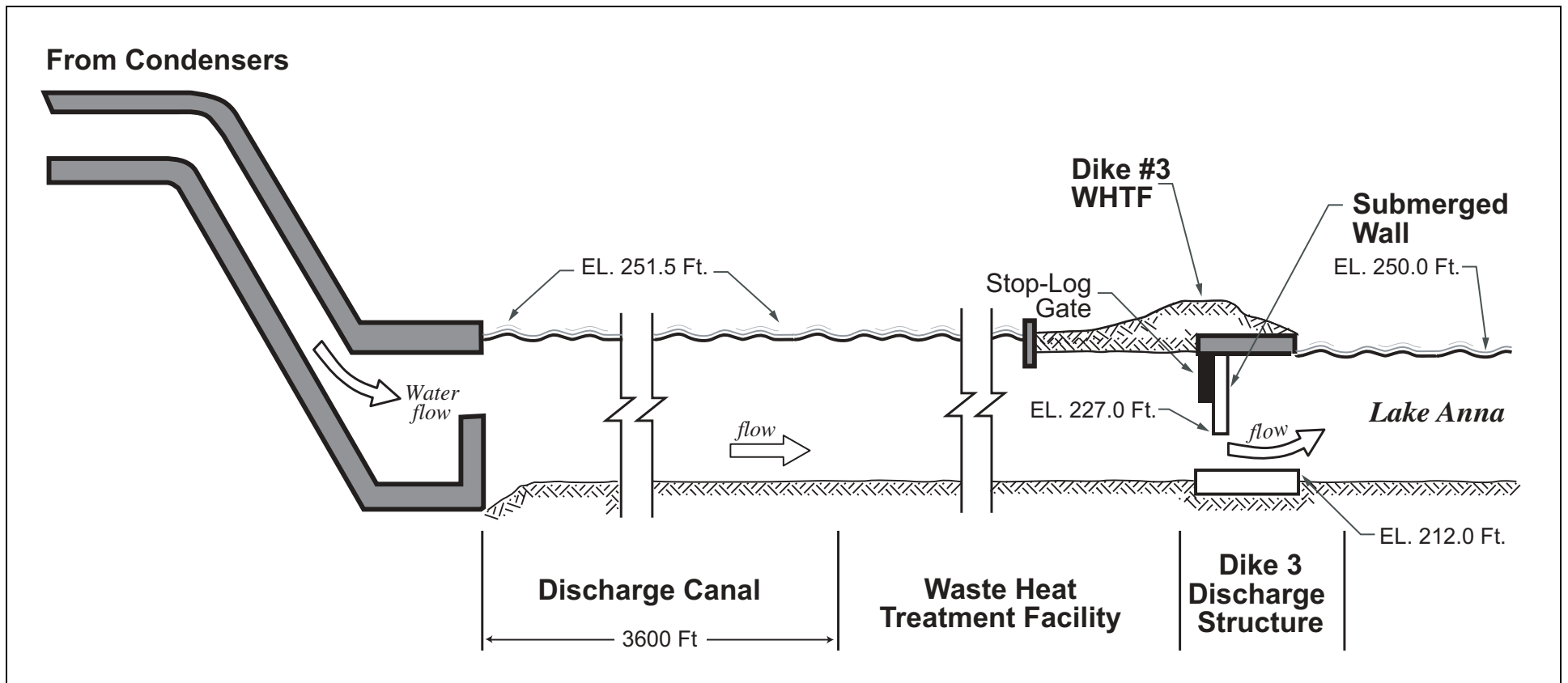
Figure 2.4-3 Schematic Cross-Sectional Diagram of Water-Discharge System at Dike 3 WHTF
