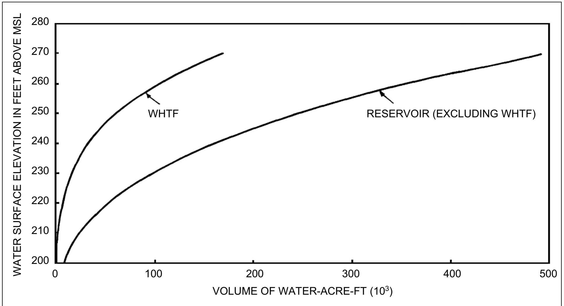
Figure 2.3-2 Elevation-Area Curves for North Anna Reservoir and Waste Heat Treatment Facility
