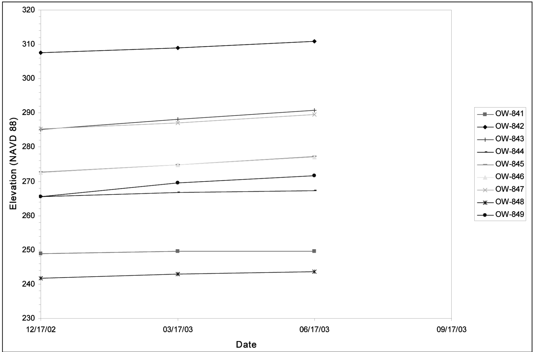
Figure 2.3-7 Ground Water Level Hydrographs
