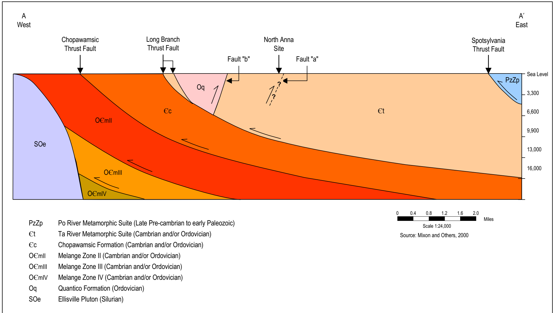
Figure 2.6-5 Site Area Geologic Cross Section (5-Mile Radius)
