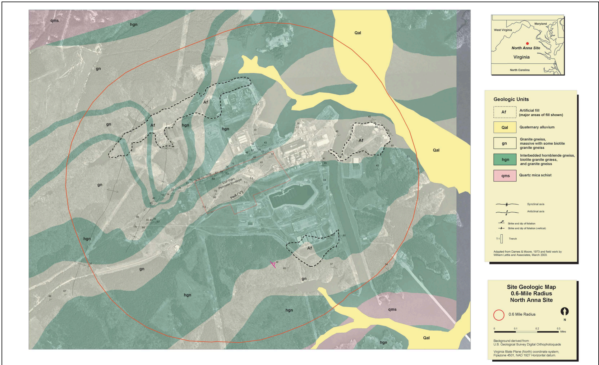
Figure 2.5-18 Site Geologic Map (0.6-Mile Radius)
