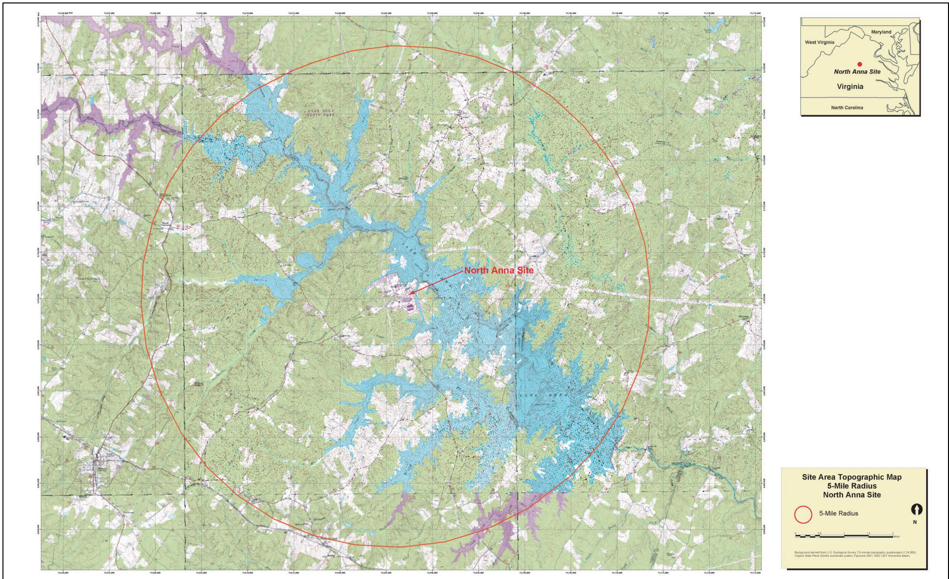
Figure 2.5-15 Site Area Topographic Map (5-Mile Radius)
