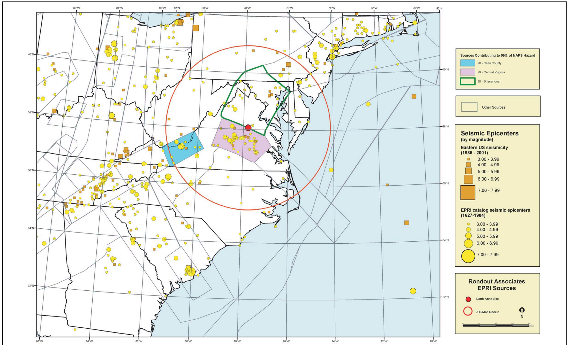
Figure 2.5-22 Rondout Associates EPRI Sources
