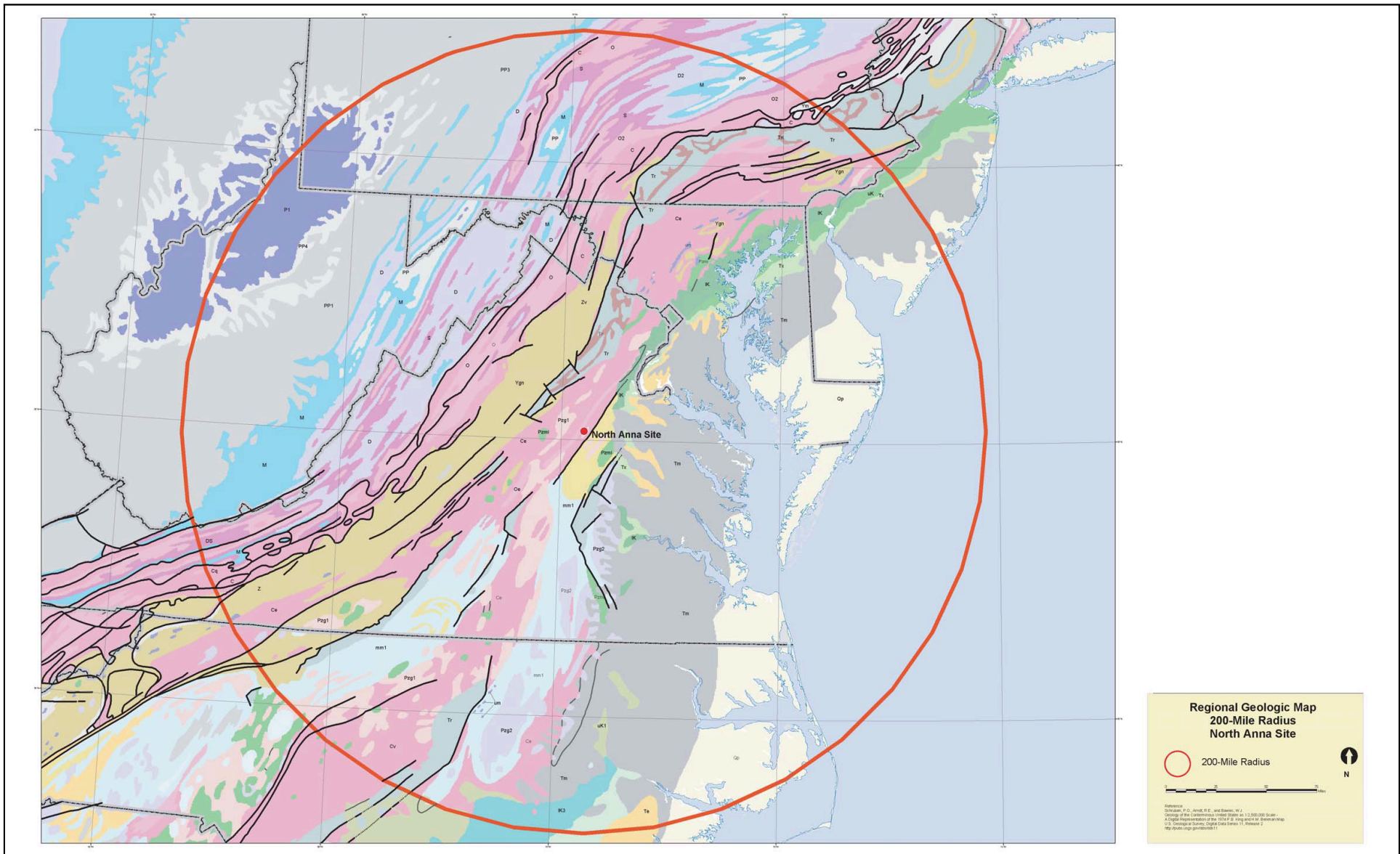
Figure 2.5-3 Regional Geologic Map (200-Mile Radius) (Sheet 1 of 2)
