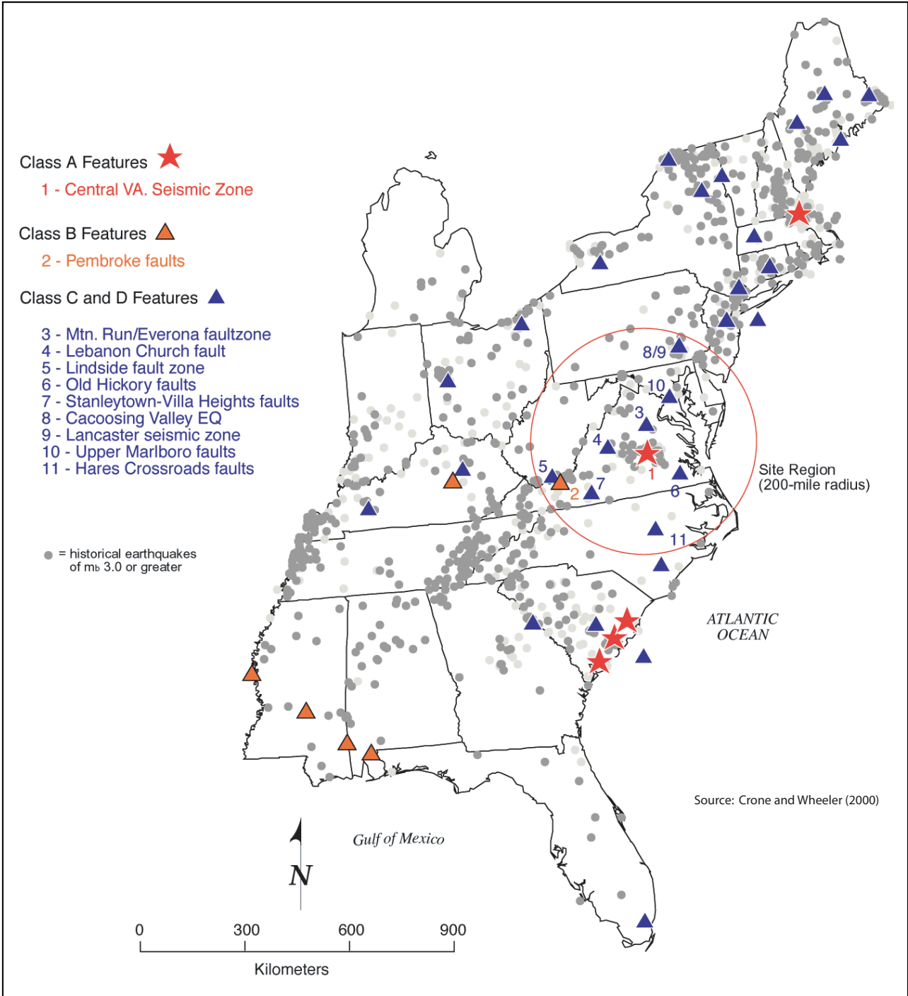
Figure 2.5-12 Quaternary Features Map
