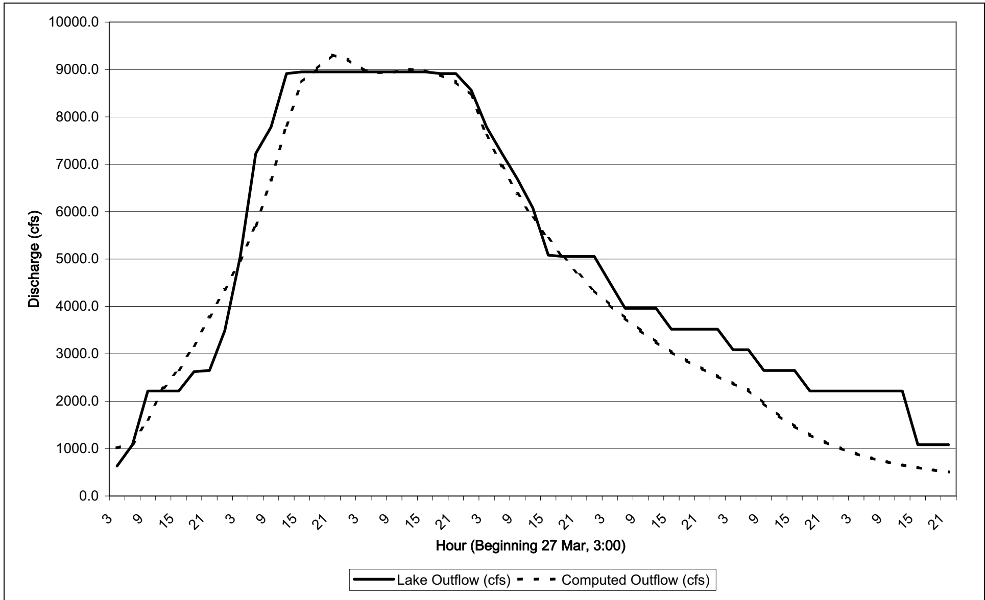
Figure 2.4-8 1994 Storm Outflow Hydrograph Comparison
