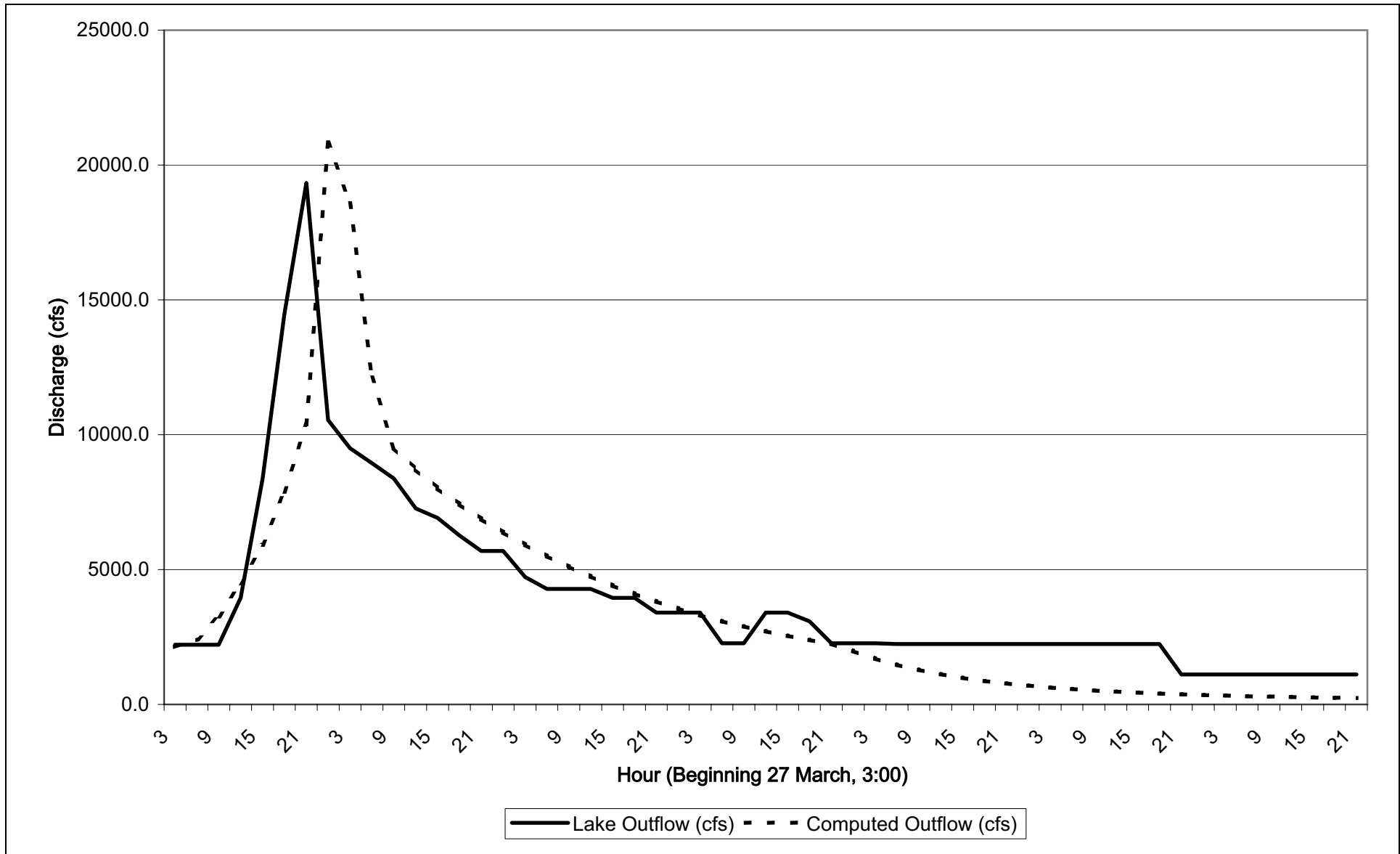
Figure 2.4-9 1995 Storm Outflow Hydrograph Comparison
