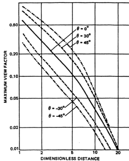
Figure 4-6. Radiation Shape Factor as a Function of Separation Distance and Tilt Angle for Fires with a Height-to-Radius Ratio of 6
