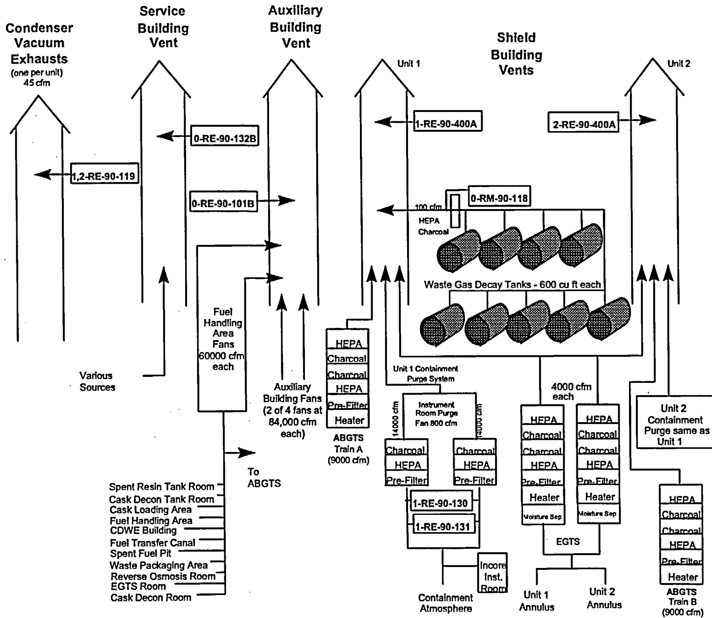
Figure 7.2 - DETAIL OF GASEOUS RELEASE/DISCHARGE POINTS
