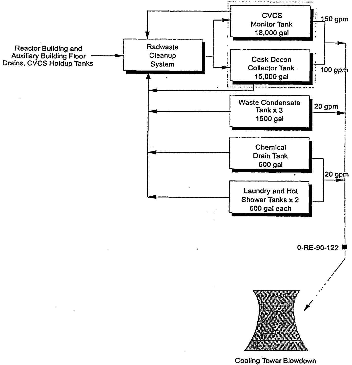
Figure 6.2 - LIQUID RADWASTE SYSTEM
