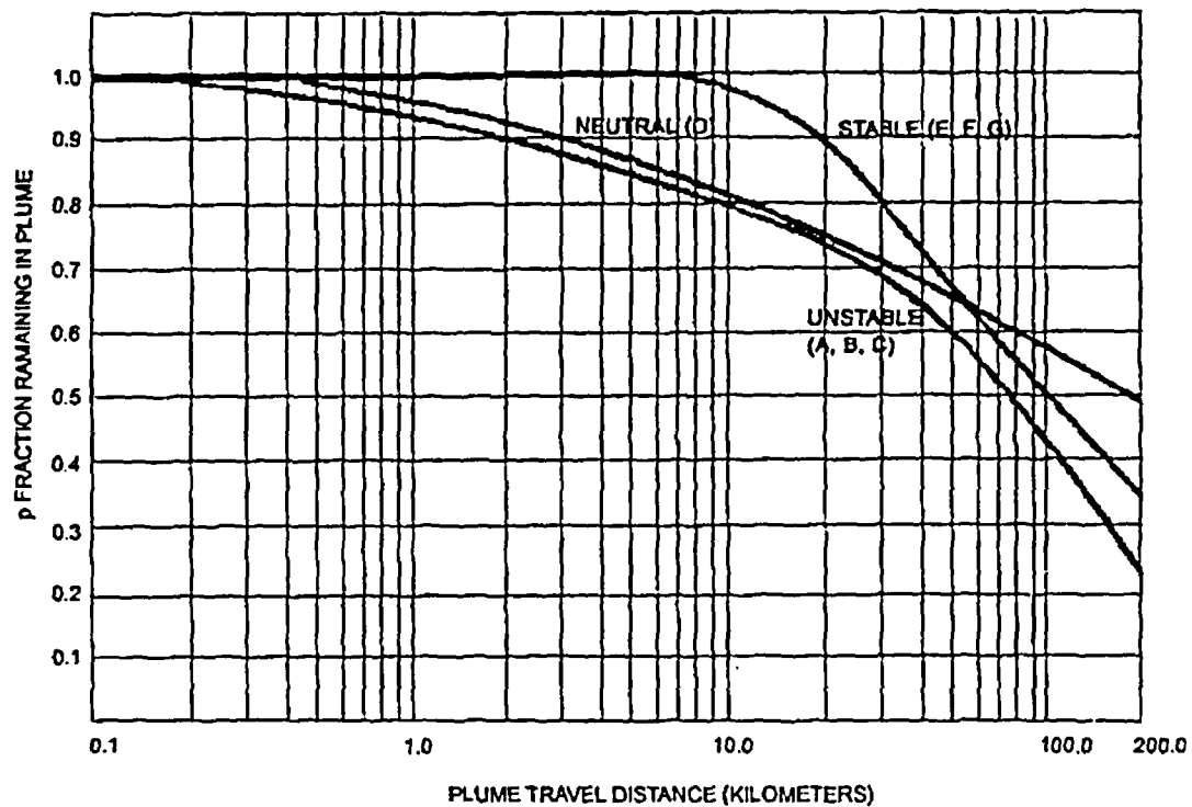
Figure 7.3 PLUME DEPLETION EFFECT (Page 2 of 4)
