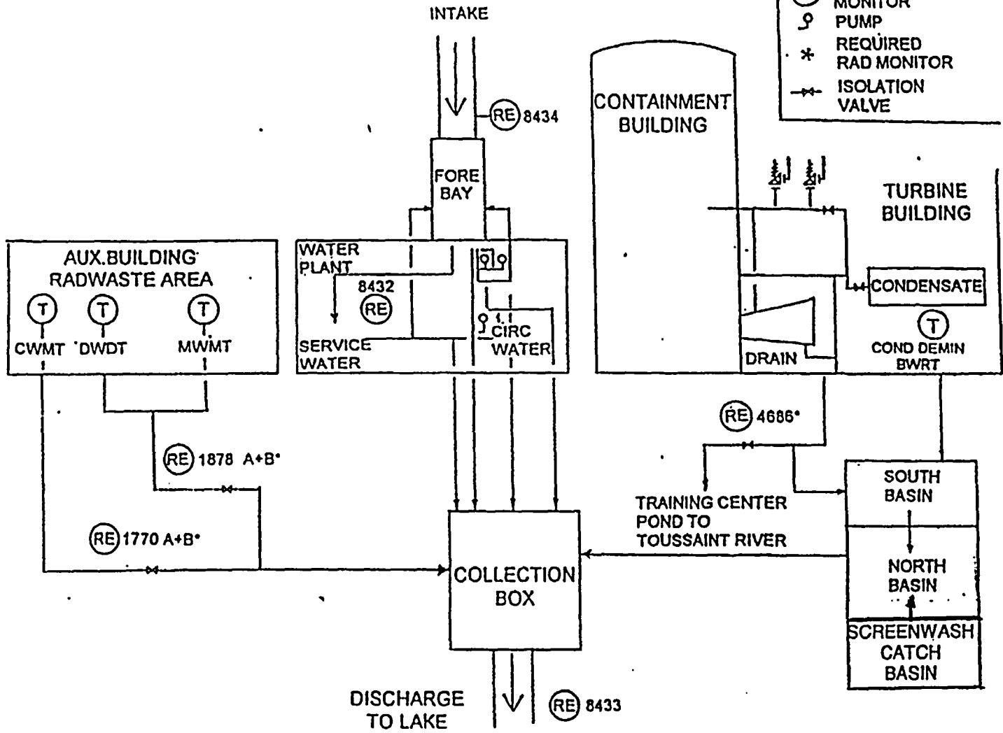
Liquid Radioactive Effluent Monitoring and Processing Diagram
