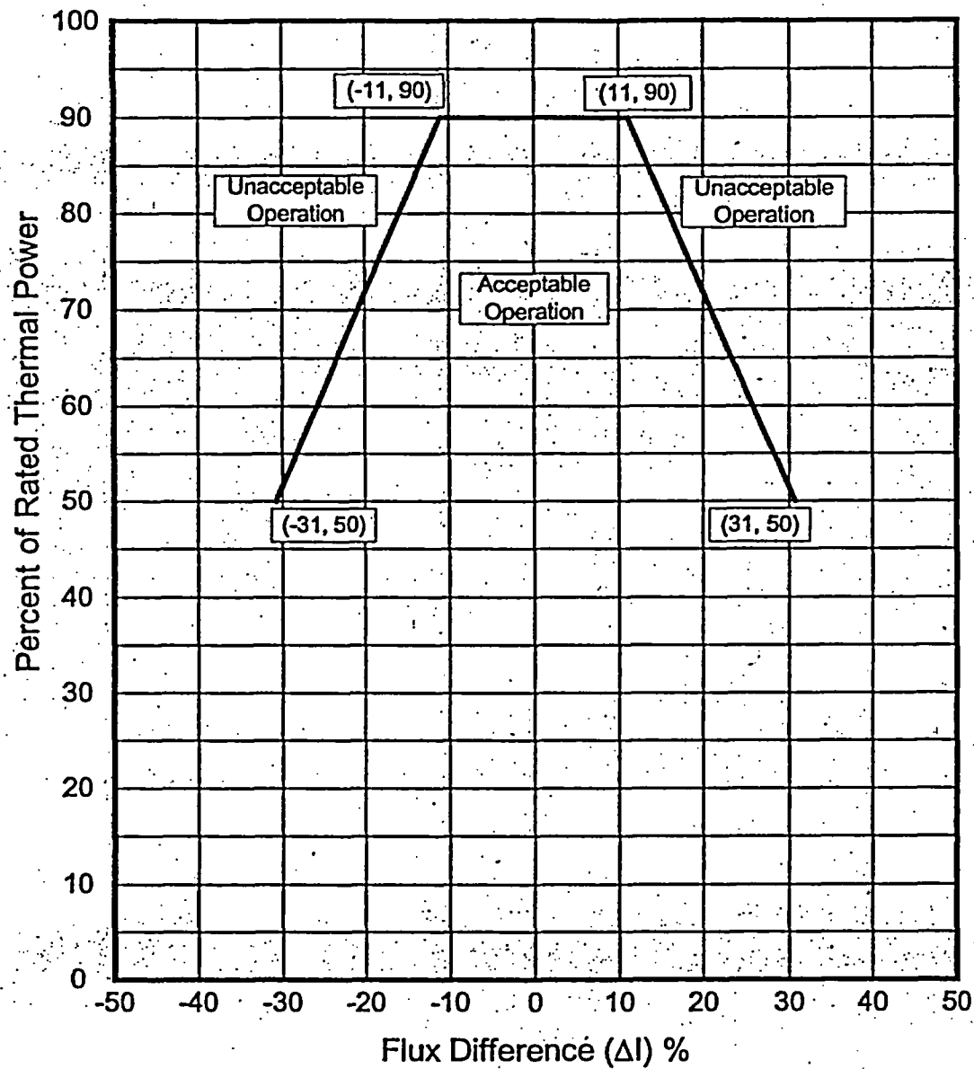
FIGURE 4.1-2 AXIAL FLUX DIFFERENCE LIMITS AS A FUNCTION OF RATED THERMAL POWER
