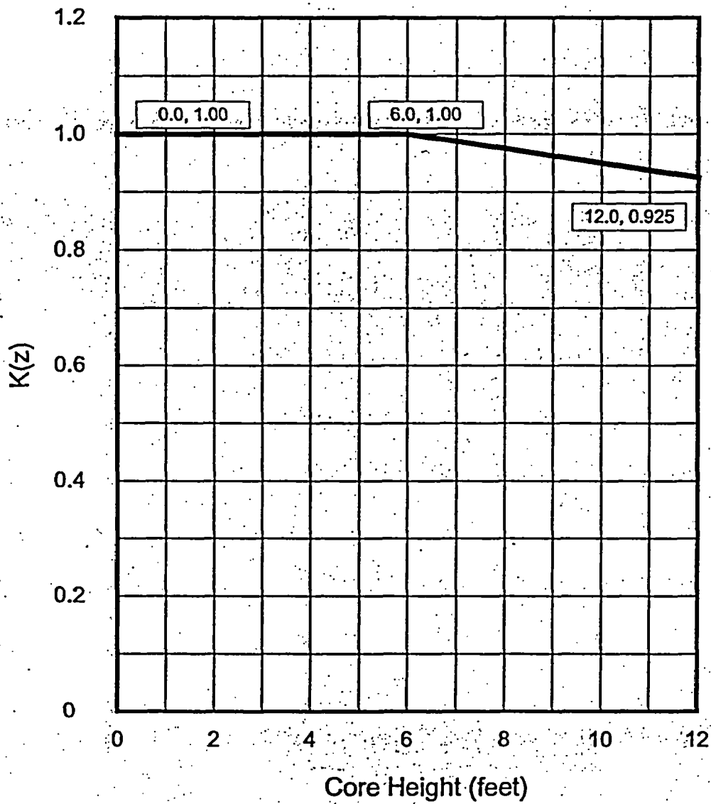
FIGURE 4.1-3 F 0 T NORMALIZED OPERATING ENVELOPE, K(Z)
