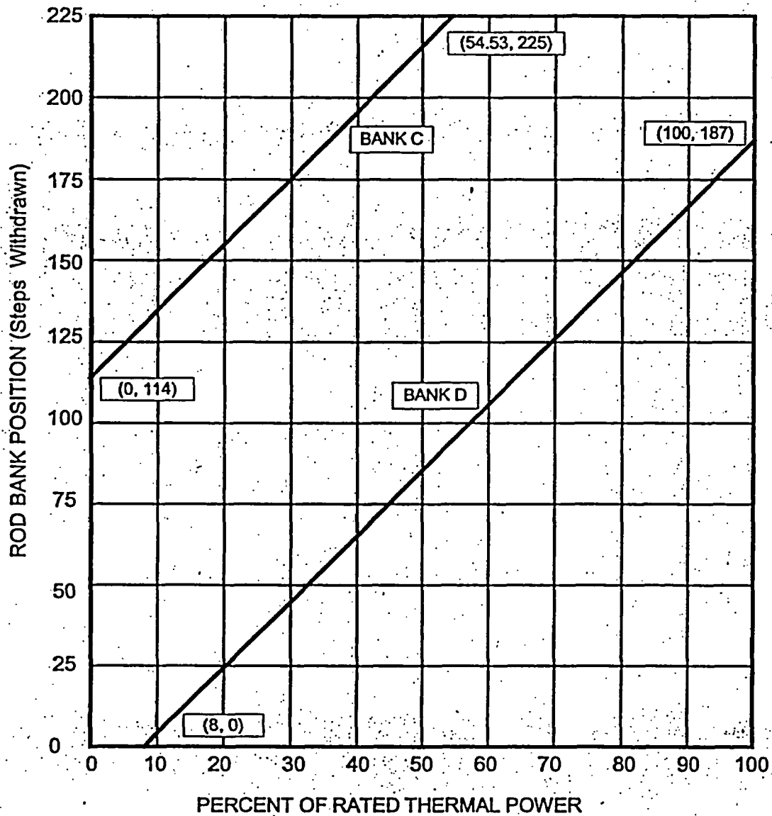
FIGURE 4.1-1 CONTROL ROD INSERTION LIMITS AS A FUNCTION OF RATED POWER LEVEL
