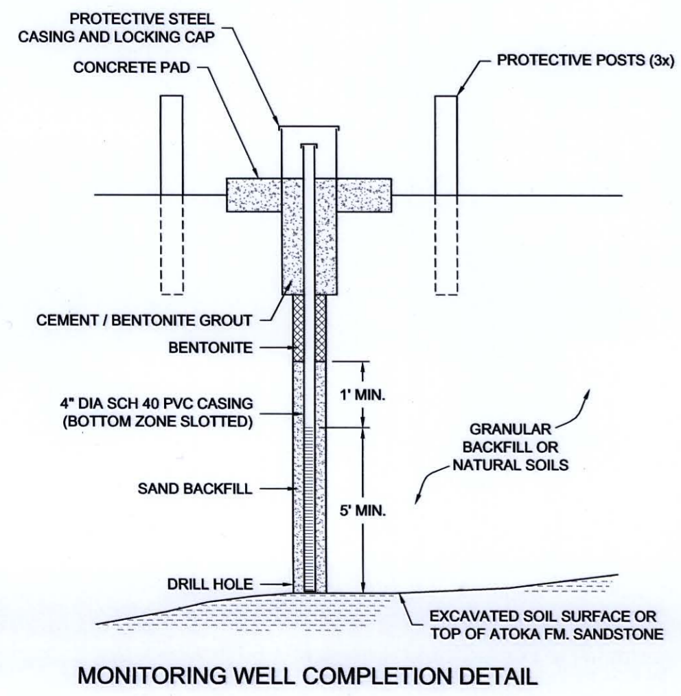
MONITORING WELL COMPLETION DETAIL
