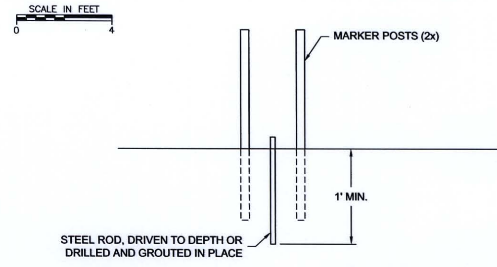
SETTLEMENT MONITORING POINT DETAIL
