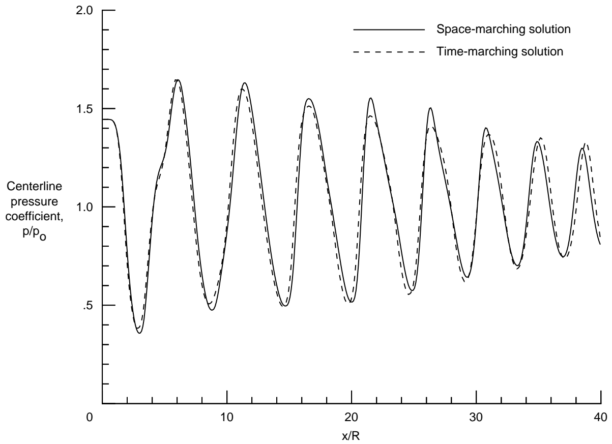
Figure 15. Space-marching and time-marching solutions for underexpanded Mach 2.0 supersonic jet computed with Jones-Lauder k-\epsilon turbulence model.
