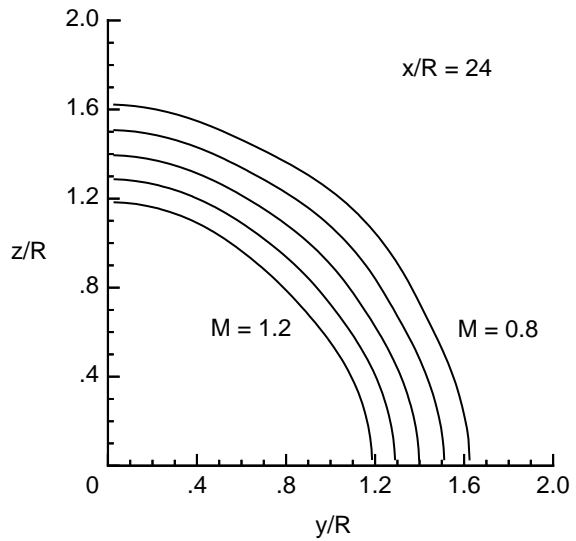
Figure 24. Cross-section shape evolution in streamwise direction of square underexpanded supersonic jet. Jet exit Mach number = 2.0; NPR = 11.12; p_e/p_o = 1.445 .
