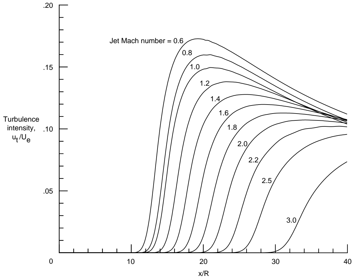
Figure 8. Centerline turbulence intensity profiles of axisymmetric jets at various subsonic and supersonic Mach numbers computed by using Jones-Launder two-equation k-\epsilon turbulence model with Wilcox compressibility correction.
