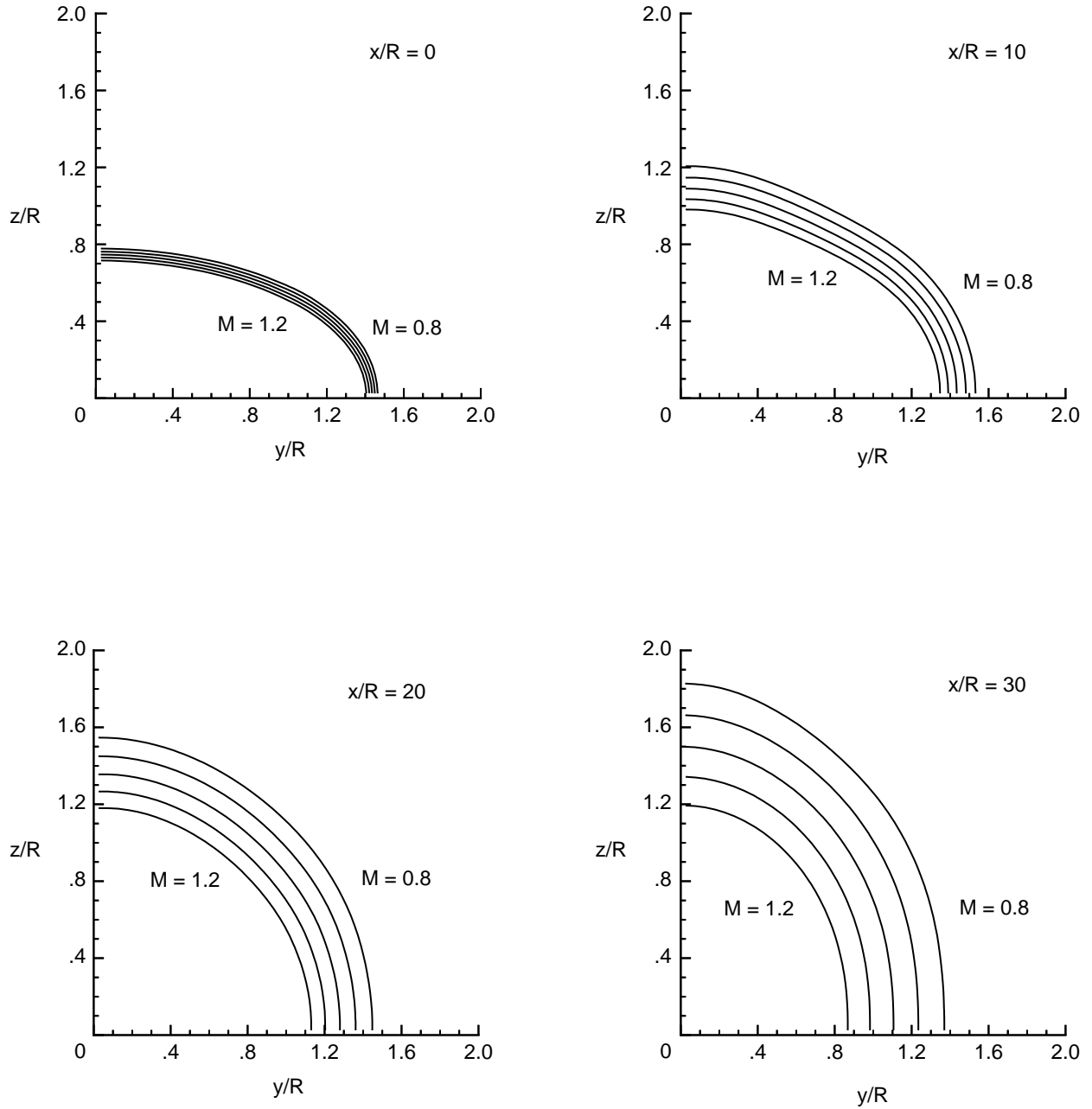
Figure 22. Cross-section shape evolution in streamwise direction of elliptic underexpanded supersonic jet. Shape aspect ratio = 2.0; Jet exit Mach number = 2.0; NPR = 11.12; p_e/p_o = 1.445 .
