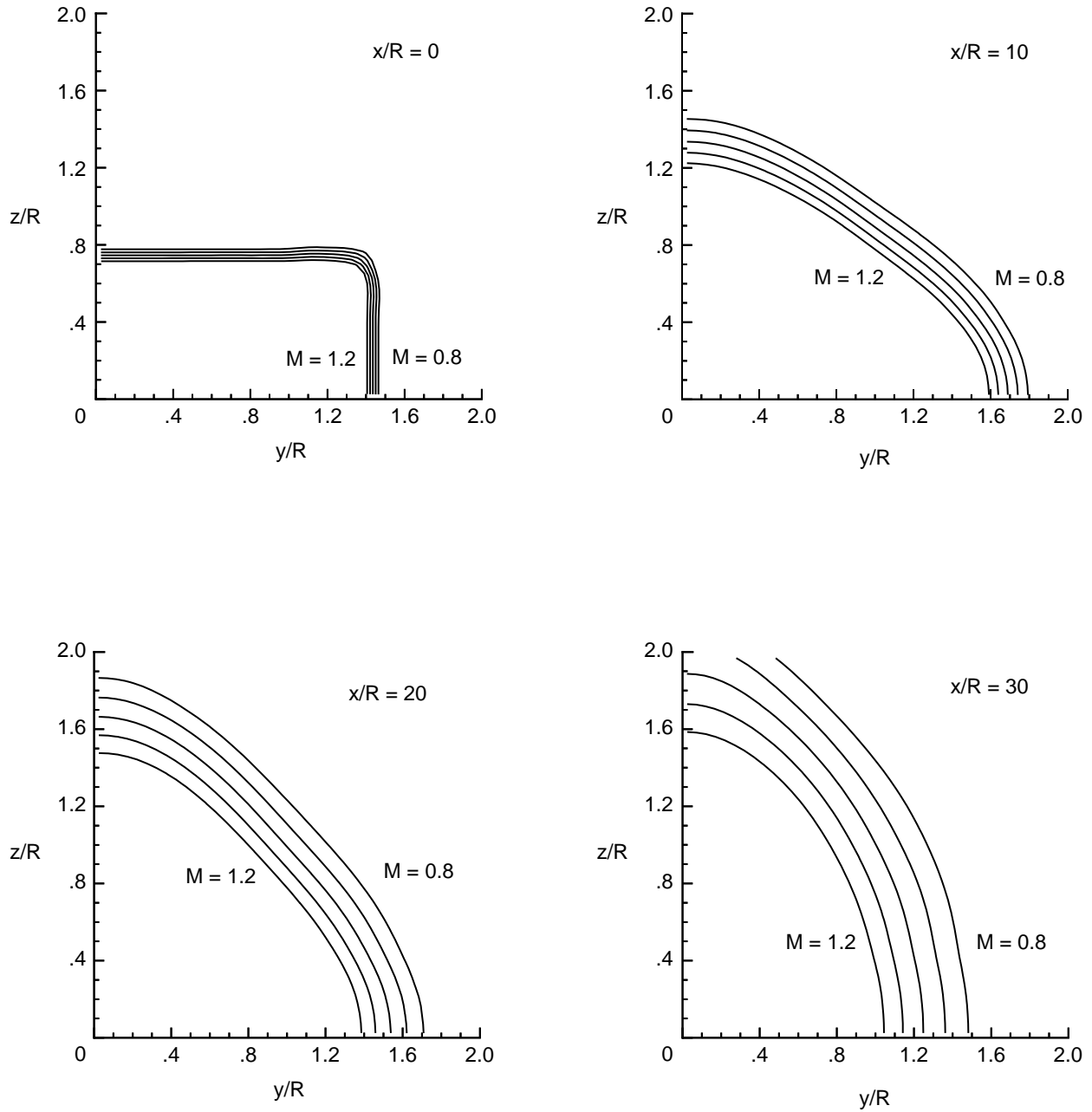
Figure 23. Cross-section shape evolution in streamwise direction of rectangular underexpanded supersonic jet. Shape aspect ratio = 2.0; Jet exit Mach number = 2.0; NPR = 11.12; p_e/p_o = 1.445 .
