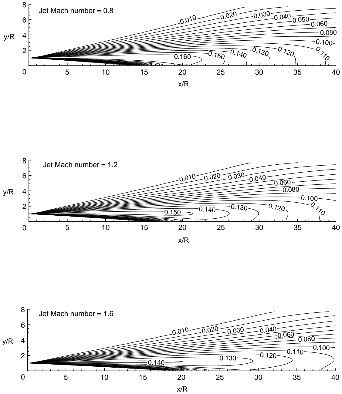
Figure 7. Typical turbulence intensity distribution in axisymmetric jets computed by using Jones-Launder k-\epsilon turbulence model with Wilcox model of compressibility correction for u_t/U_e contours.
