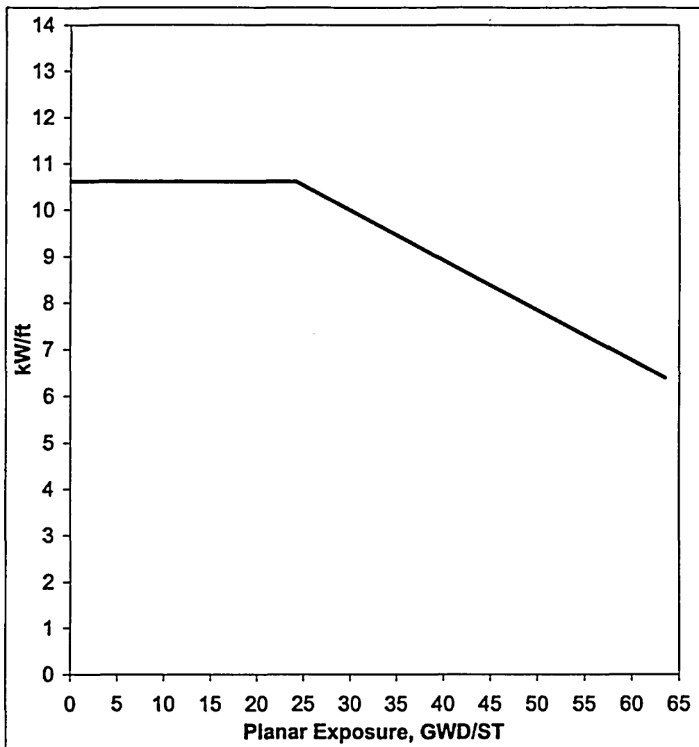
Exposure Dependent APLHGR Limit for GE12 Fuel
