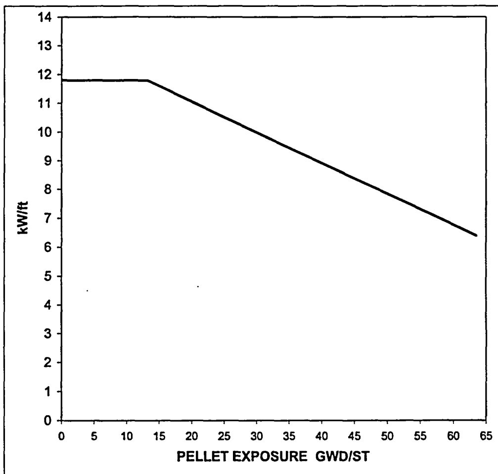
Exposure Dependent LHGR Limit for GE12 Fuel
