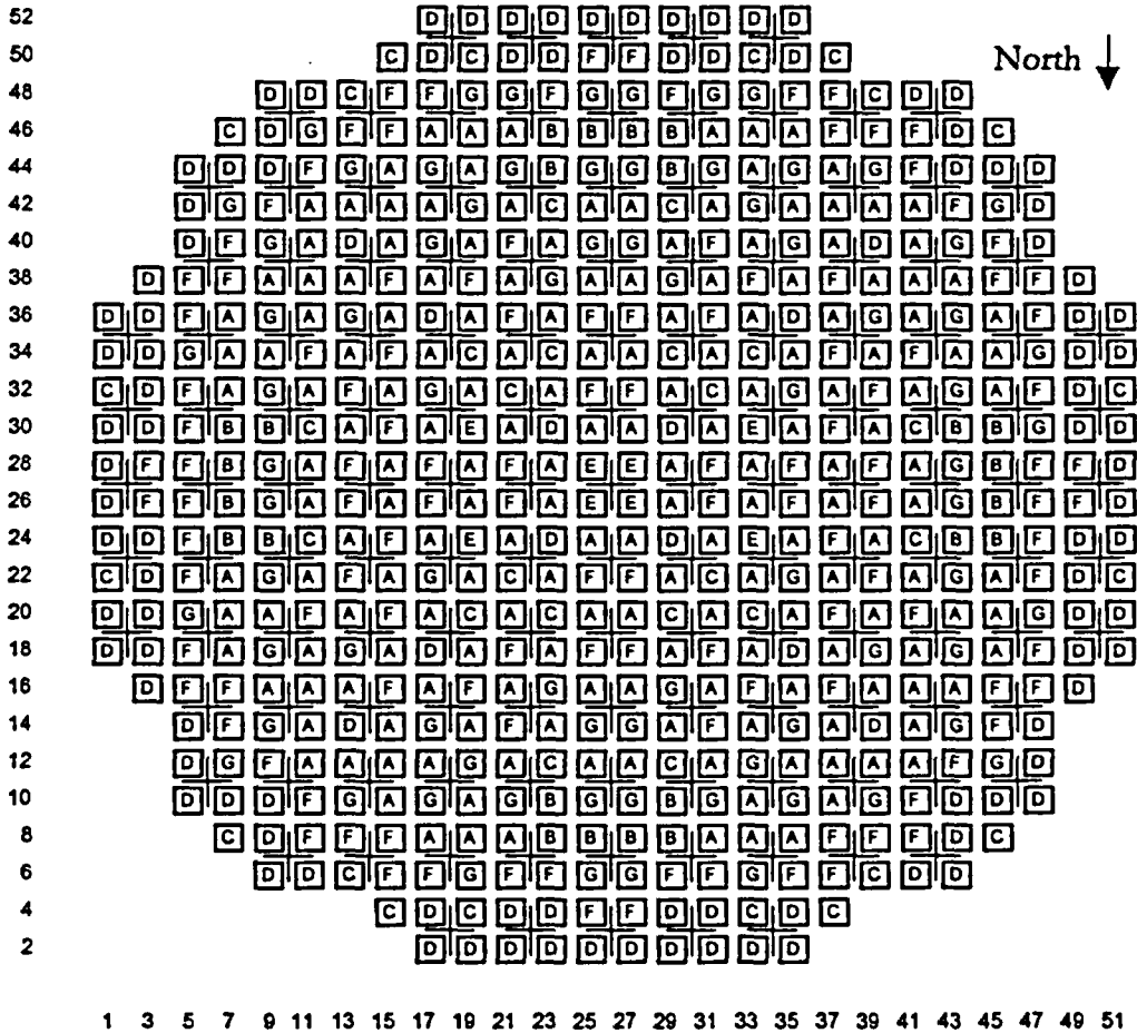
Cycle 17 Loading Pattern by Bundle Design
