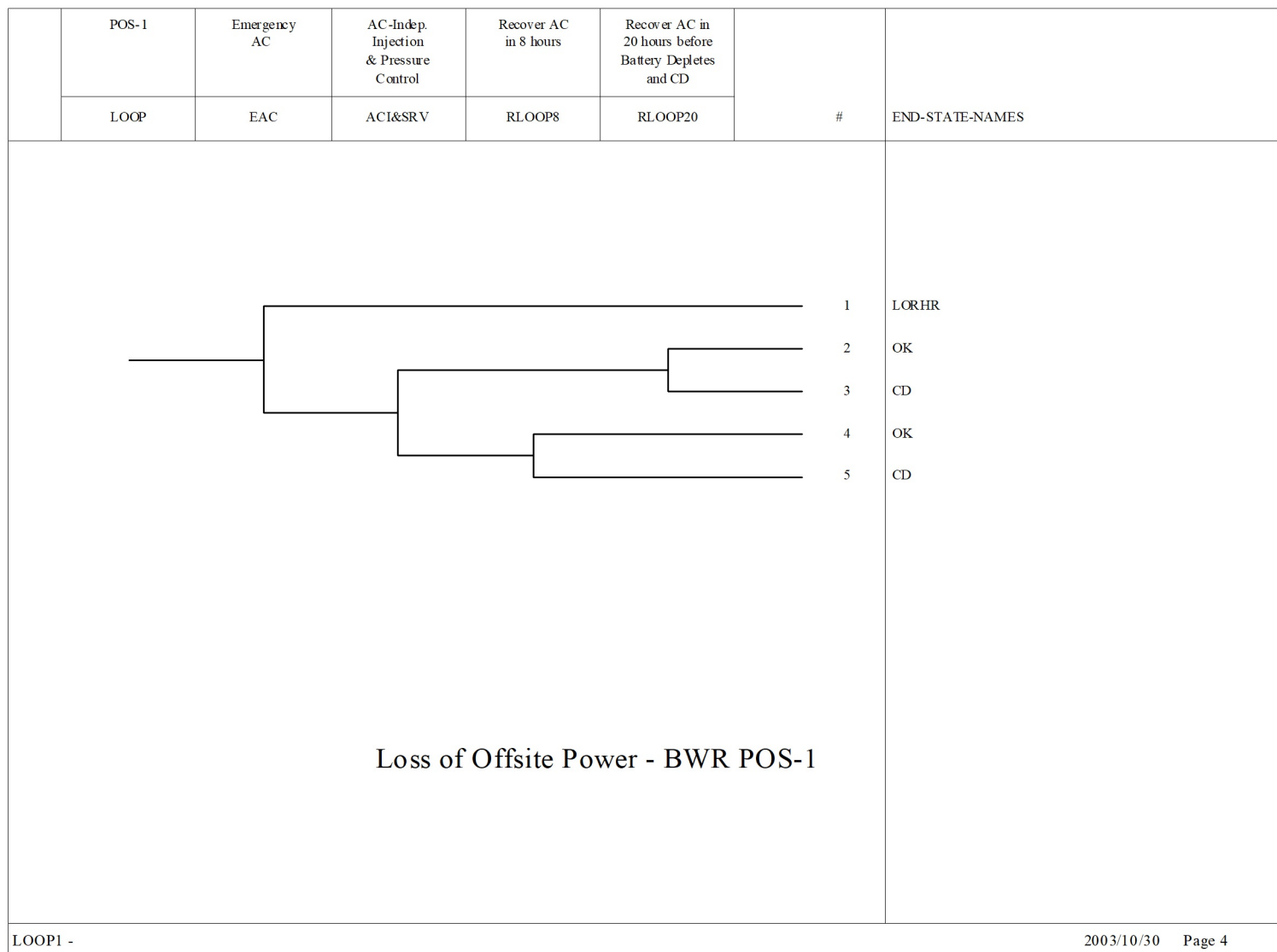
Figure 5 - Event Tree for Loss of Offsite Power - BWR POS-1
