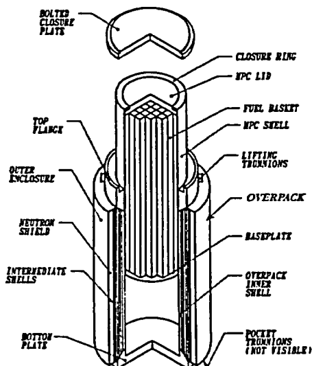
Figure 3. HOLTEC HI-STAR 100 Spent Fuel Transportation Cask
