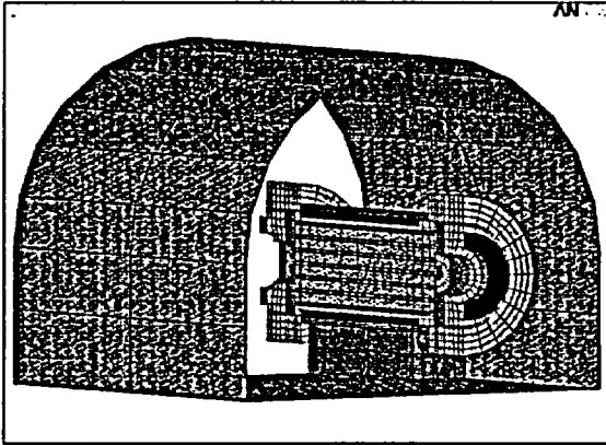
Figure 5. ANSYS HI-STAR 100 Cask Analysis Model Element Plot
