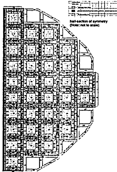
Figure 6. COBRA-SFS Model of TN-68 Basket and Support Rails
