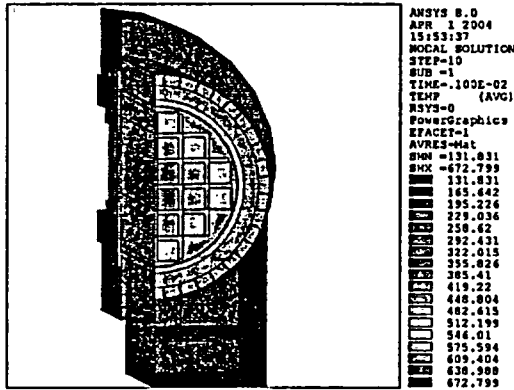
Figure 7. HI-STAR 100 Cask Normal Condition Temperature Distribution
