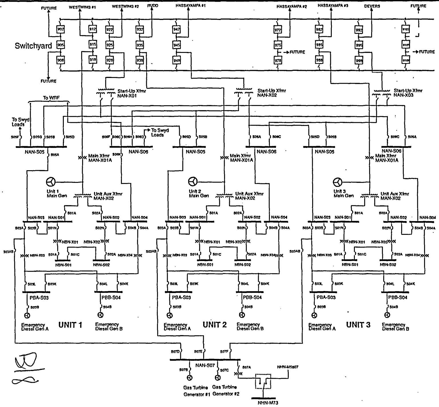
Appendix 51, Electric Plant Single Line Diagram
