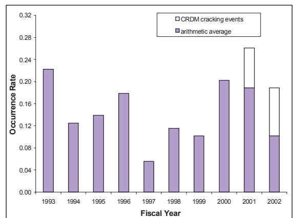
Figure 8: Precursors involving PWRs-occurrence rate, by fiscal year. No trend line is shown because no trend is detected that is statistically significant ( p -value = 0.37).
