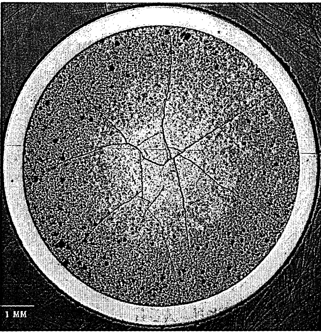
Micrograph of Irradiated MOX Pellet (RG)
