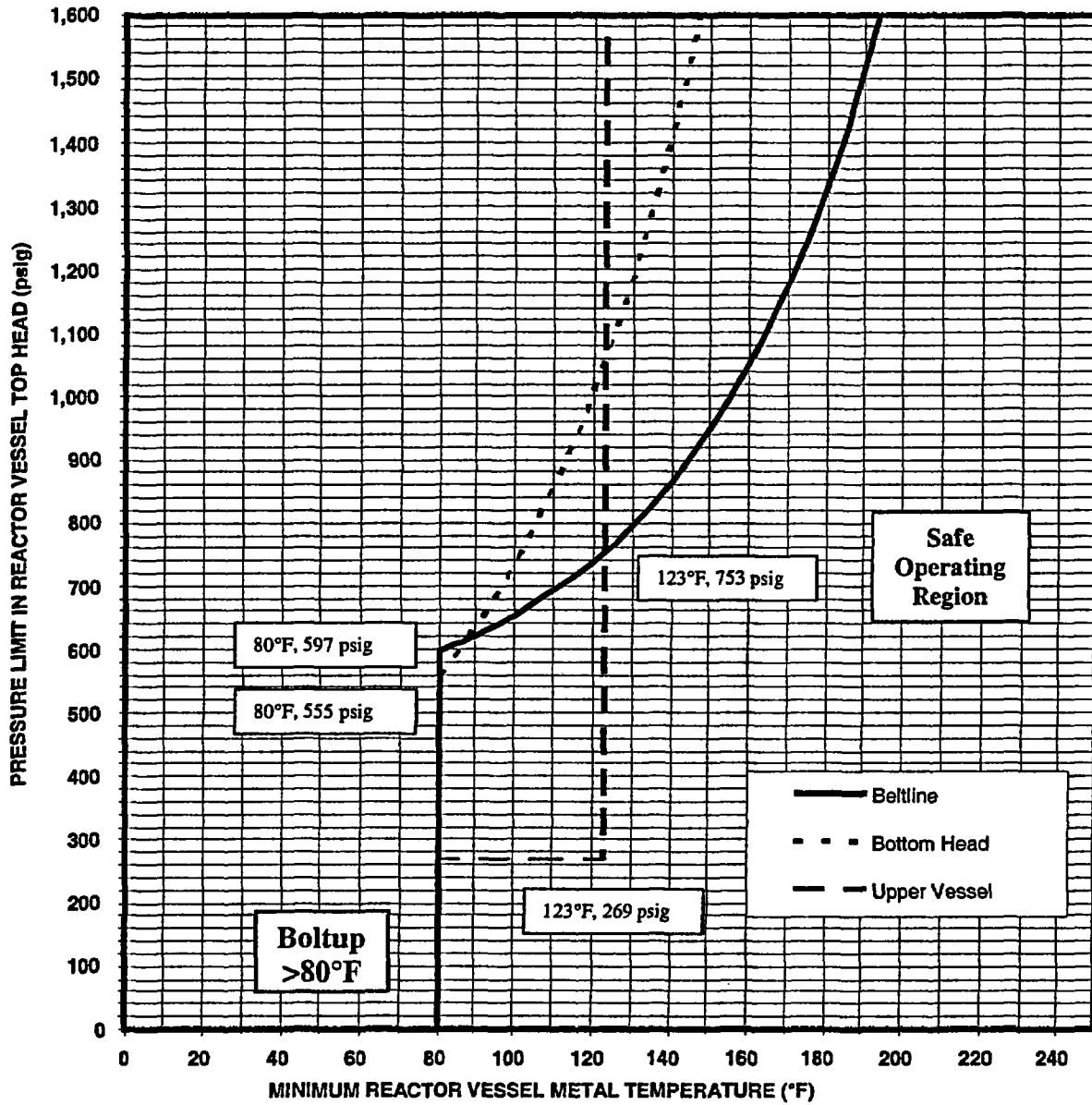
Figure 3.4.9-2 (page 1 of 1) Pressure/Temperature Limits for Inservice Hydrostatic and Inservice Leakage Tests Valid Through End of Cycle 23
