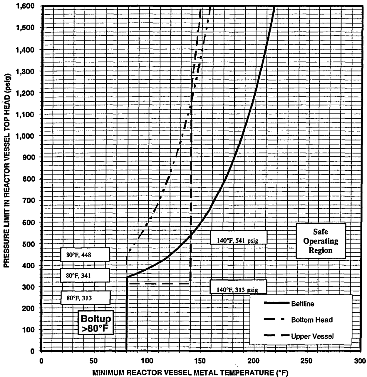
Figure 3.4.9-1 (page 1 of 1) Pressure/Temperature Limits for Non-Nuclear Heatup or Cooldown Following Nuclear Shutdown Valid Through End of Cycle 23
