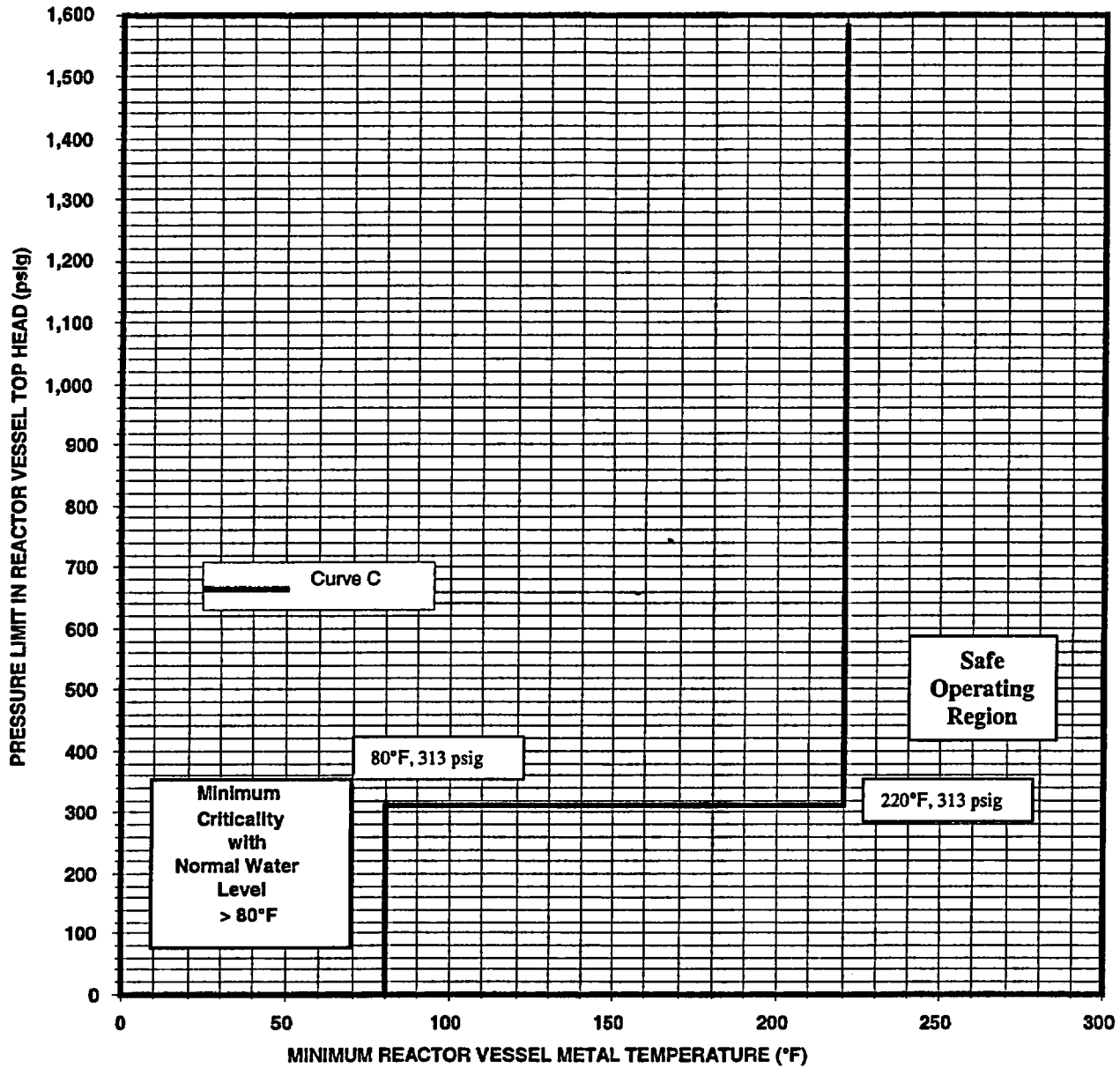
Figure 3.4.9-3 (page 1 of 1) Pressure/Temperature Limits for Criticality Valid Through End of Cycle 23
