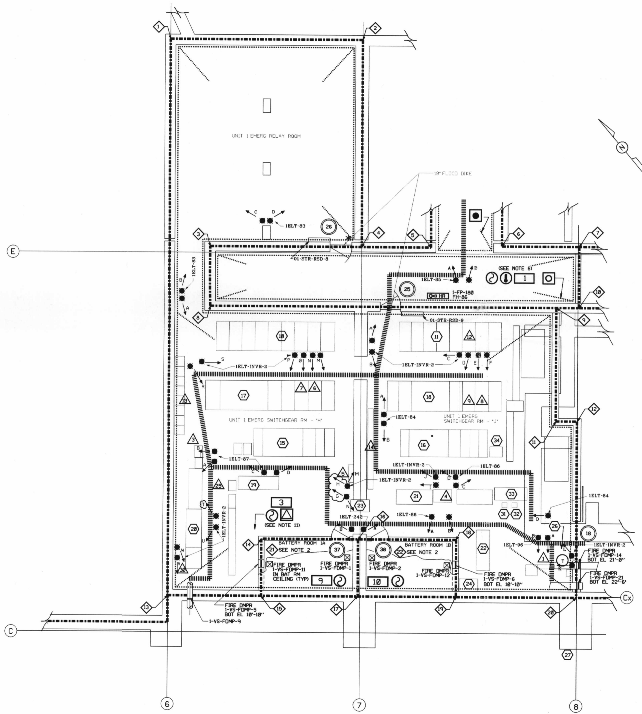
PLAN - EL. 9'-6"
