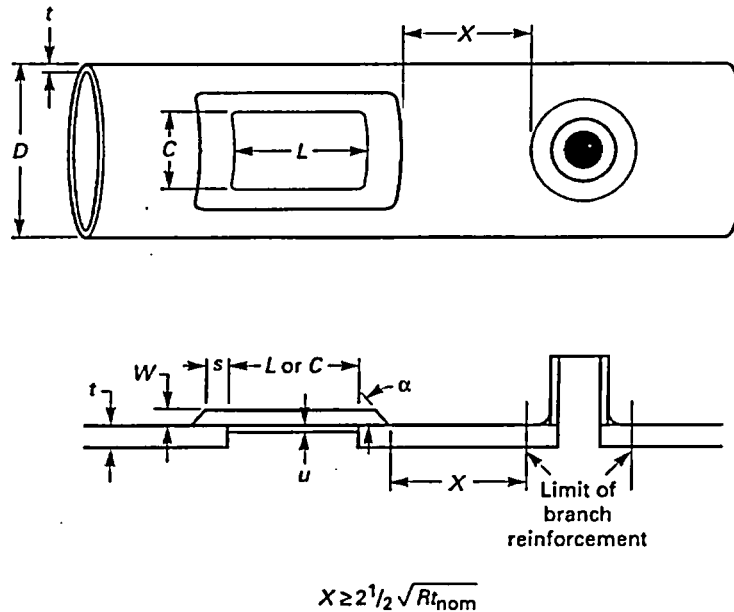
FIG. 1 BRANCH REINFORCEMENT
