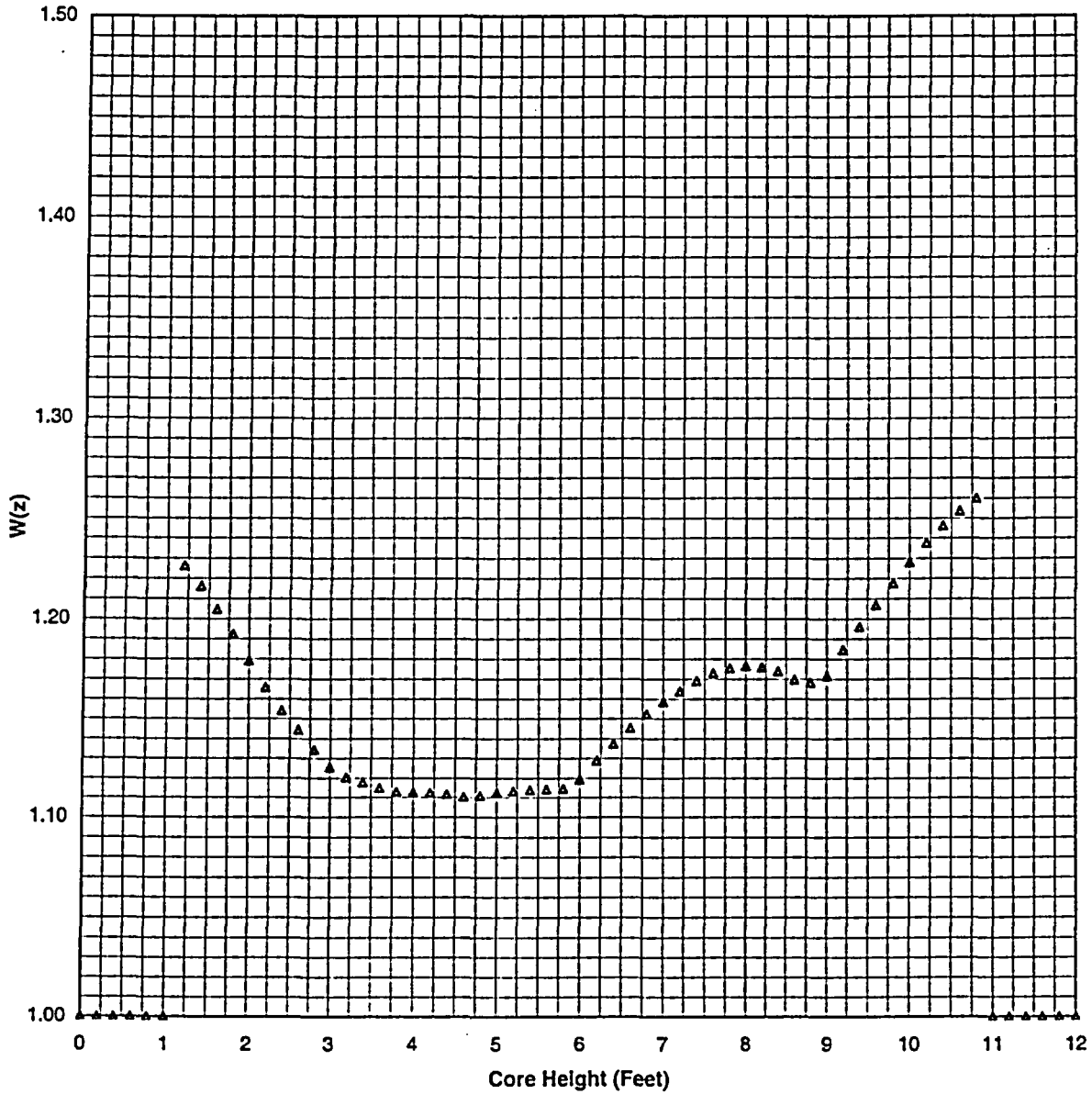
Figure 5a RAOC Summary of W(z) at 9500 MWD/MTU
