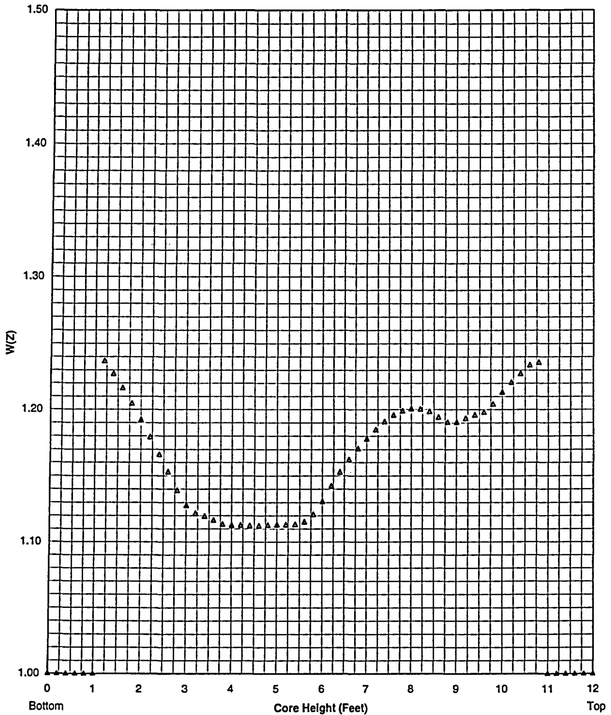
Figure 5b RAOC Summary of W(Z) at 12000 MWD/MTU
