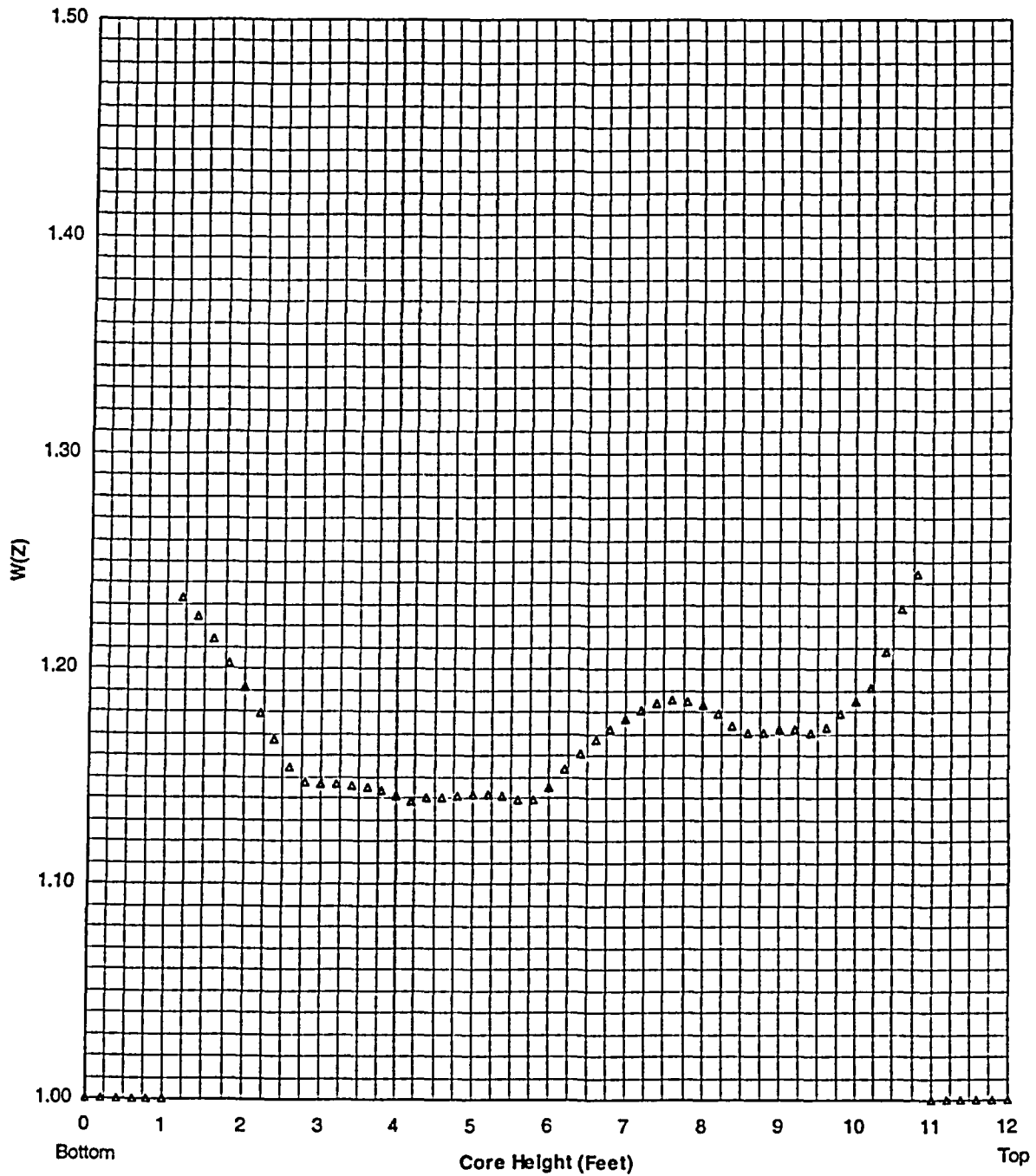
Figure 5c RAOC Summary of W(Z) at 16000 MWD/MTU
