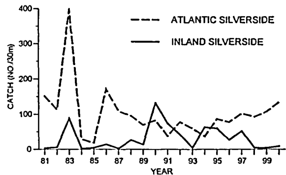
Fig. 6. Annual \Delta -mean CPUE (no./30 m) of Atlantic silverside (dashed line) and inland silverside (solid line) taken by seine at station JC from 1981 through 2000.
