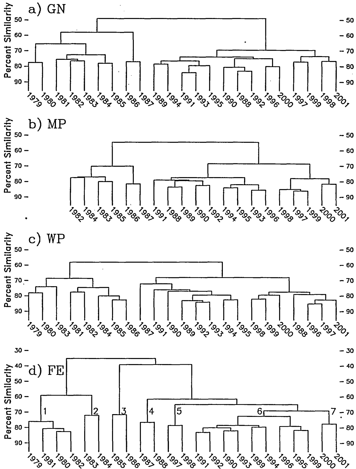
Fig. 3. Clustering dendrogram of percent similarity of qualitative algal collections, by year, at rocky intertidal sampling stations. Numbered groups at FE are further characterized in Table 1.
