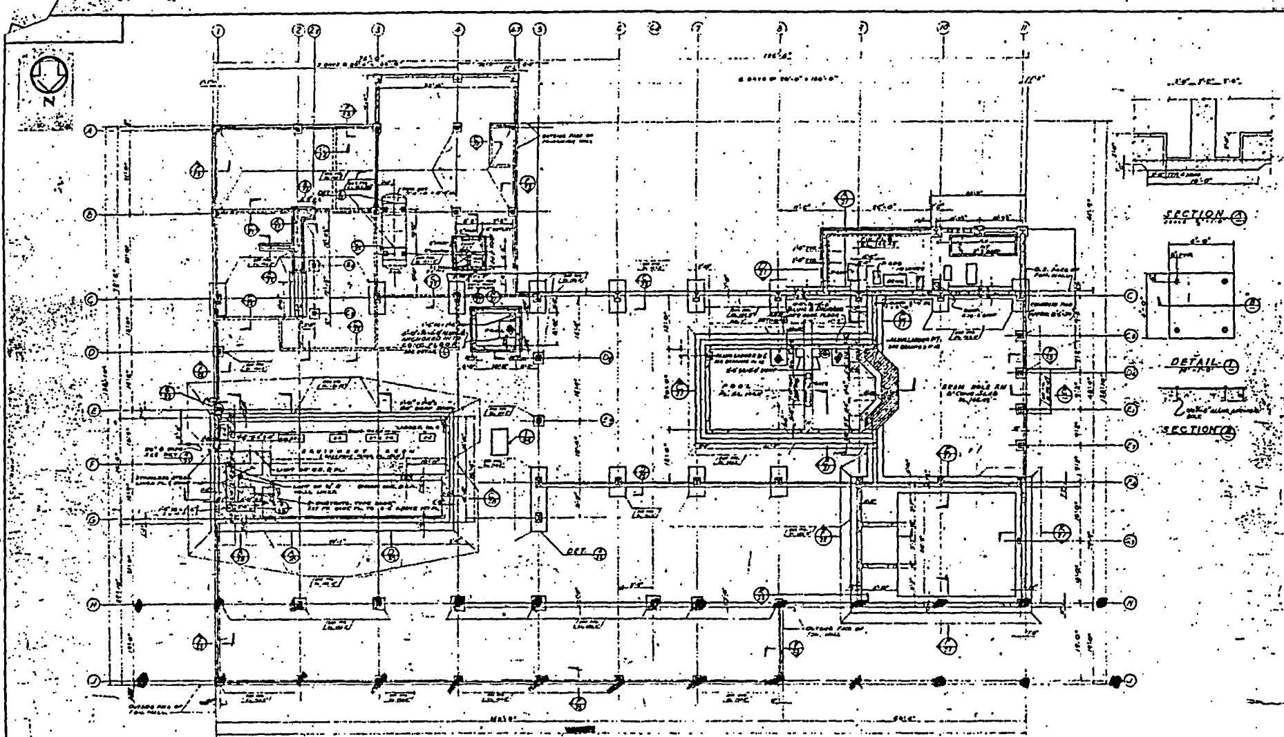
FINISH FLOOR EL. 160'-0" BASEMENT AND FOUNDATION PLAN
