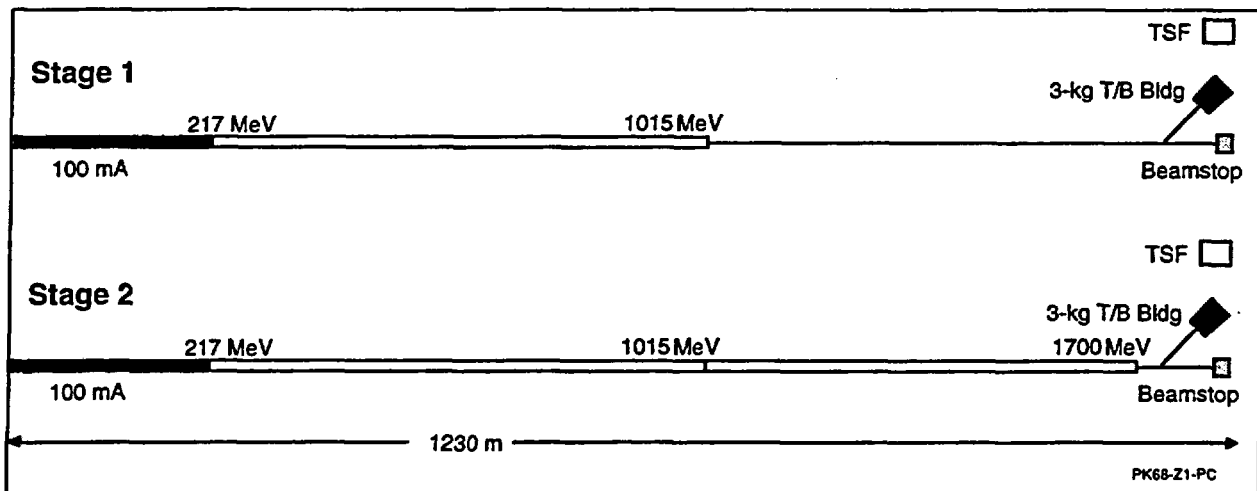
Figure 2-11. Staging with extended linac tunnel.
