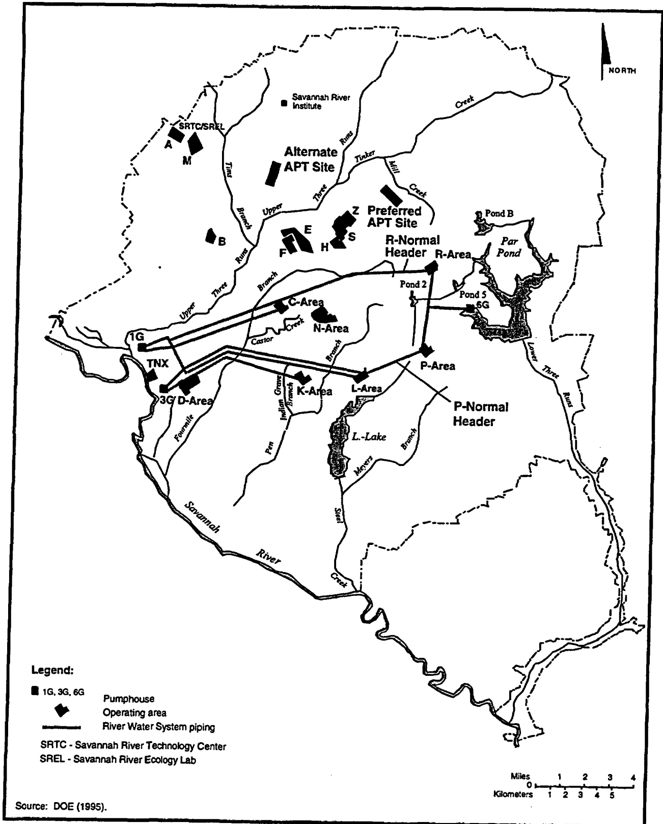
Figure 2-5. Map of the SRS showing existing features that could be used to provide cooling water for the accelerator.
