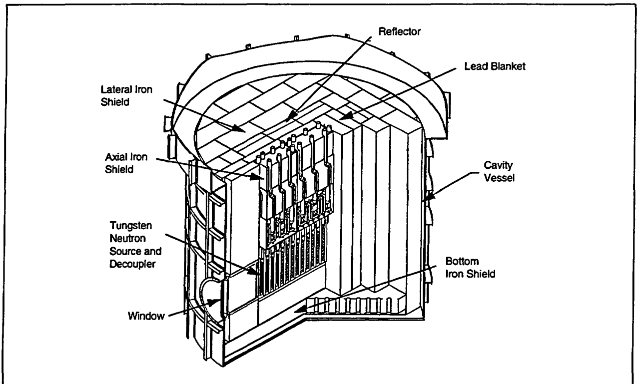
Figure A-13. Target/blanket assembly (LANL 1997).
