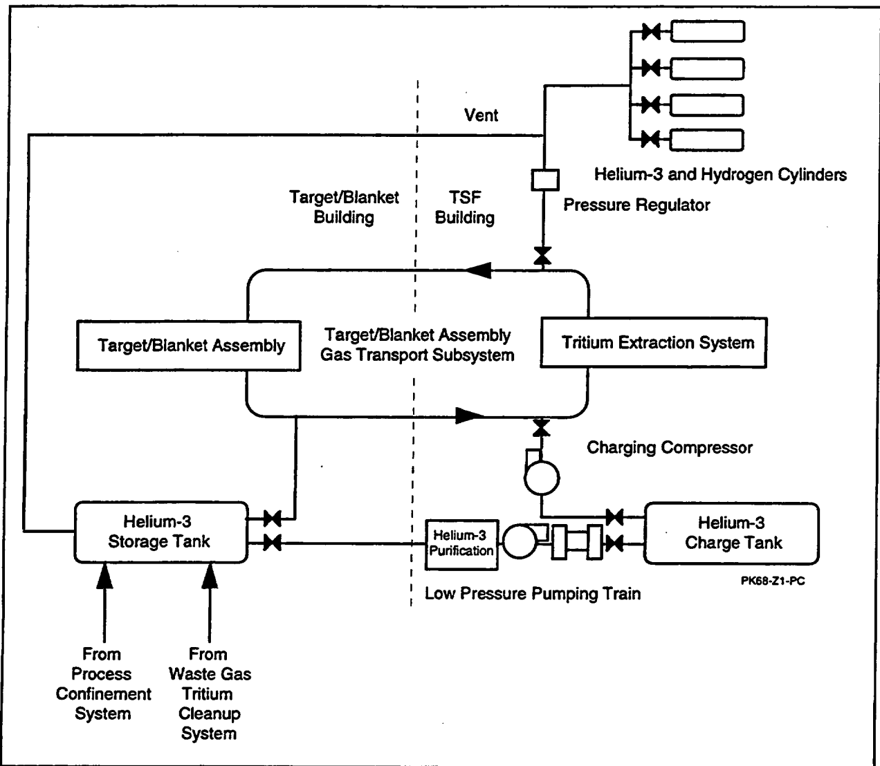
Figure A-22. Helium supply system (LANL 1997).
