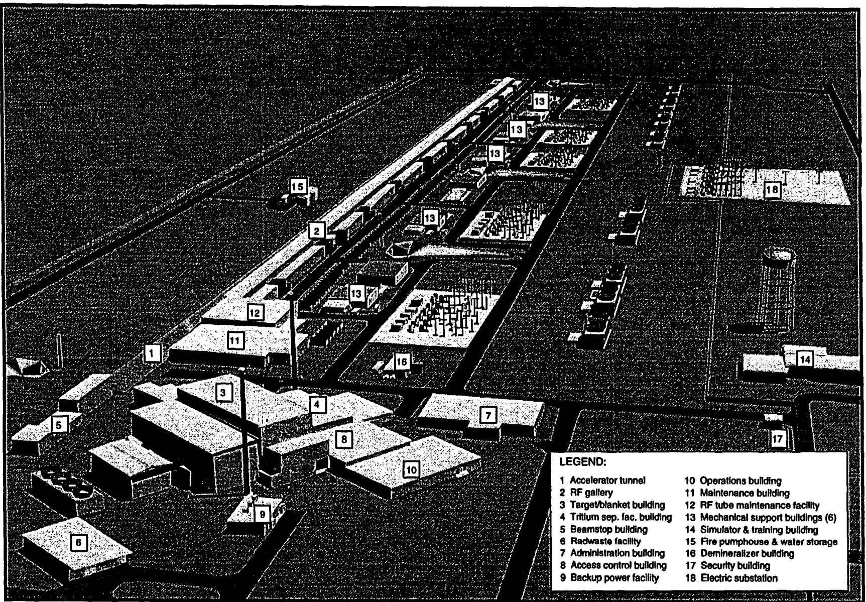
Figure A-1. Conceptual layout of APT facilities and structure (LANL 1997).
