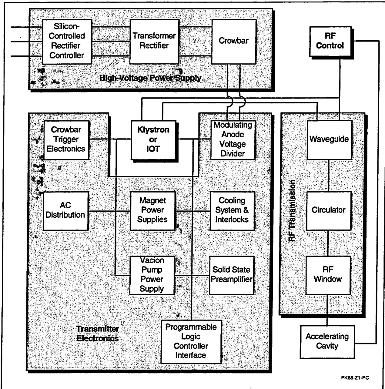
Figure A-9. Block diagram of RF Power System (LANL 1997).
