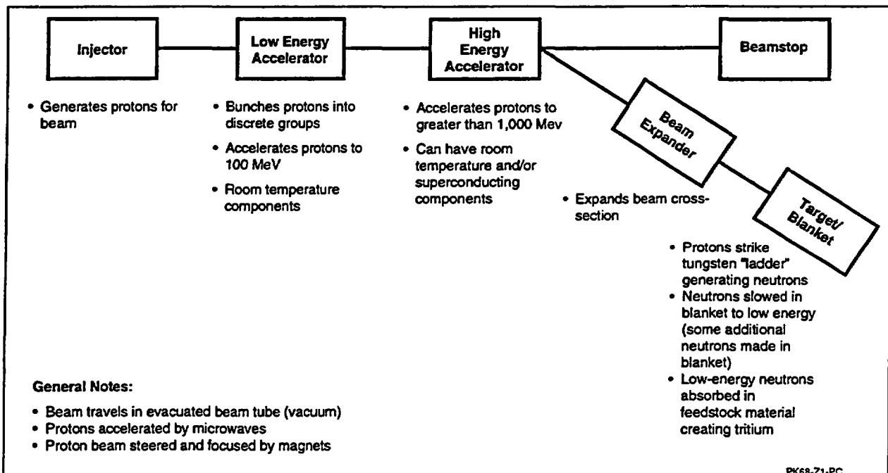
Figure 2-2. Accelerator schematic.
