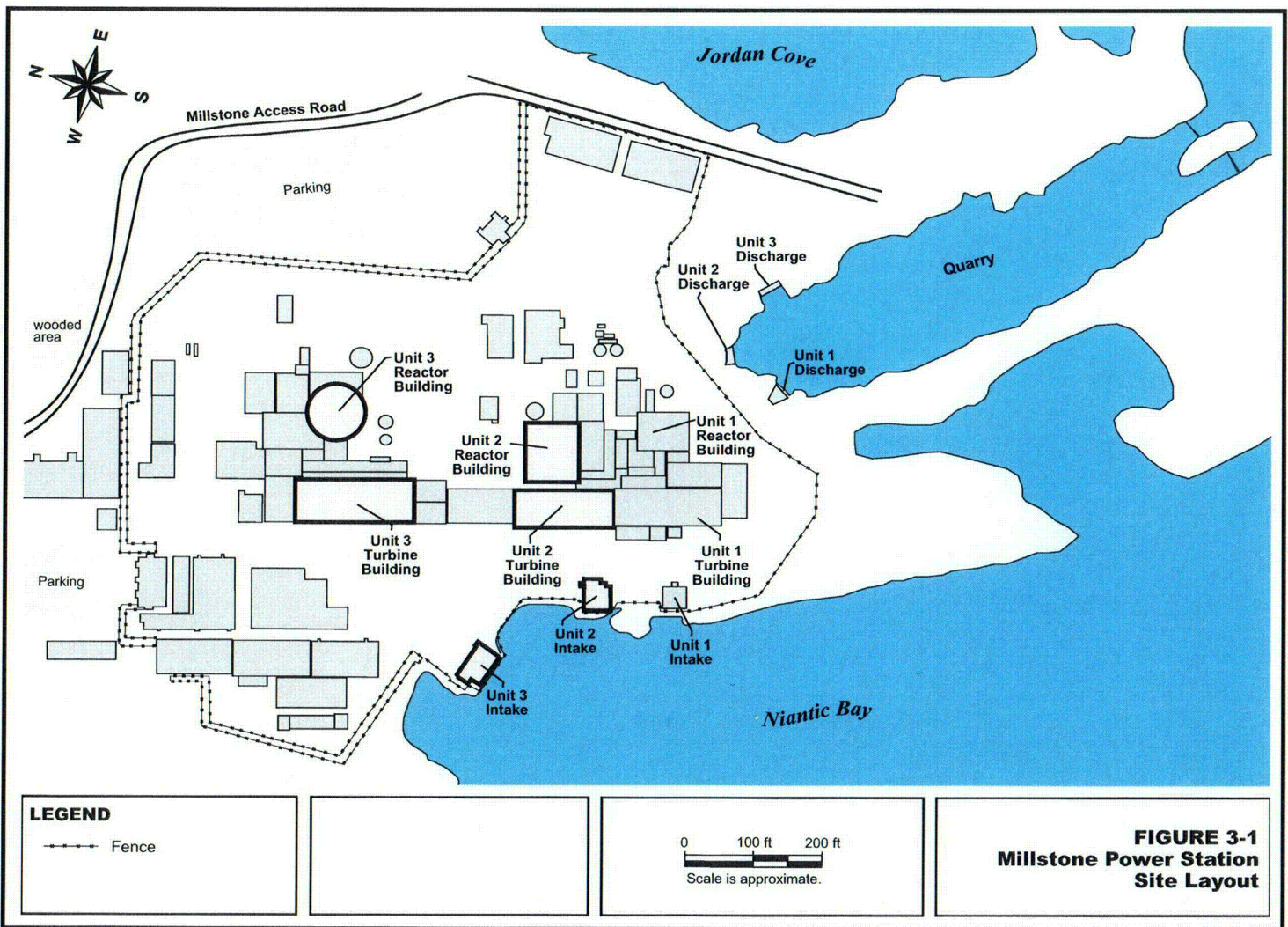
Figure 3-1 Millstone Power Station Site Layout
