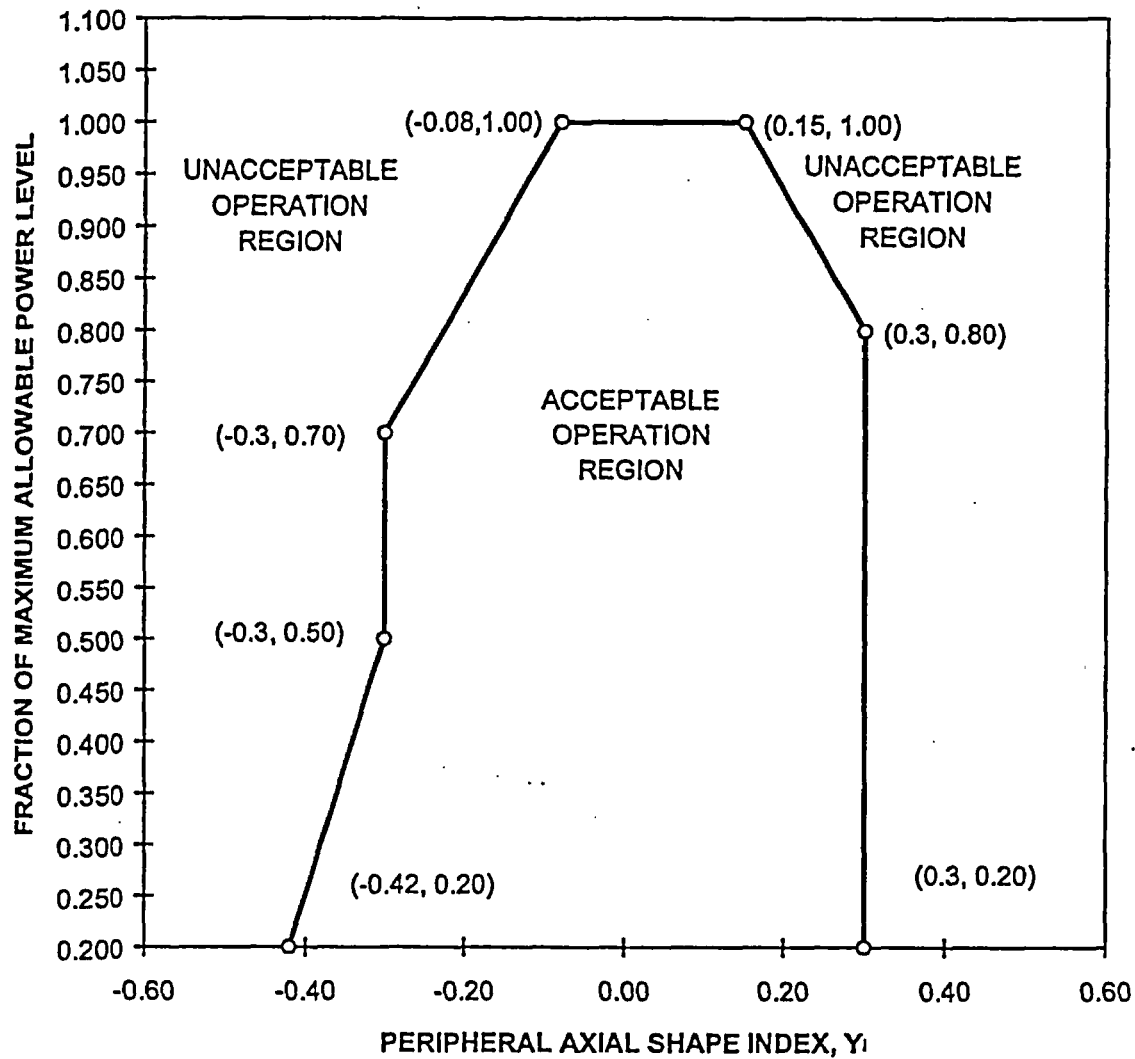
Figure 3.2.5 DNB Axial Flux Offset Control Limits (See NEOP-13 for Administrative Limits)
