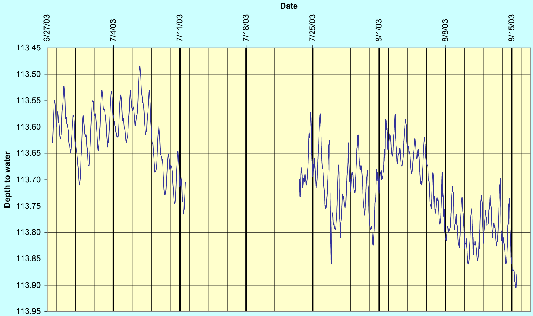
Figure 3-4 Well 402 Background Water Level Monitoring
