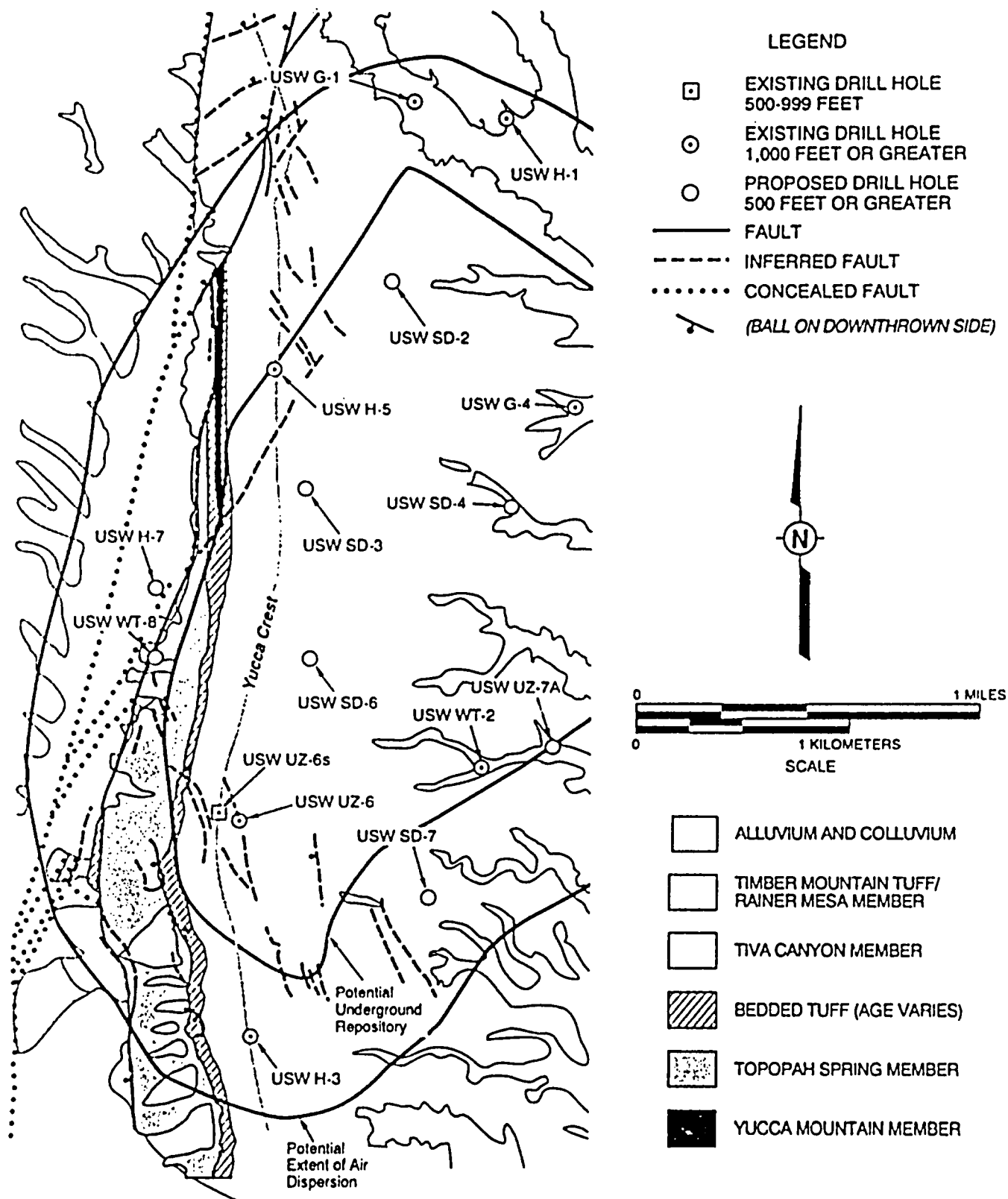
Figure 4-11 Geologic Map of Yucca Crest
