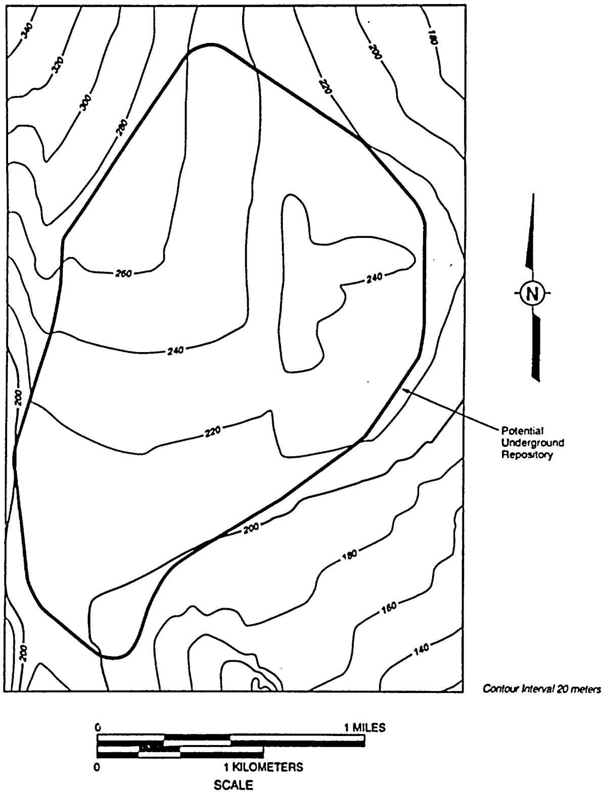
Figure 3-38 Thickness of the Topopah Spring Member Above the Repository Floor (REF0284) 3-60
