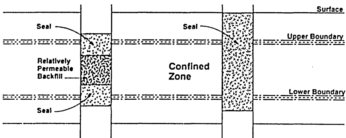
Complete Sealing of the Confined Zone
