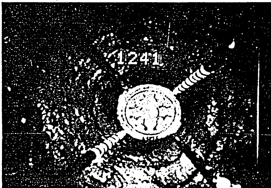
Figure 3-34 UE-25 WT#18; Topopah Spring Member; Densely Welded, Devitrified; 1,241 ft. (C2); Borehole Diameter—12.25 in.
