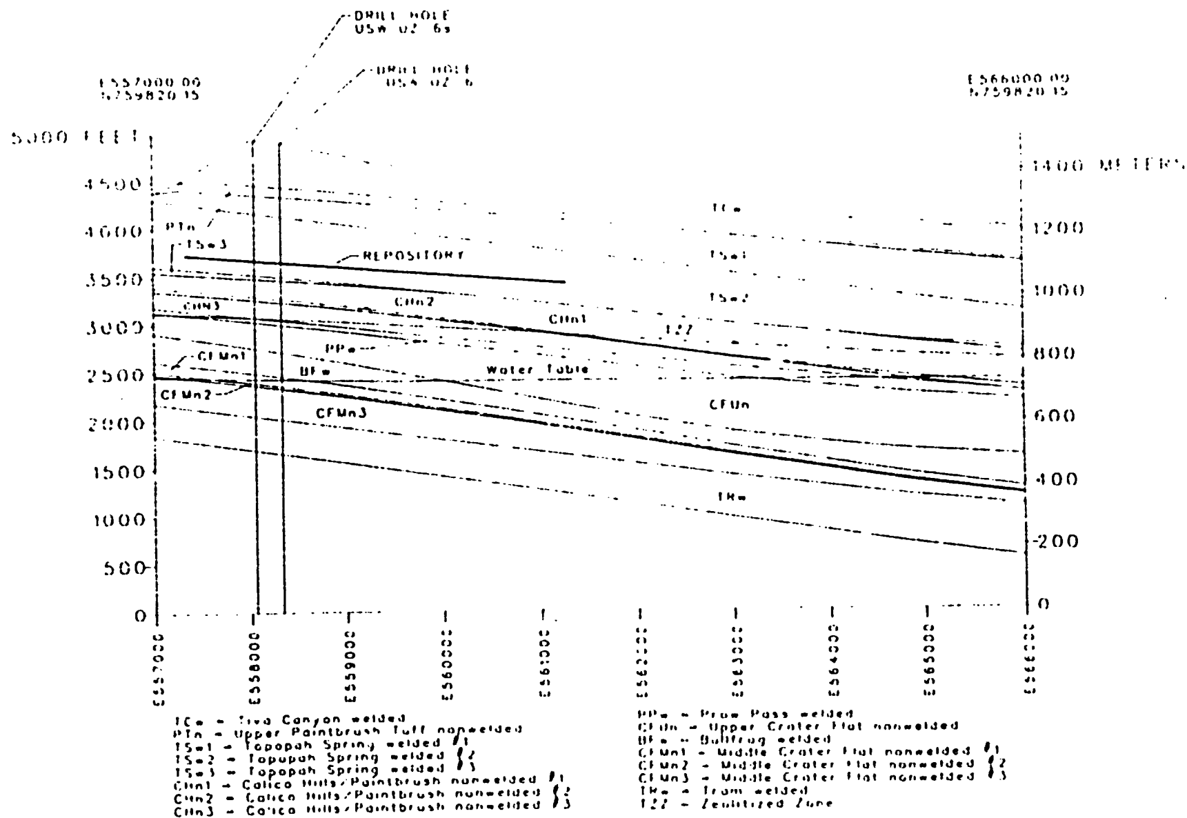
WEST-EAST SECTION THROUGH MIDPOINT BETWEEN USW 02 6 AND USW 02 6s
