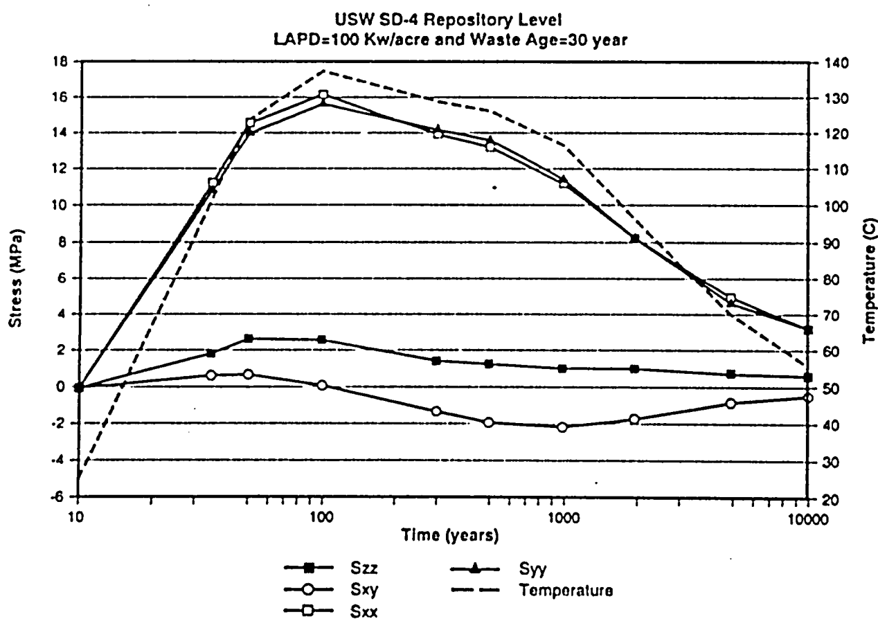
Figure 3-16 Development of Temperature and Thermal Stress for USW SD-4 (Local Areal Power Density of 100 kW per Acre) for Seal Locations 1 and 2
