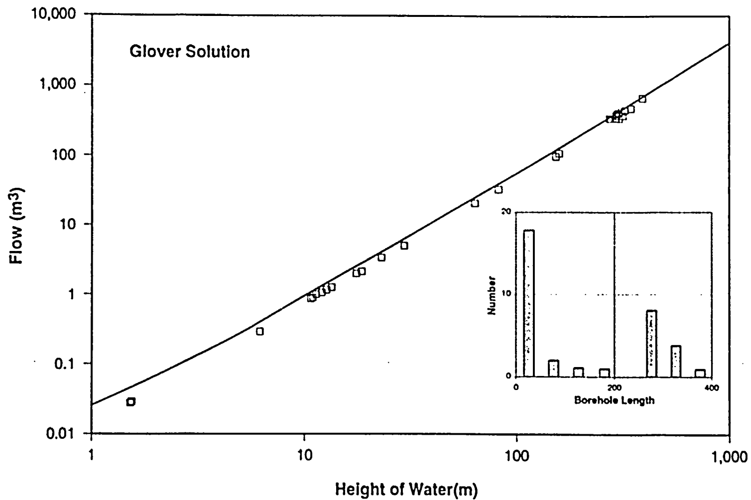
Figure 4-5 Hydrologic Significance of Borehole Seals Glover Solution
