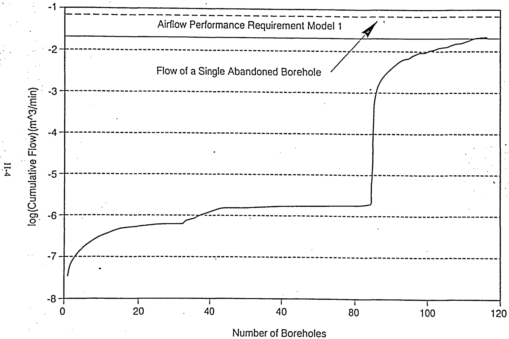
Figure H-2 Cumulative Flow for Model 1
