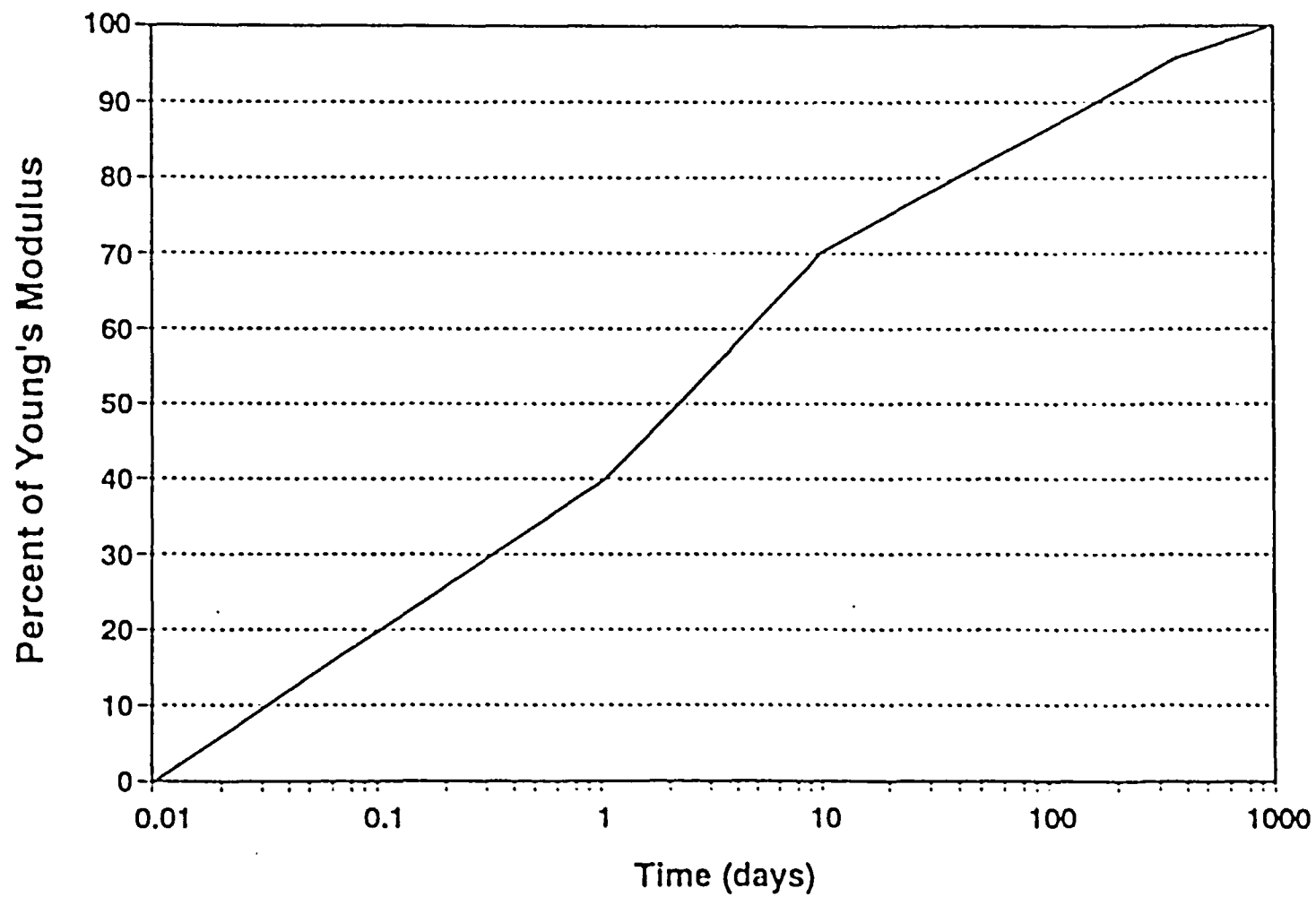
Figure 1-2 Evolution of Young's Modulus for a Cementitious Material
