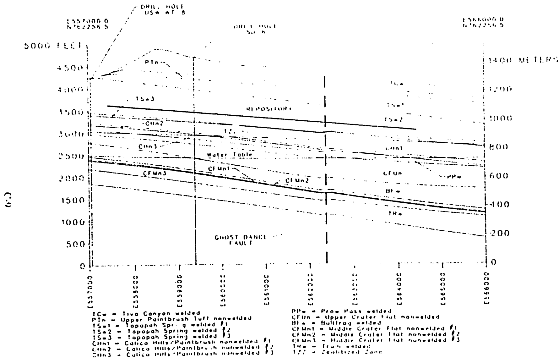
WEST-EAST SECTION THROUGH MIDPOINT BETWEEN USW WT 8 AND SD 6
