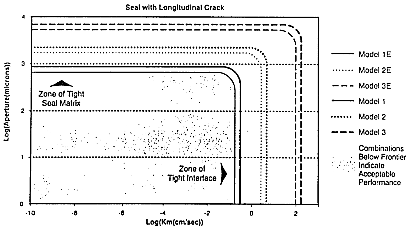
Figure 5-2 Airflow Performance Requirements for Seals (a) No Longitudinal Crack and (b) with Longitudinal Crack
