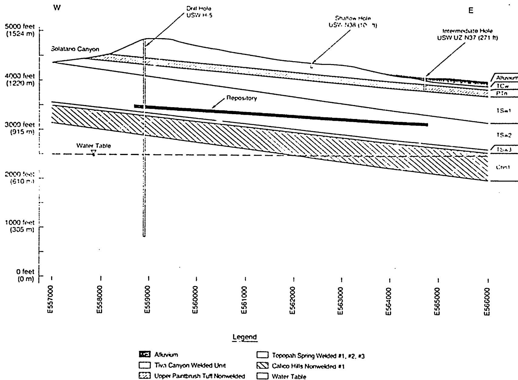
Figure 2-1 Typical Boreholes at Yucca Mountain
