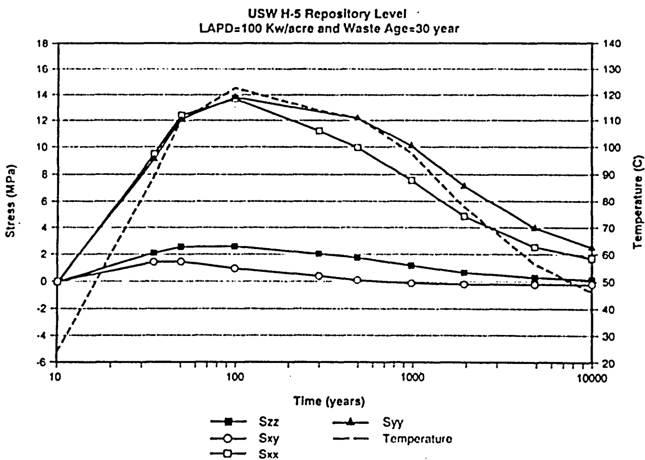
Figure 3-19 Development of Temperature and Thermal Stress for USW H-5 (Local Areal Power Density of 100 kW per Acre) for Seal Locations 1 and 2
