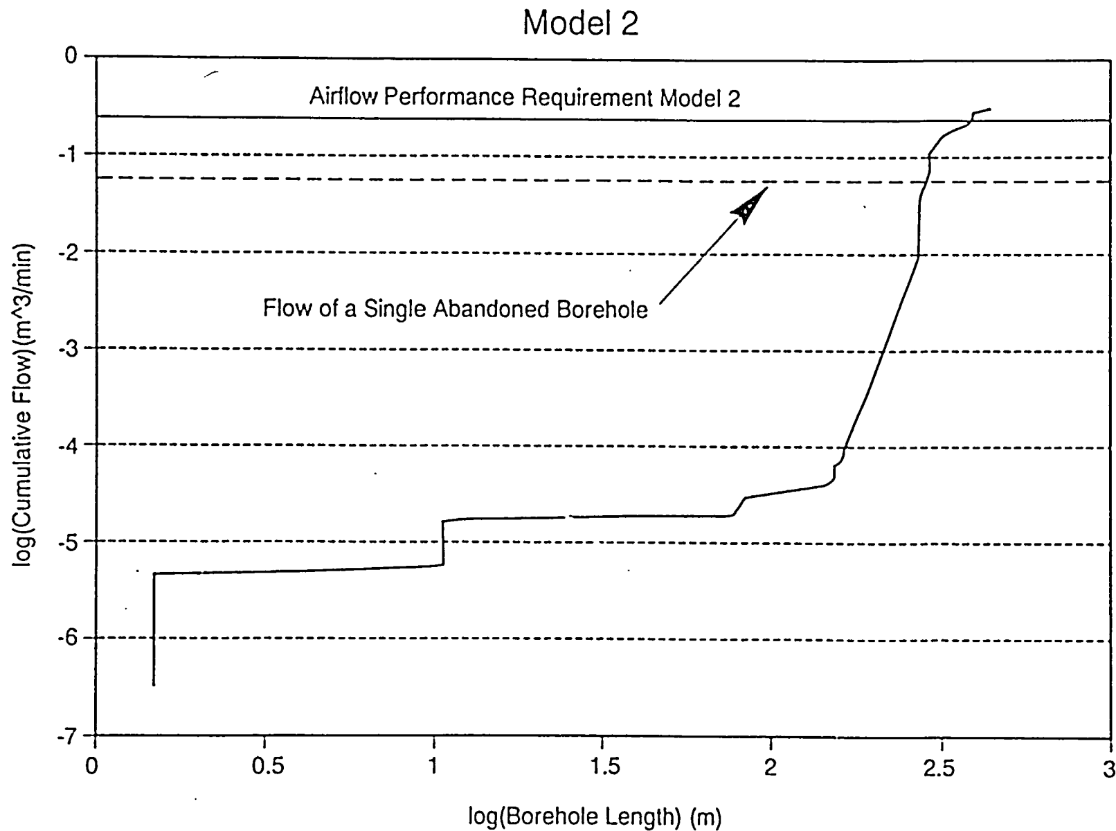
Figure H-6 Cumulative Flow Versus Borehole Length – Model 2
