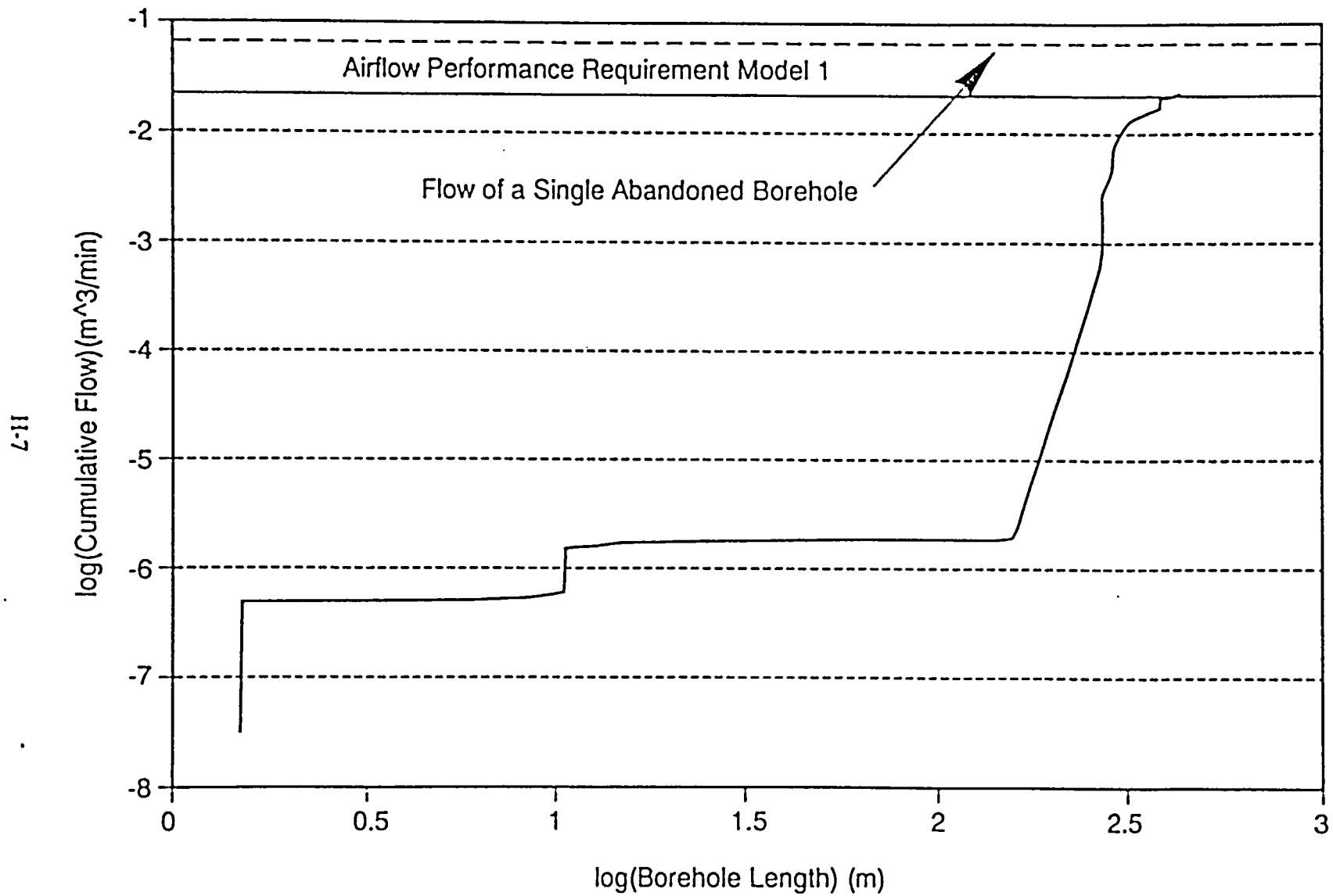
Figure H-5 Cumulative Flow Versus Borehole Length – Model 1
