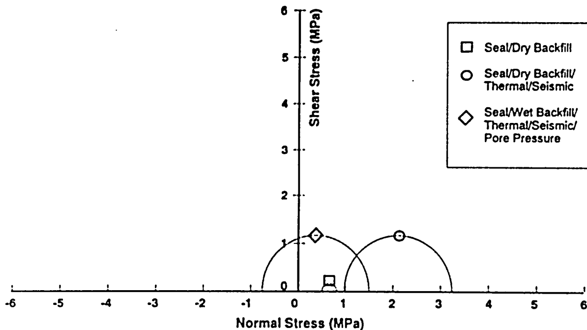
Figure 5-14 Evaluation of Scenarios in the (a) Rock and (b) Seal at the Upper Sealing Location
