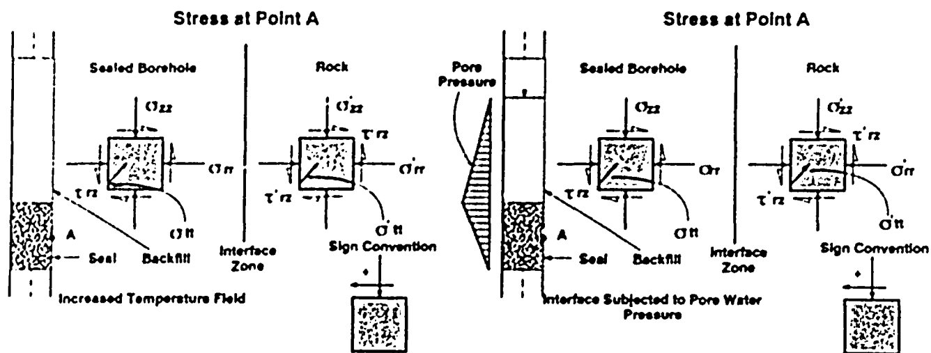
State of Stress After Backfilling and Waste Emplacement
