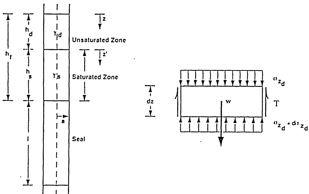
Seal Geometry
