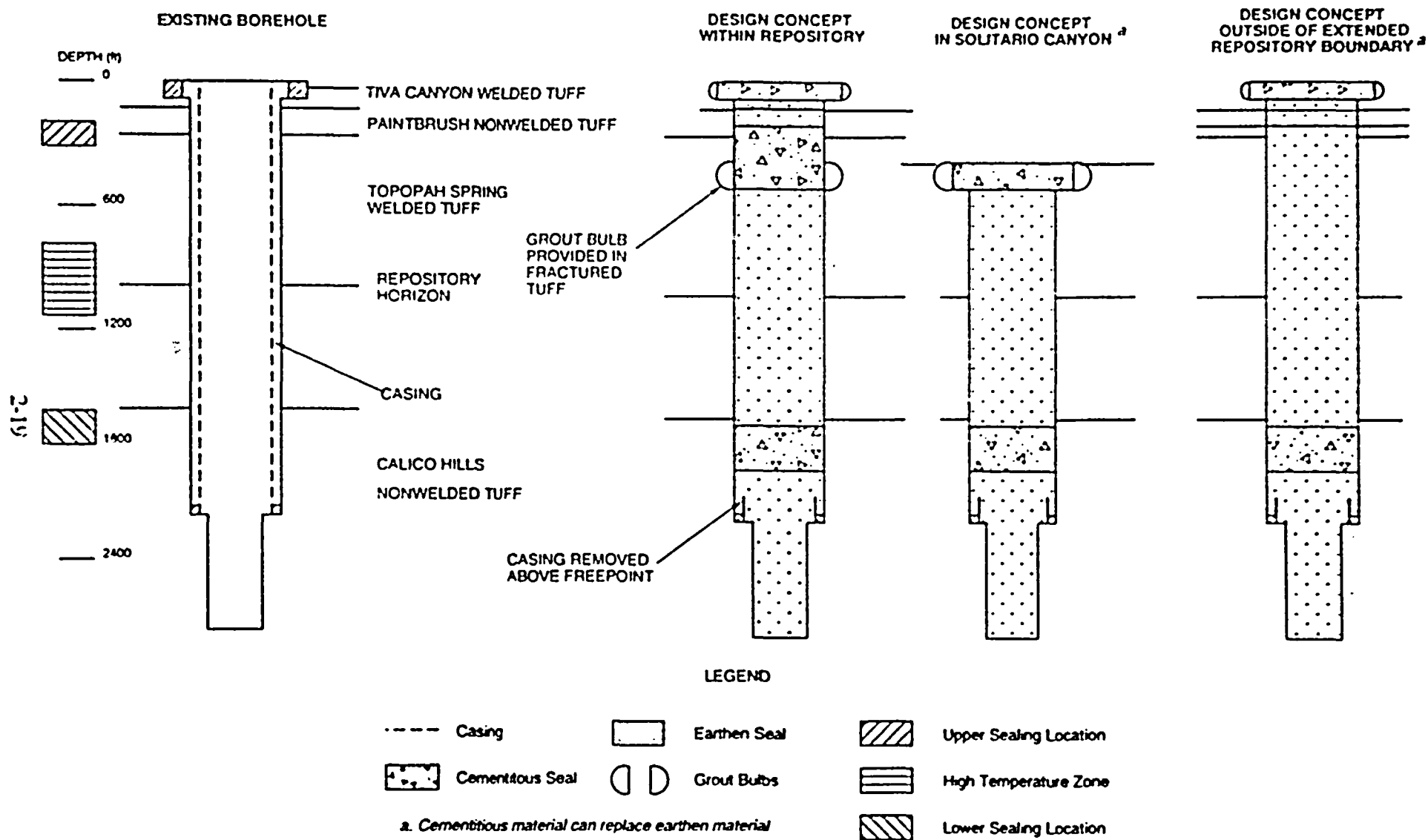
Figure 2-8 Design Concepts for Sealing Exploratory Boreholes
