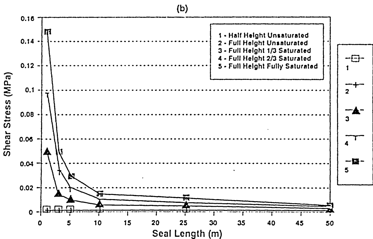
Figure J-3 Structural Analysis of Rockfill at the Potential Repository Horizon (a) Static Loading and (b) Dynamic Loading
