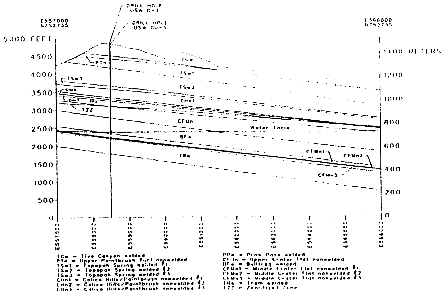
WEST-EAST SECTION THROUGH MIDPOINT BETWEEN USW G-3 AND USW GU-3
