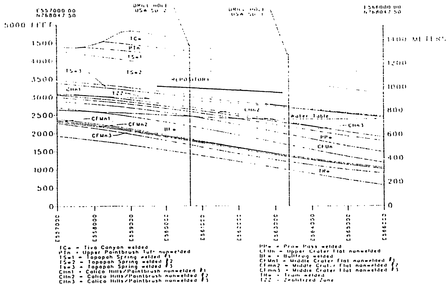
WEST-EAST SECTION THROUGH MIDPOINT BETWEEN USW 50-1 AND USW 50-2
