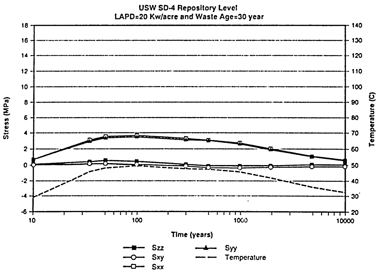
Figure 3-14 Development of Temperature and Thermal Stress for USW SD-4 (Local Areal Power Density of 20 kW per Acre) for Seal Locations 1 and 2
