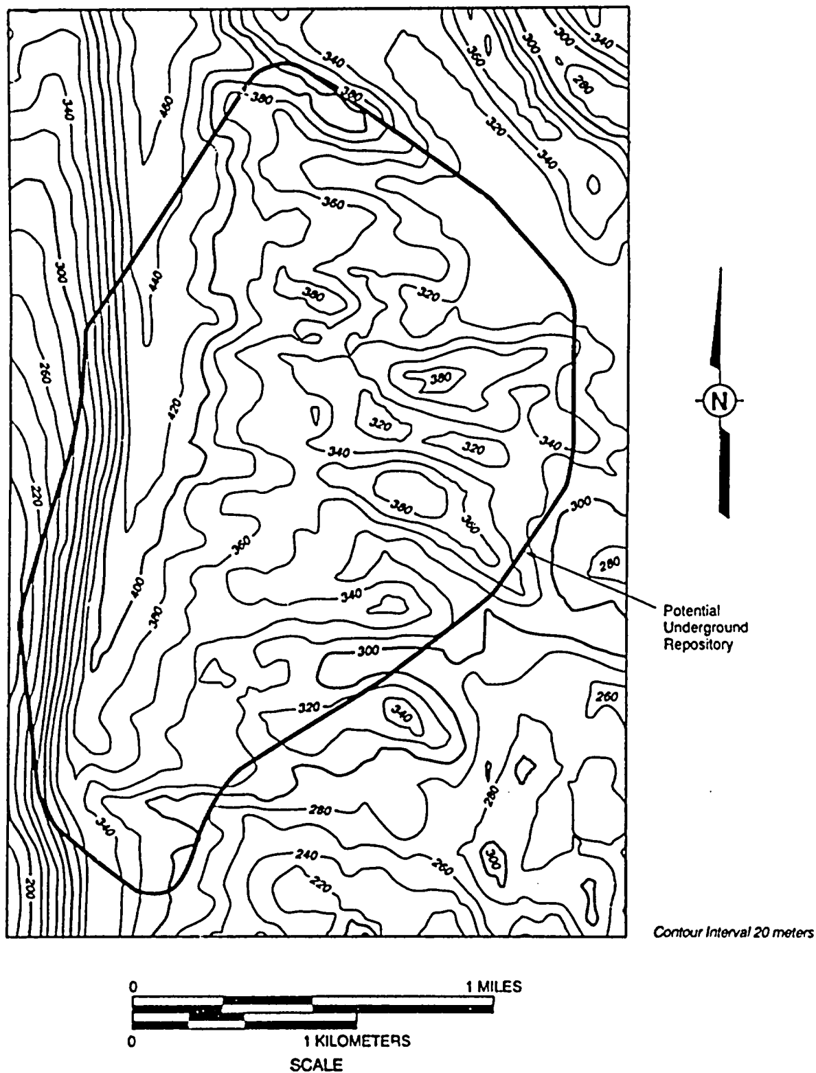
Figure 3-39 Total Thickness of the Rock Above the Repository Floor (REF0283, REF0284, REF0287)
