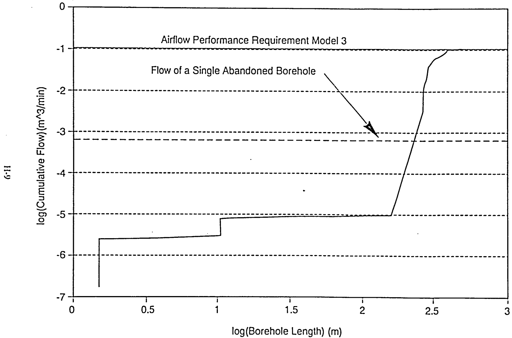
Figure H-7 Cumulative Flow Versus Borehole Length – Model 3
