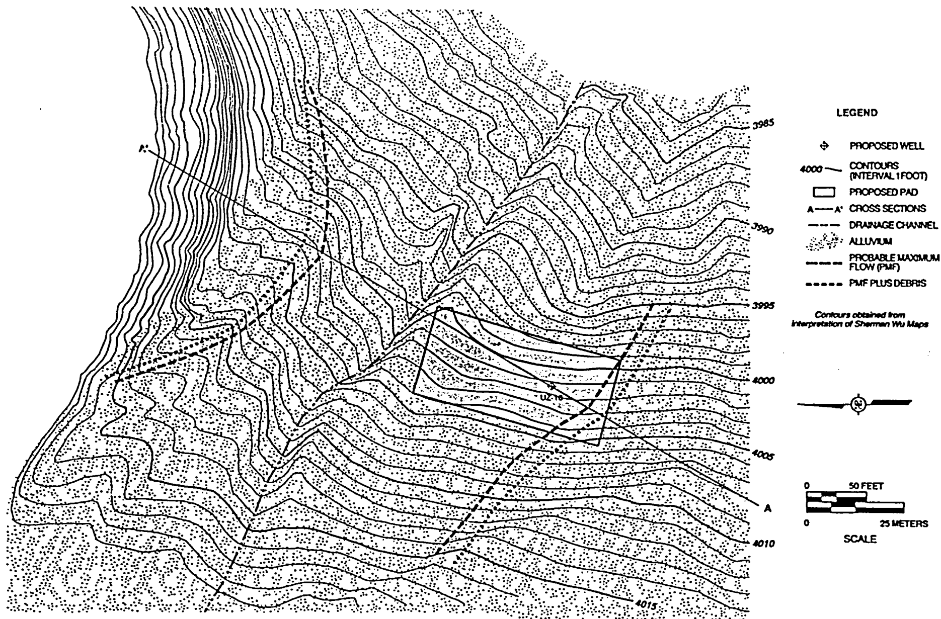
Figure 4-3a Extent of Flooding Near USW UZ-16 (a) Plan View and (b) Topographic Cross Section with Probable Maximum Flood Levels
