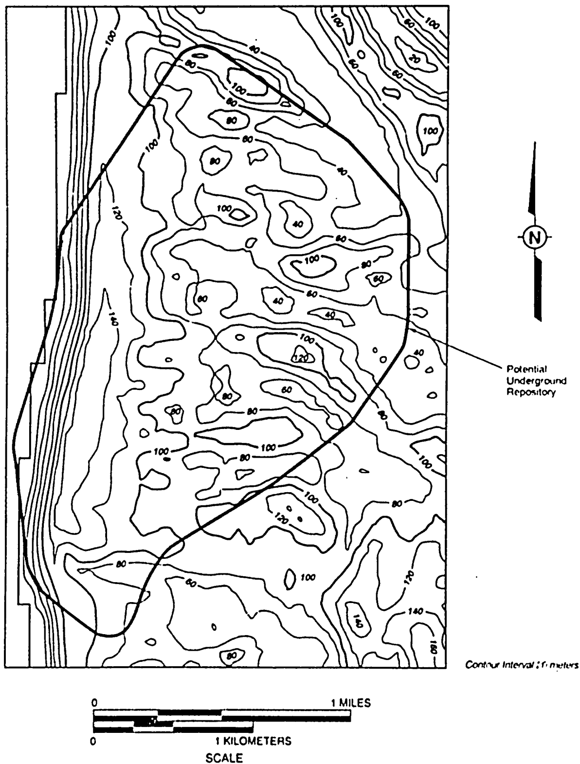
Figure 3-36 Thickness of the Tiva Canyon (TCw) Unit (REF0287)
