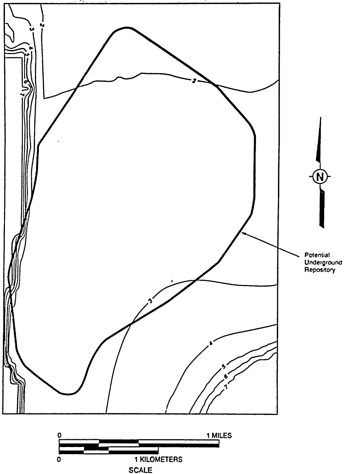
Figure 3-41 Conductance of Stratigraphic Units Above Potential Repository (Ln-value \times 10^9/\text{min} ), Model 2
