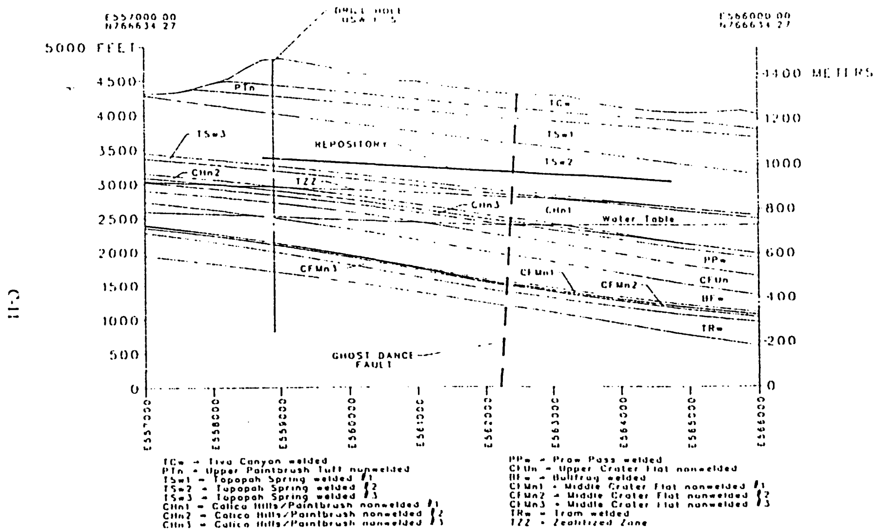
WEST-EAST SECTION THROUGH USW H 5
