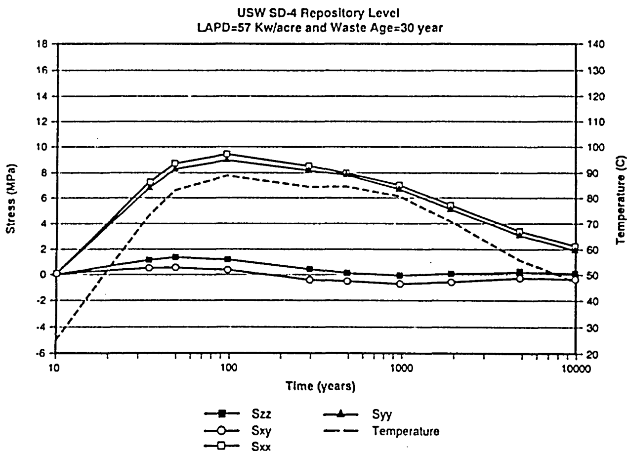
Figure 3-15 Development of Temperature and Thermal Stress for USW SD-4 (Local Areal Power Density of 57 kW per Acre) for Seal Locations 1 and 2
