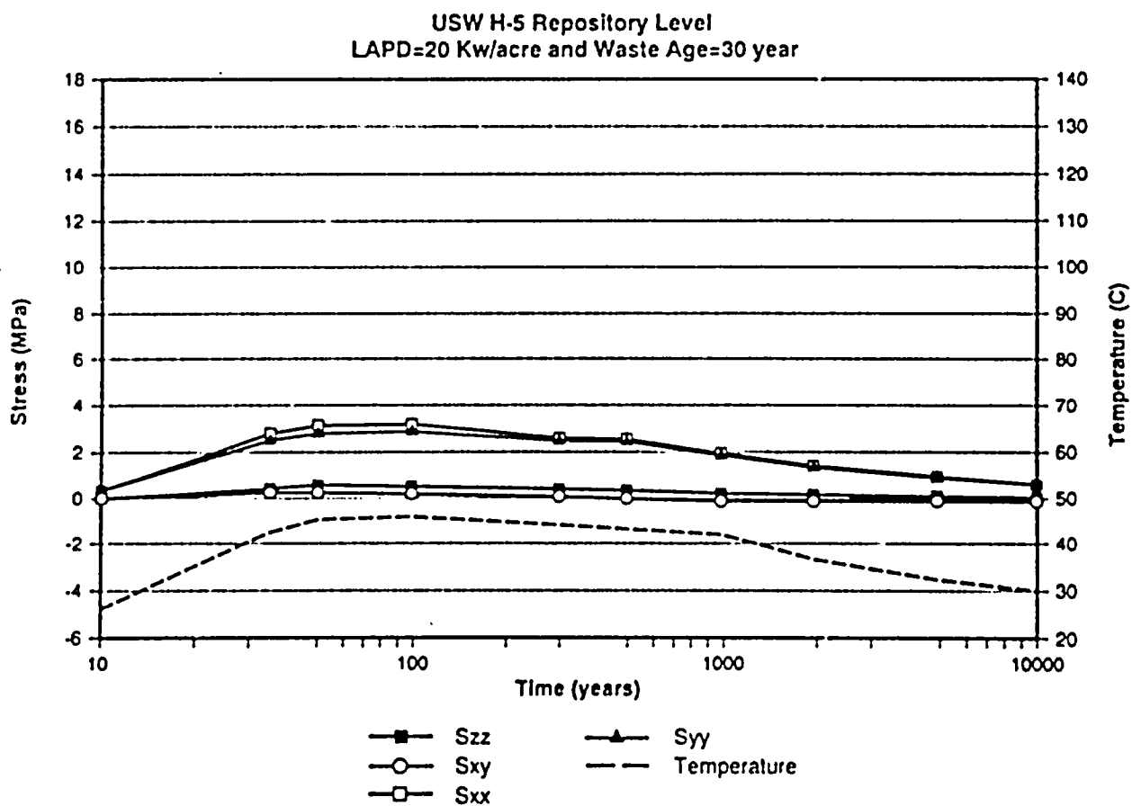
Figure 3-17 Development of Temperature and Thermal Stress for USW H-5 (Local Areal Power Density of 20 kW per Acre) for Seal Locations 1 and 2
