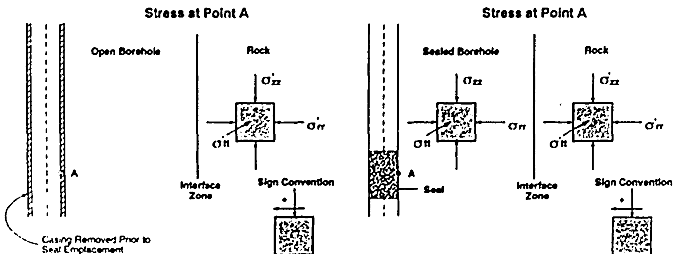
Initial State of Stress in an Open Borehole after Casing Removal
