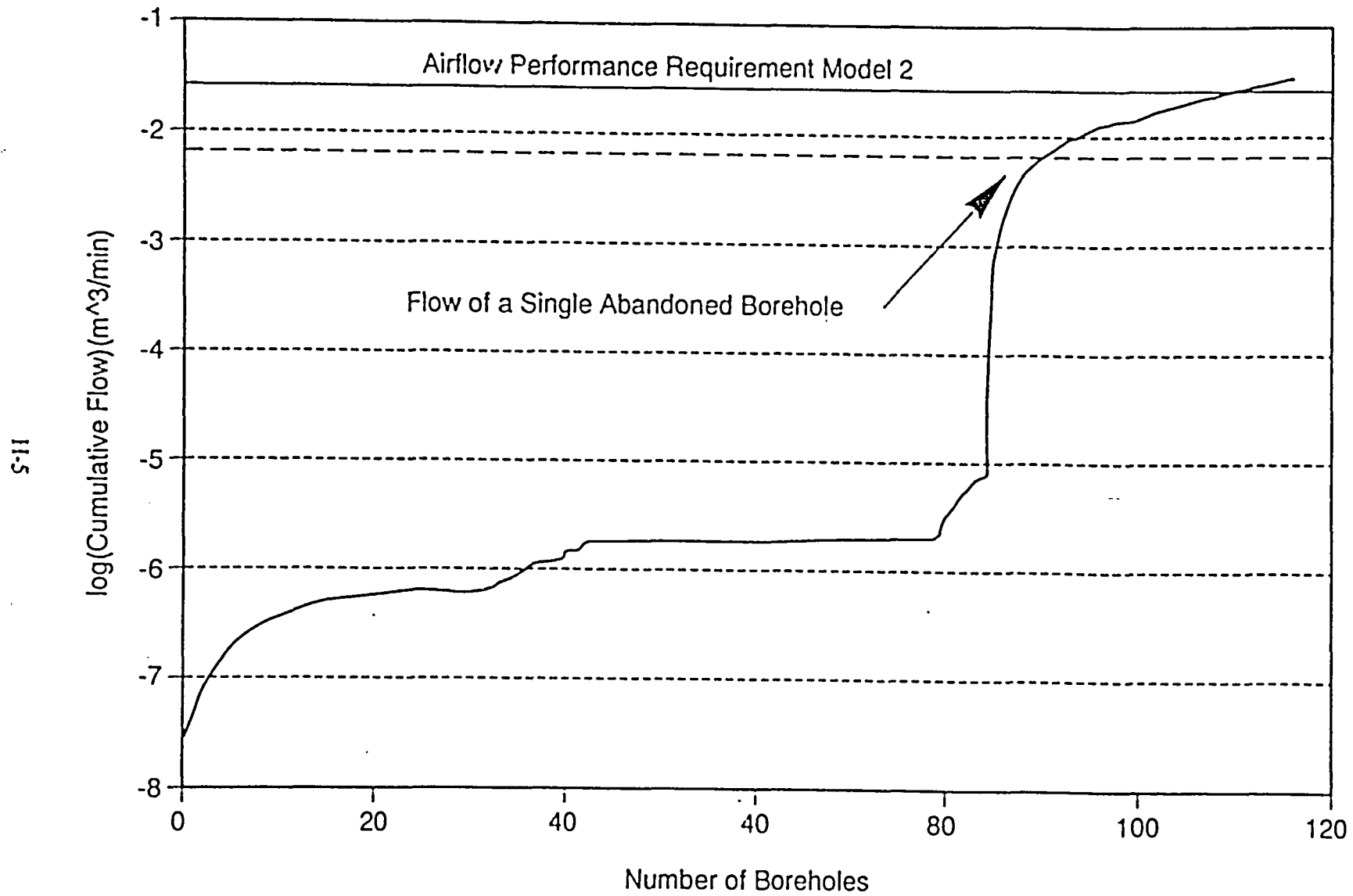
Figure H-3 Cumulative Flow for Model 2
