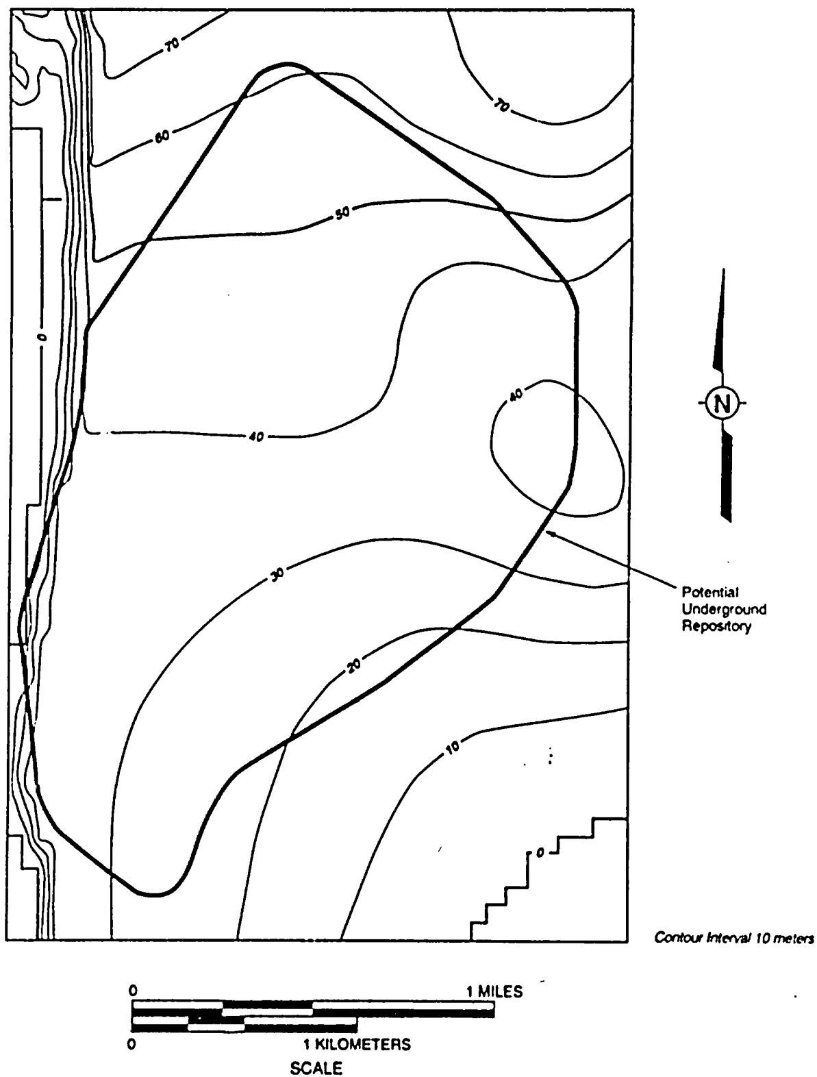
Figure 3-37 Thickness of the Paintbrush Nonwelded (PTn) Unit (REF0283)
