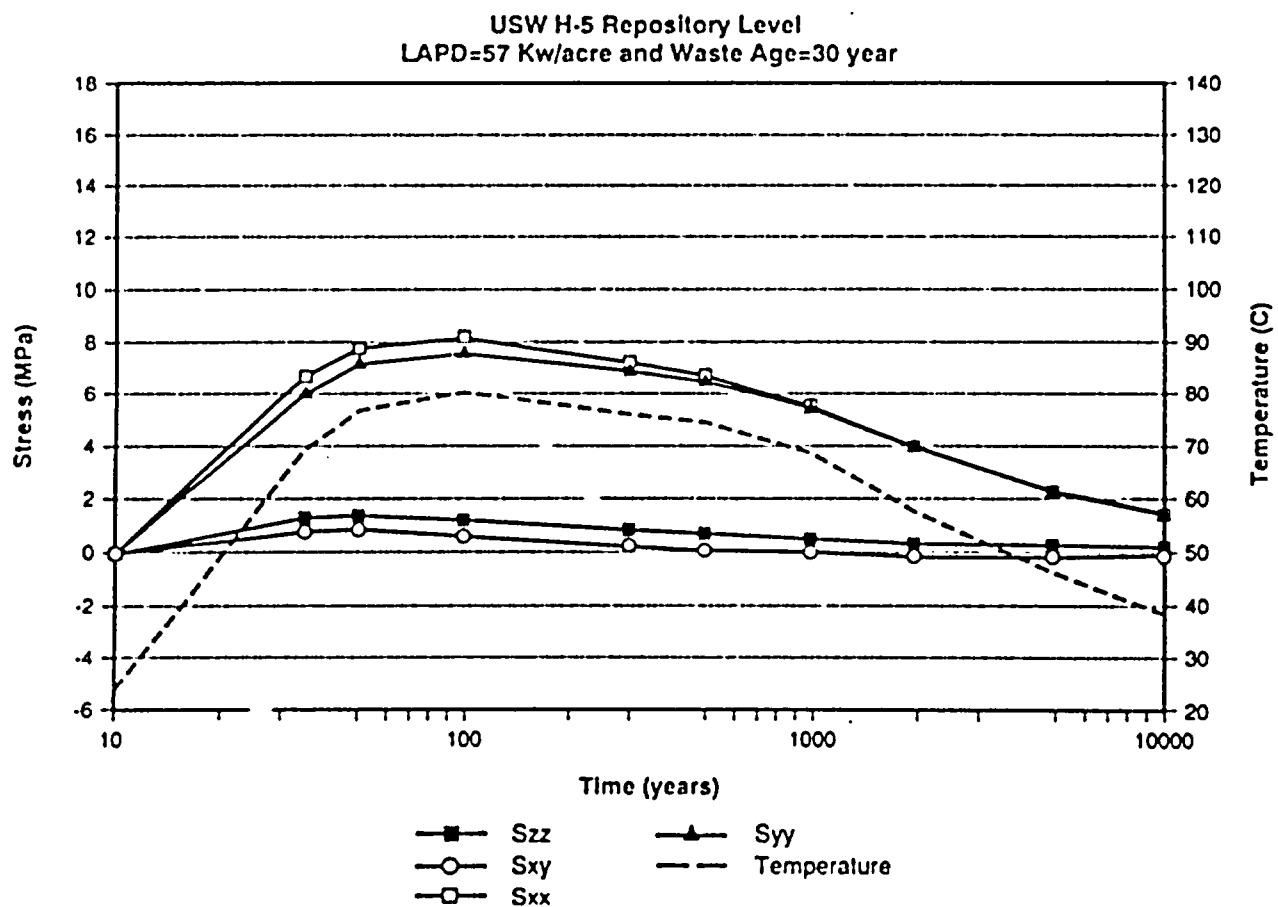
Figure 3-18 Development of Temperature and Thermal Stress for USW H-5 (Local Areal Power Density of 57 kW per Acre) for Seal Locations 1 and 2
