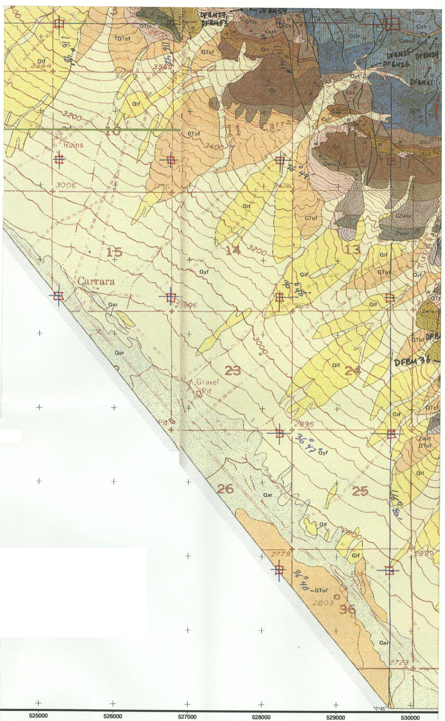
Geologic Map of Bare Mountain Nye County, Nevada From Monsen, et al, 1992 UTM, Zone 11; NAD27 Datum
