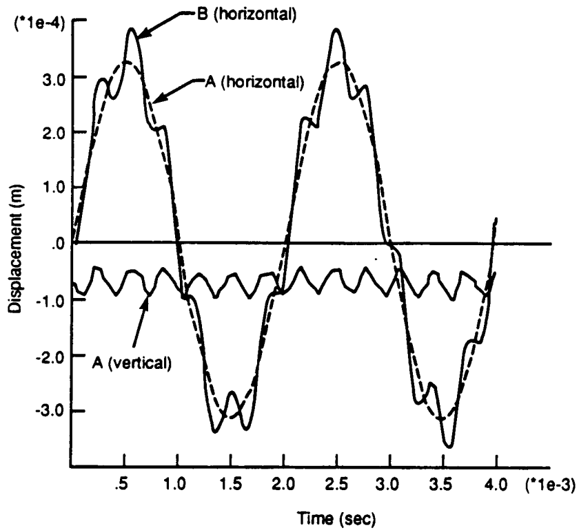
Figure 4-13. Horizontal and vertical displacement histories for 500-Hz input frequency
