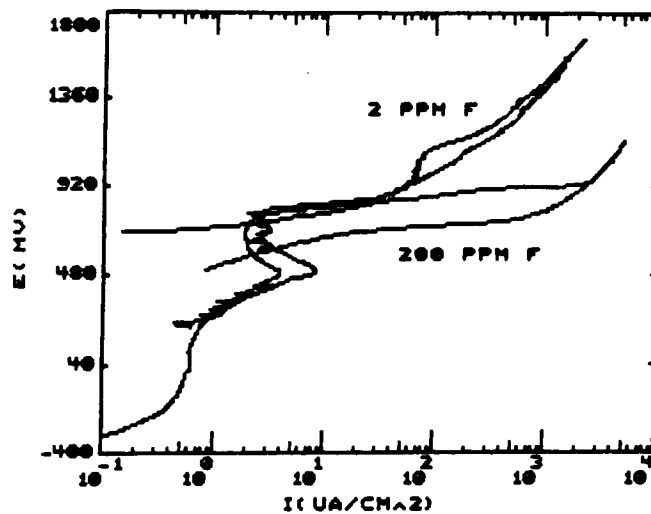
Figure 5-2. Typical cyclic polarization curves for alloy 825 at 95°C indicating the effect of fluoride at a chloride concentration of 6 ppm
