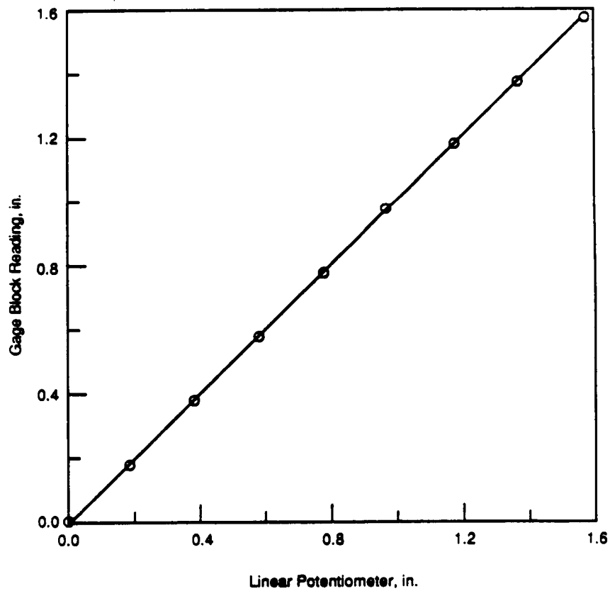
Figure 4-21. Extensometer calibration curve for MPBX No. E, position 3
