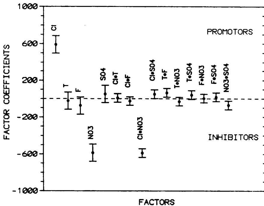
Figure 5-7. The coefficients in Eq. (2) plotted for various factors along with their 95-percent confidence levels
