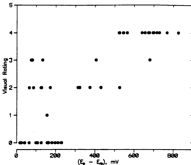
Figure 5-6. E_p - E_{rp} vs. visual rating of specimens indicating a lack of correlation between these two parameters
