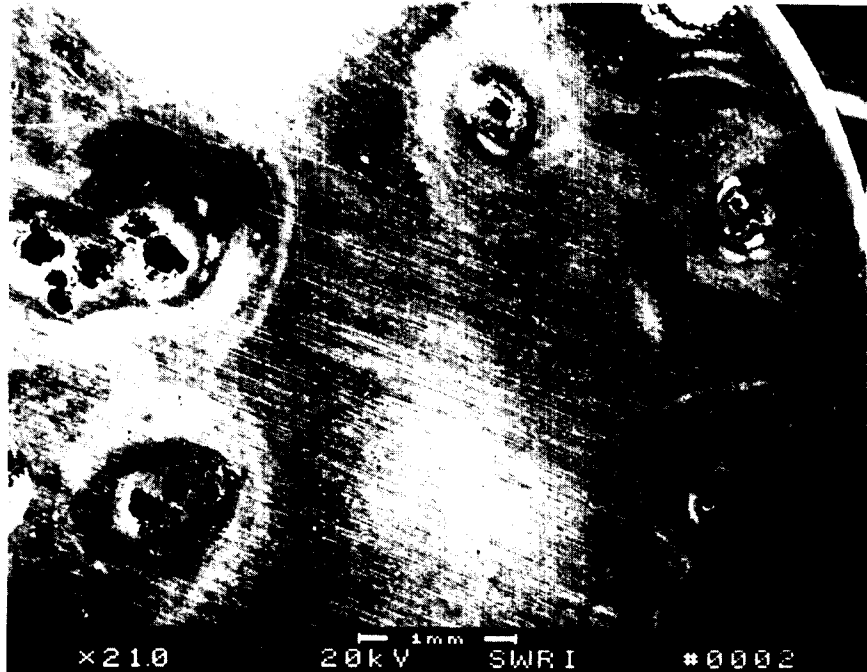
Figure 5-3a. Scanning electron microscope view of pits that were rated 4. Specimens rated 3 also pitted in a similar fashion but without crevice corrosion.
