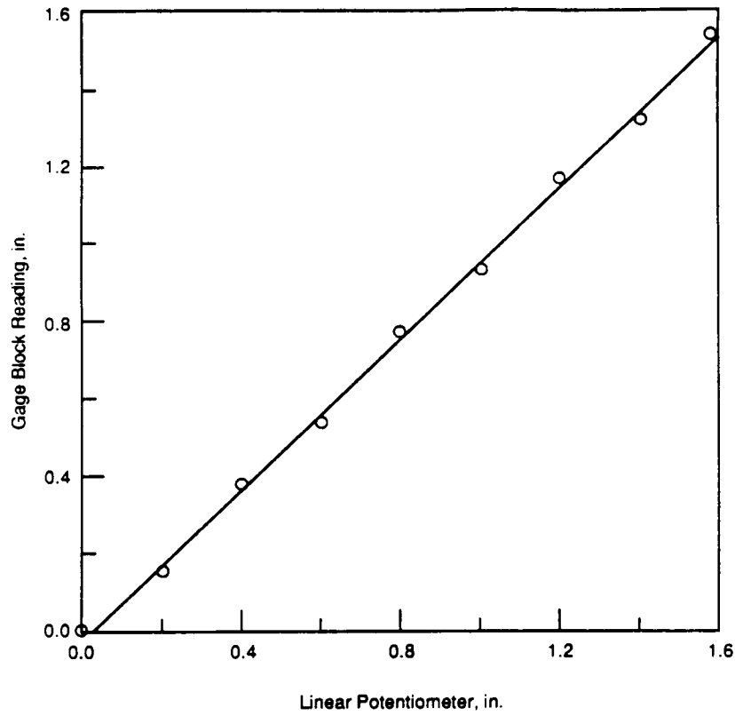
Figure 4-20. Extensometer calibration curve for MPBX No. B, position 3
