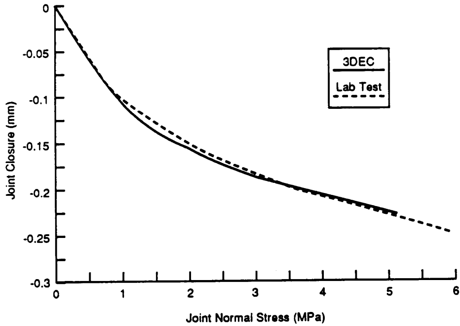
Figure 4-3. Comparison of 3DEC model to laboratory test results for joint closure variation with pseudostatic normal stress
