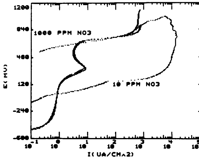
Figure 5-1. Typical cyclic polarization curves for alloy 825 at 95°C indicating the effect of nitrate at a chloride concentration of 1000 ppm
