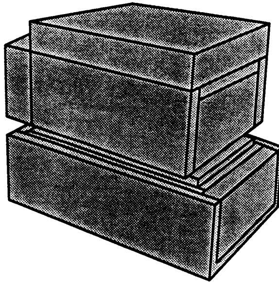
Figure 4-2. 3DEC full model consisting of a jointed tuff specimen inside the shear box
