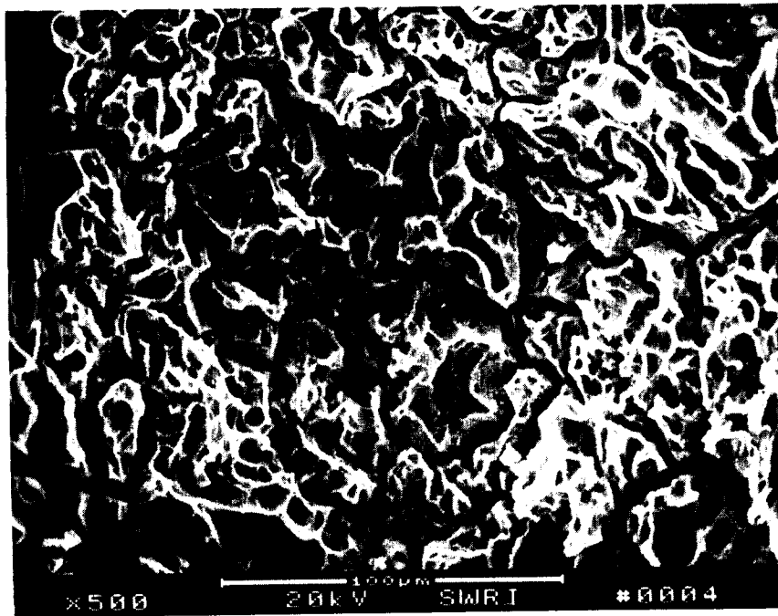
Figure 5-4b. Magnified view of the bottom of a pit shown above. Intergranular attack is evident in these pits.
