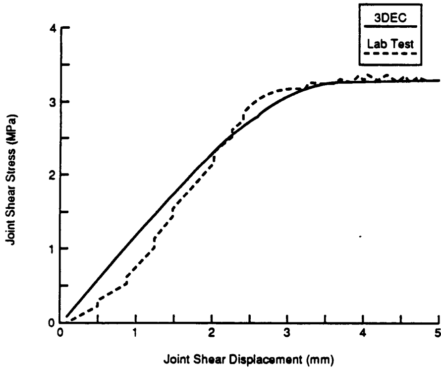
Figure 4-4. Comparison of 3DEC model to laboratory test results for joint stress variation with joint shear displacement at normal stress = 4.36 MPa
