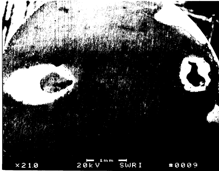
Figure 5-5a. Scanning electron microscope view of pits rated 1
