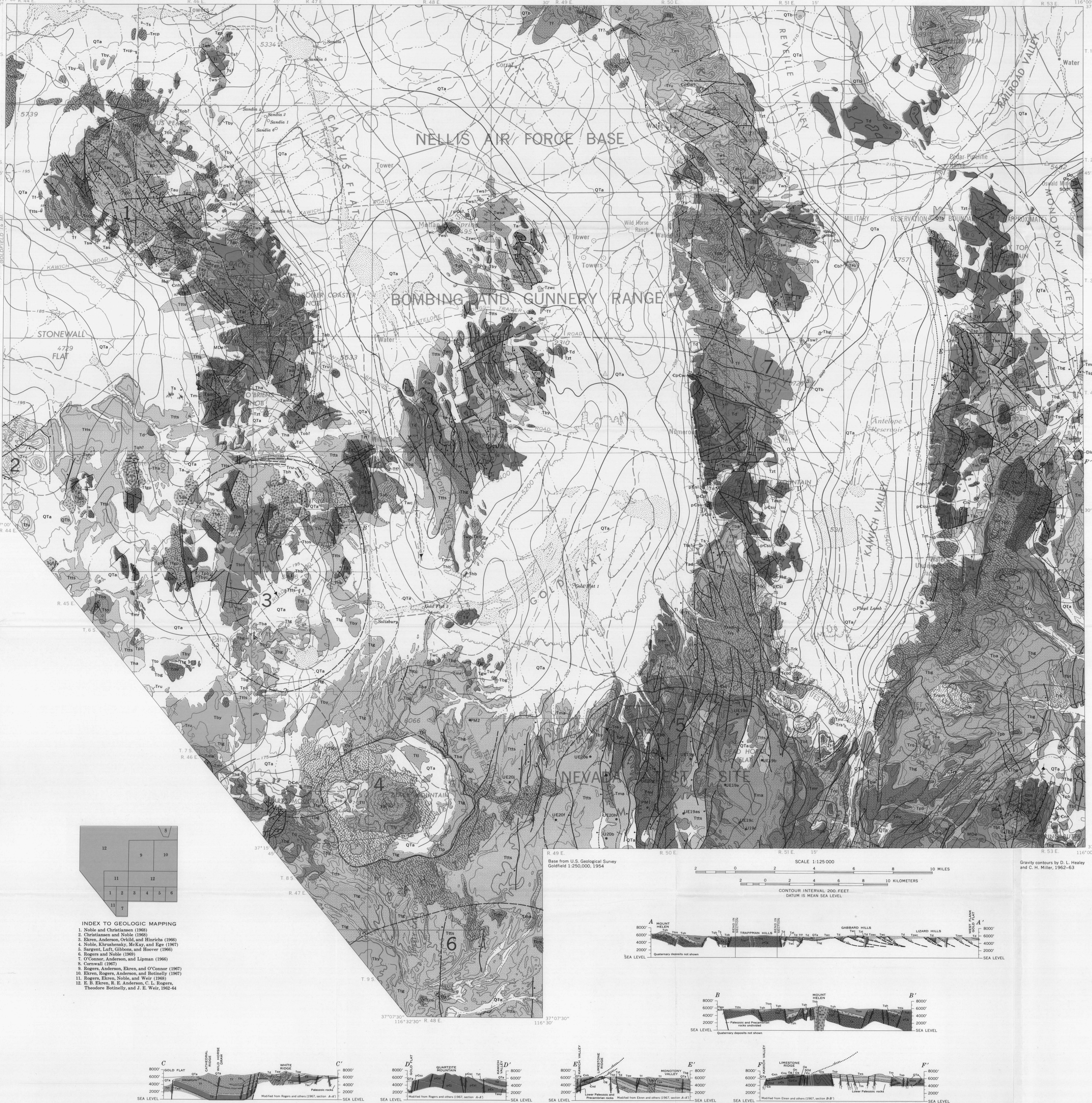
GEOLOGIC AND BOUGUER GRAVITY MAP AND SECTIONS OF NORTHERN NELLIS AIR FORCE BASE BOMBING AND GUNNERY RANGE, NYE COUNTY, NEVADA
