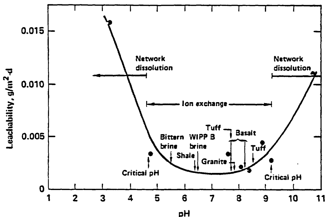
FIGURE 5-3 Effect of pH on leach rate of silicon from borosilicate glass, based on 5-day static tests at 25°C with S/V = 0.1 cm -1 . WIPP refers to the Waste Isolation Pilot Plant. Source: Plodinec et al. (1982).
