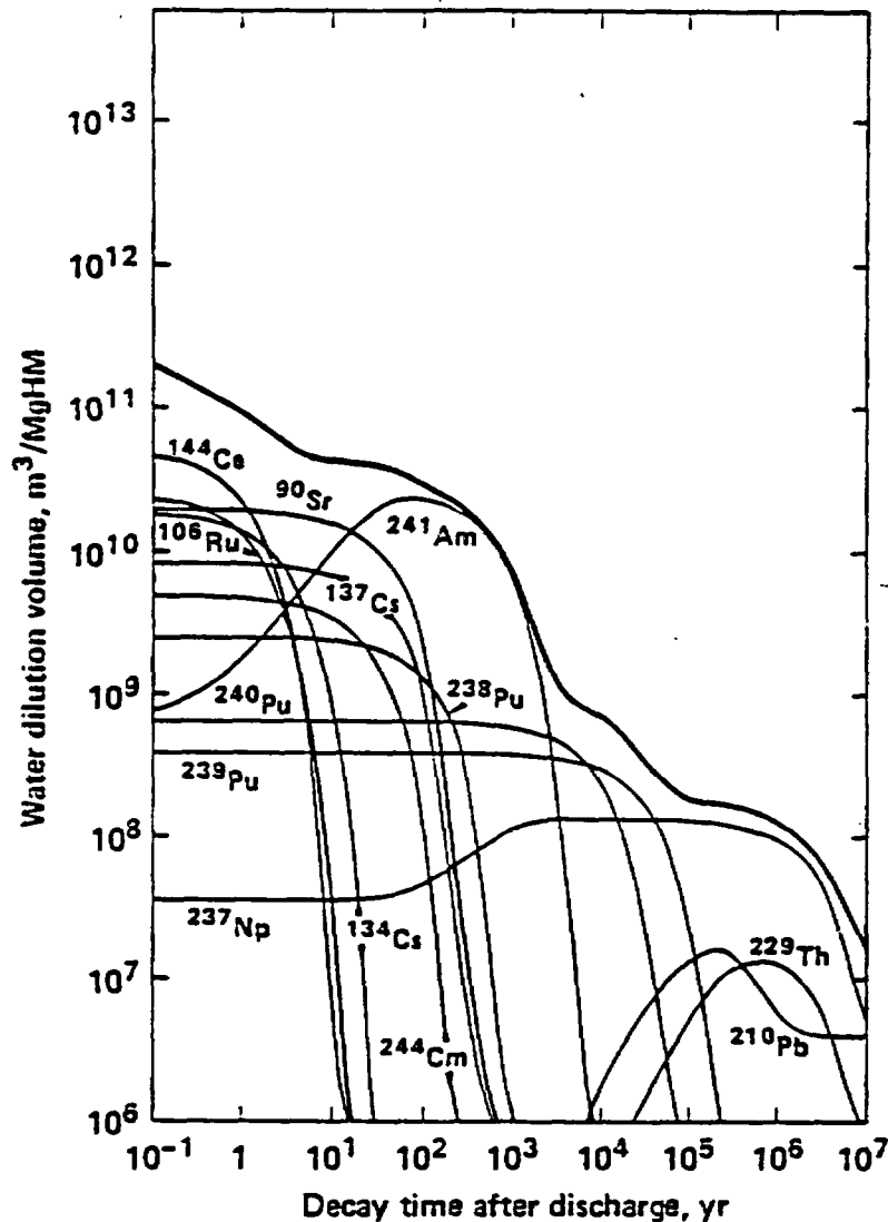
FIGURE 4-4 Water dilution volume of PWR spent fuel.
