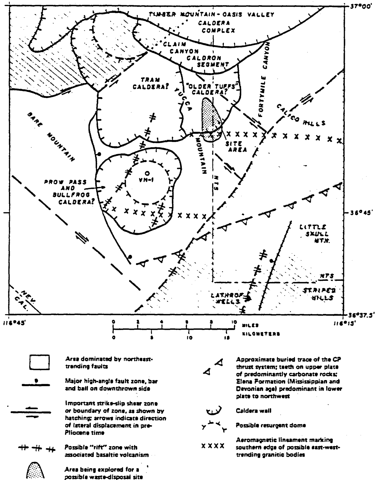
FIGURE 7-6 Diagram of the Yucca Mountain region, showing known and inferred volcanic calderas, major thrust and strike-slip faults, and basalt rift zones. Source: Carr (1982).
