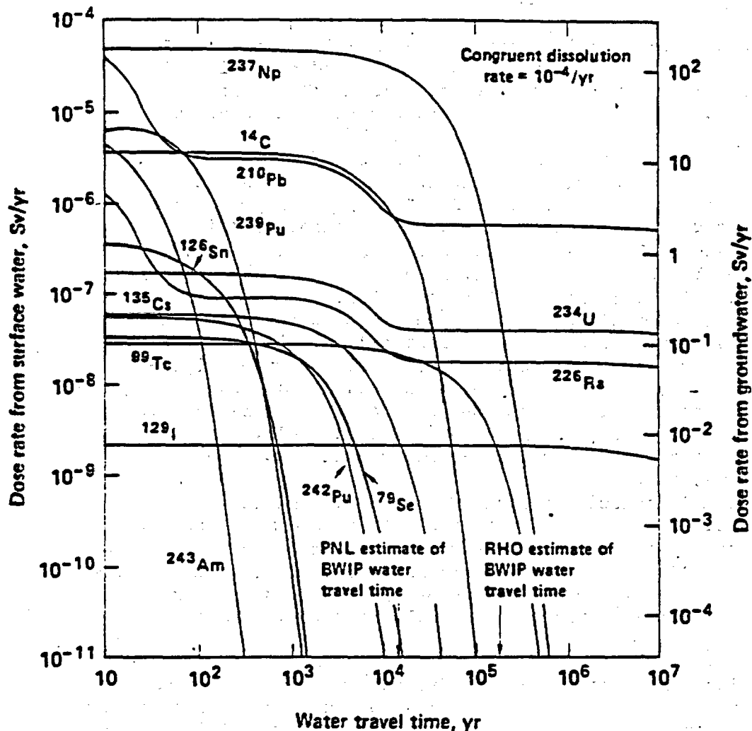
FIGURE 9-13 Individual radiation dose as a function of water travel time in basalt: unprocessed spent fuel from 10 5 Mg uranium fuel, congruent dissolution, no dispersion.
