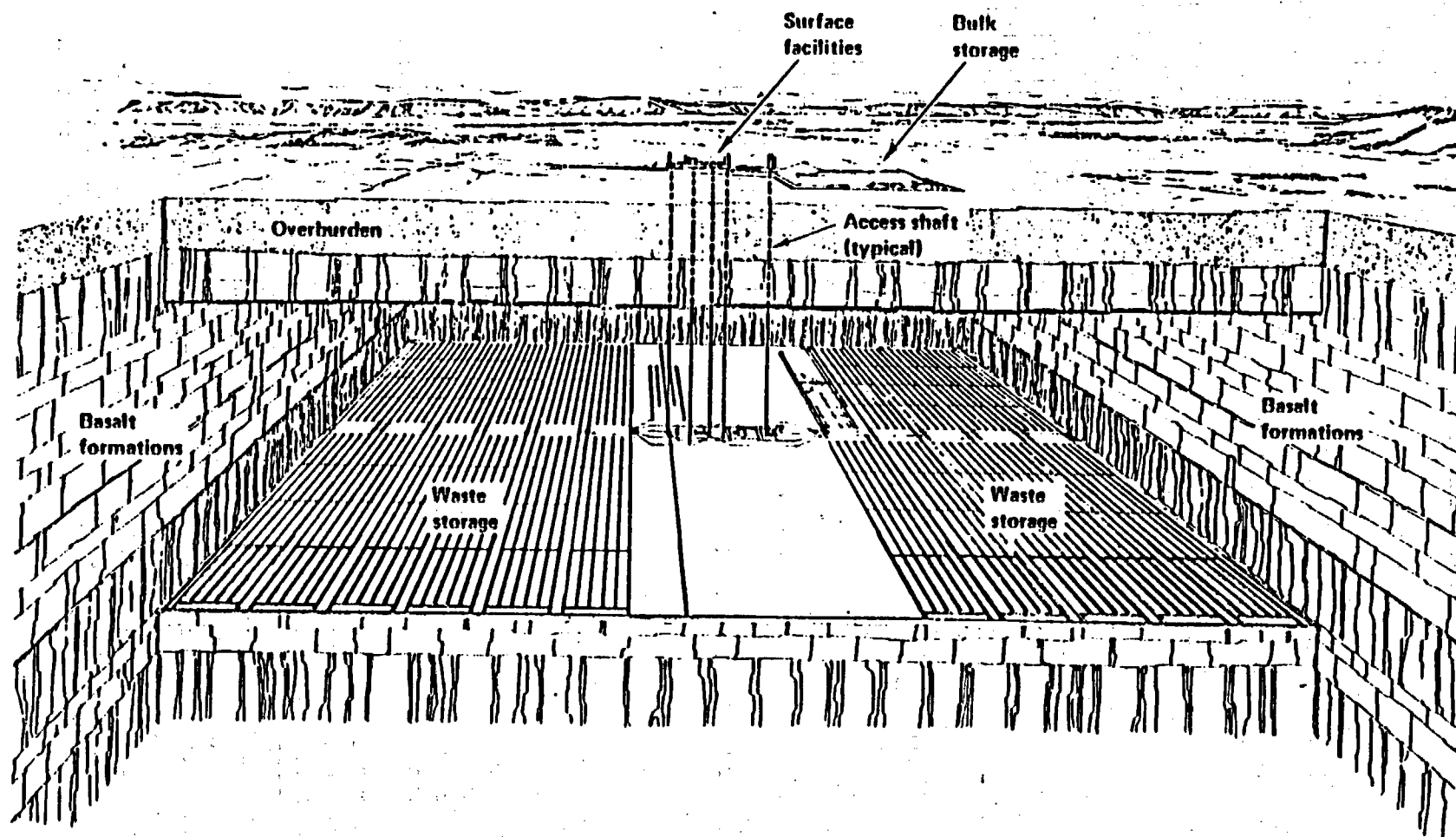
FIGURE 6-1 Cutaway perspective of a conceptual repository in basalt. Source: Schmidt (1981).
