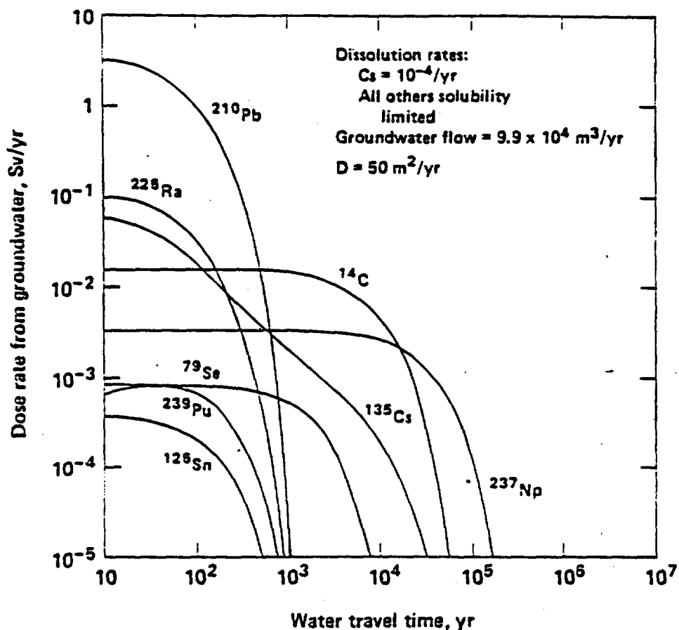
FIGURE 9-12 Individual radiation dose as a function of water travel time in tuff: reprocessing waste from 10^5 Mg uranium fuel, solubility-limited dissolution.
