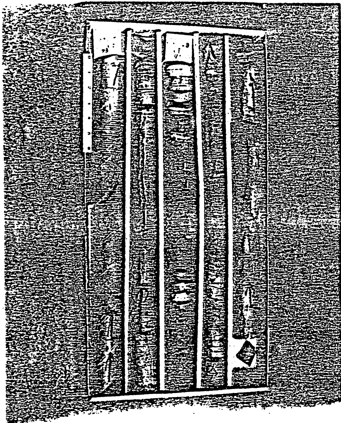
FIGURE 6-7 Basalt core from Hanford—moderate discing. Source: Courtesy of Rockwell International.
