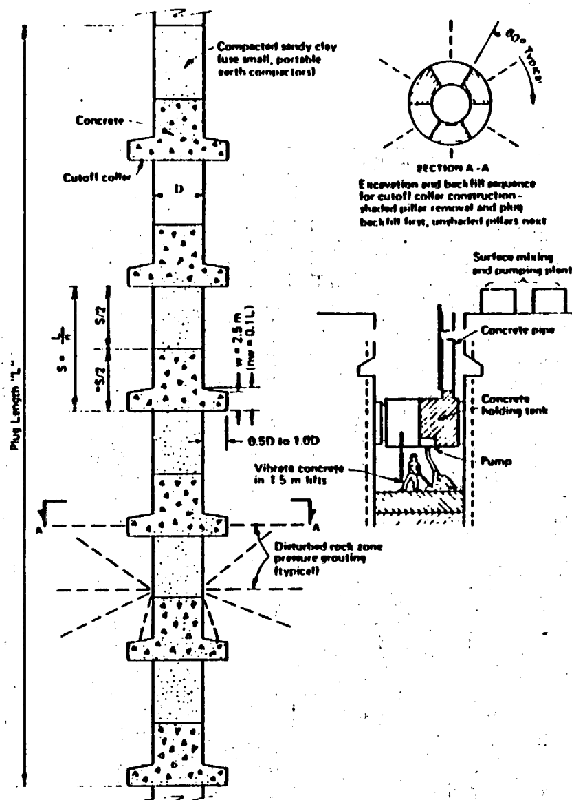
FIGURE 6-11 Preconceptual design of shaft plugs in basalt. Source: Basalt Waste Isolation Project Staff (1981a).
