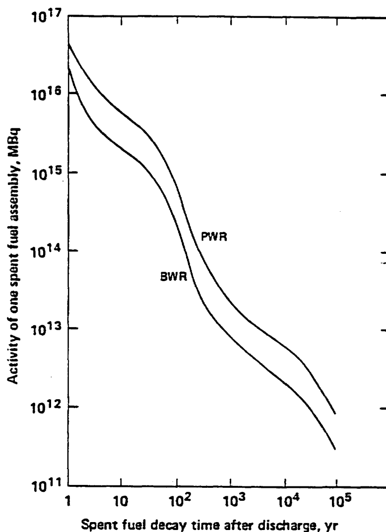
FIGURE 4-3 Activities of spent BWR and PWR fuel assemblies.
