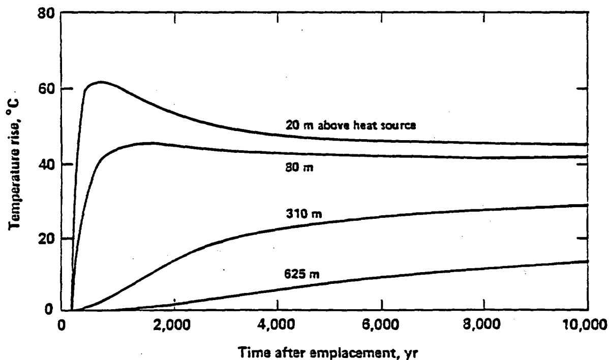
FIGURE 6-13 Far-field temperature effects for an areal thermal load of 12.3 W/m² in basalt. Source: Reference Repository Conditions Interface Working Groups (1981b).
