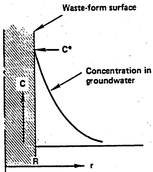
FIGURE 5-5 Velocity and concentration profiles for groundwater flowing across a waste cylinder.
