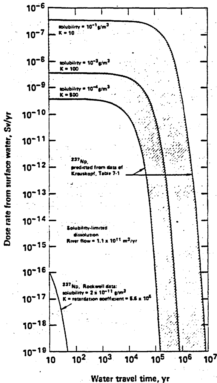
FIGURE 9-17 Individual radiation dose from neptunium-237 as a function of water travel time in basalt, showing the effect of Rockwell data on solubility and retardation: reprocessing waste from 10^4 Mg uranium fuel, solubility-limited dissolution.
