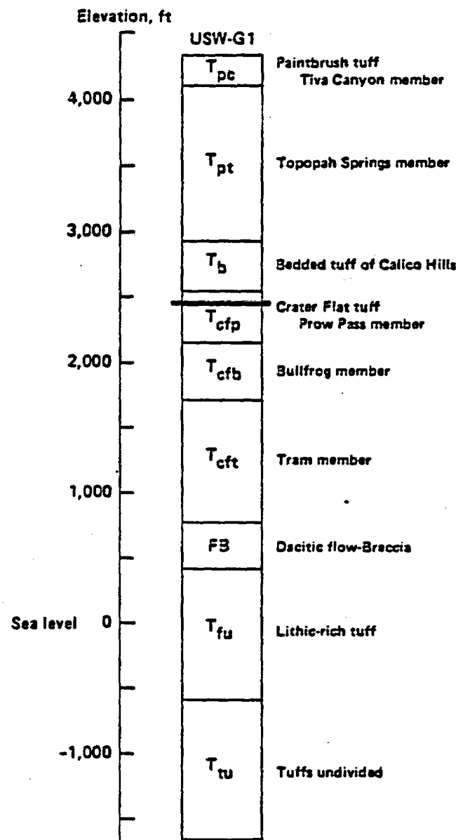
FIGURE 7-10 Stratigraphic column from drill hole USW-G1 in Yucca Mountain. The heavy black line is the static water level in this hole. Source: Bish (1981).
