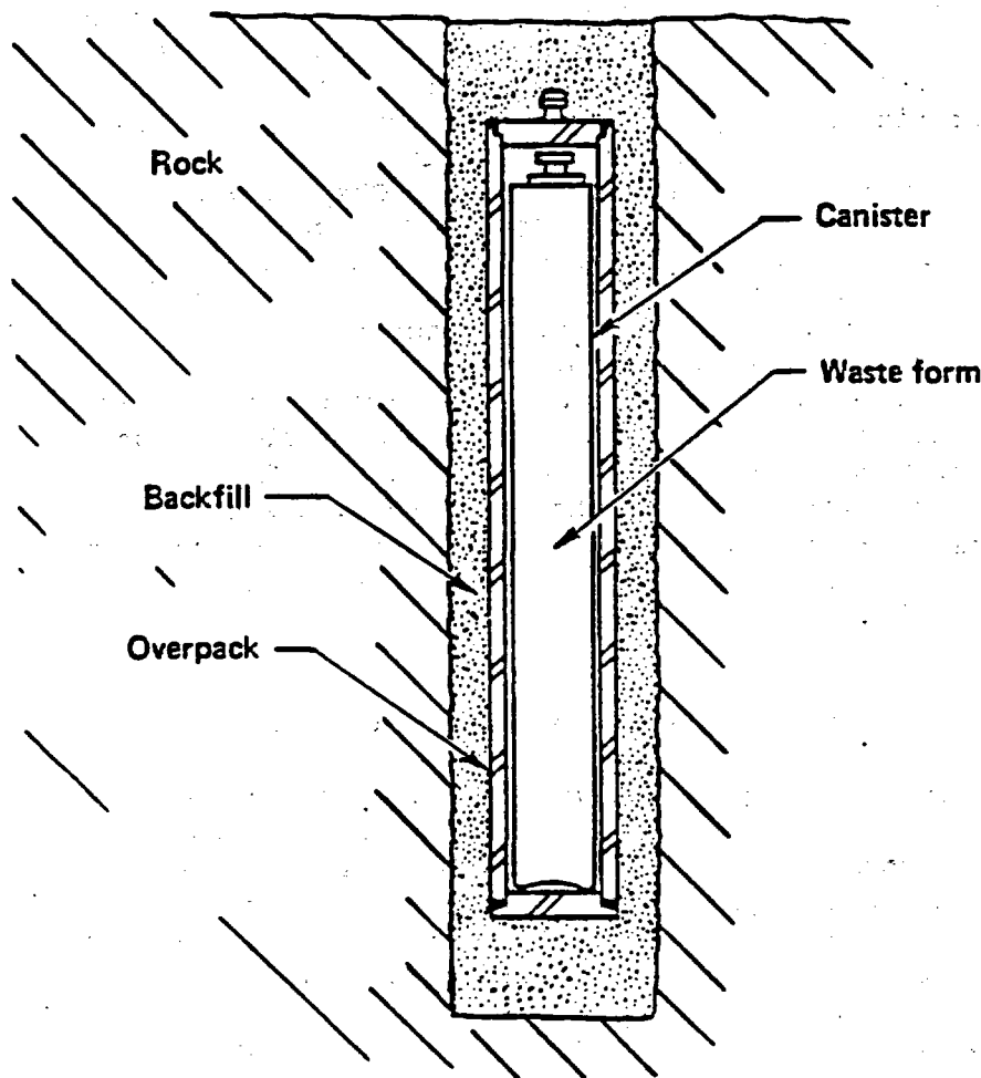
FIGURE 5-1 Waste package schematic.
