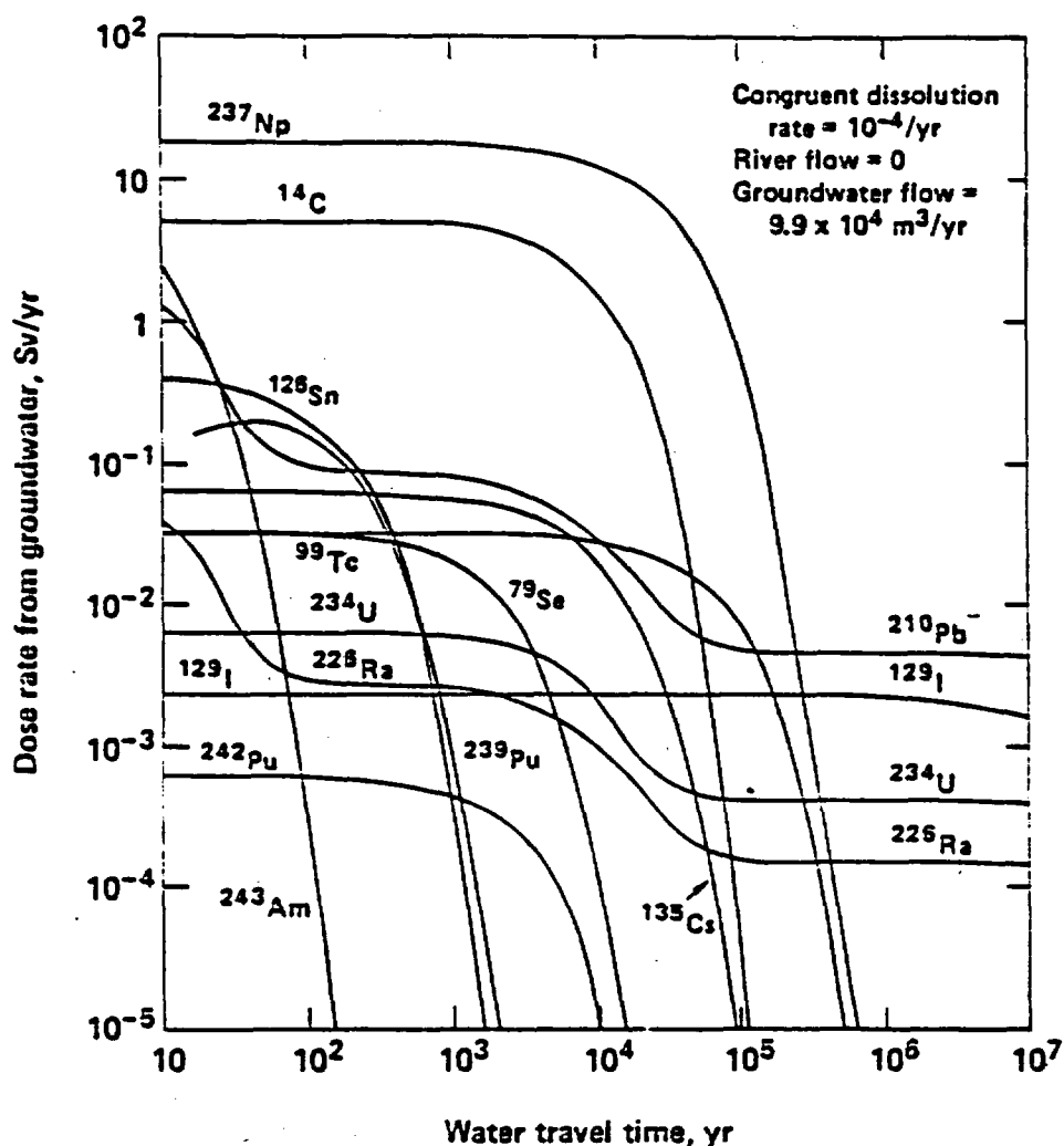
FIGURE 9-6 Individual radiation dose as a function of water travel time in tuff: reprocessing waste from 10^5 Mg uranium fuel, congruent dissolution, no dispersion.
