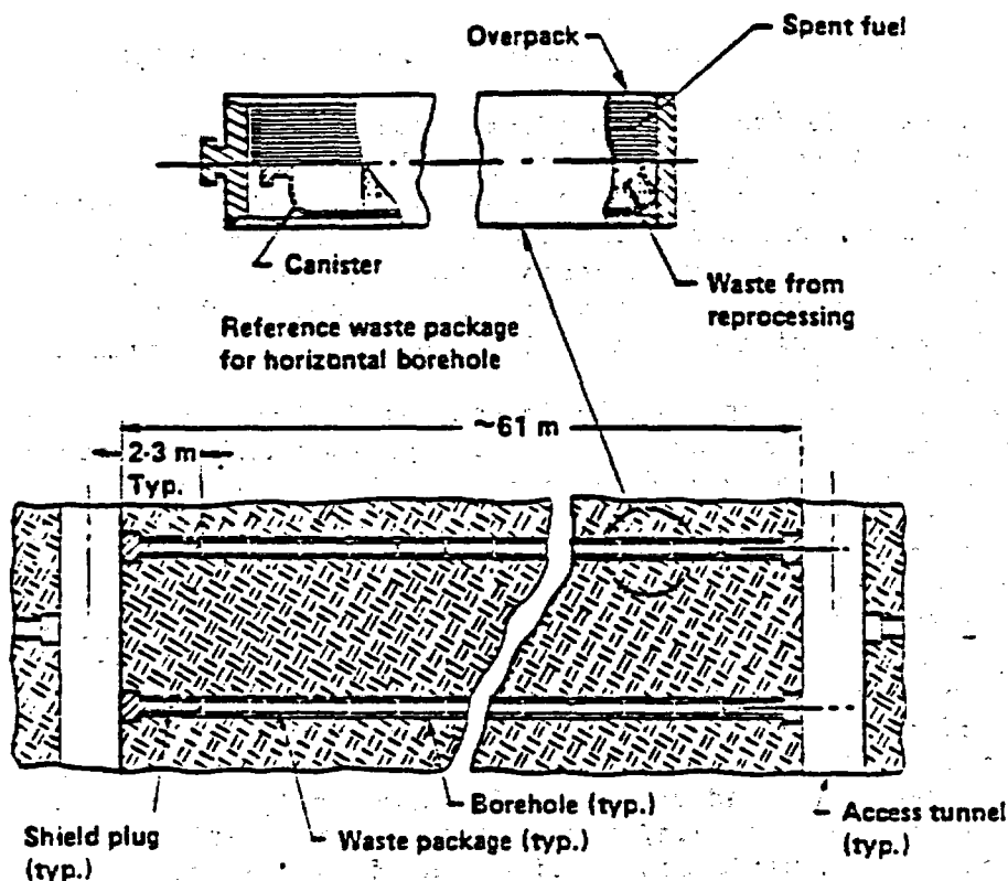
FIGURE 5-8 Borehole type package for horizontal emplacement in basalt. Source: Westinghouse (1982a).
