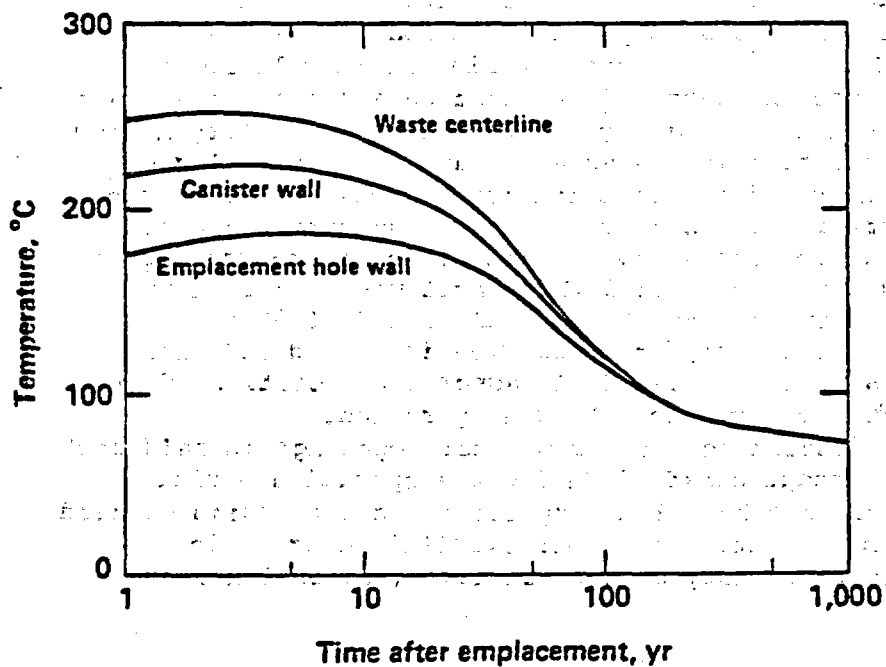
FIGURE 6-15 Alternate commercial high-level waste repository maximum temperatures in basalt. Source: Reference Repository Conditions Interface Working Groups (1981b).
