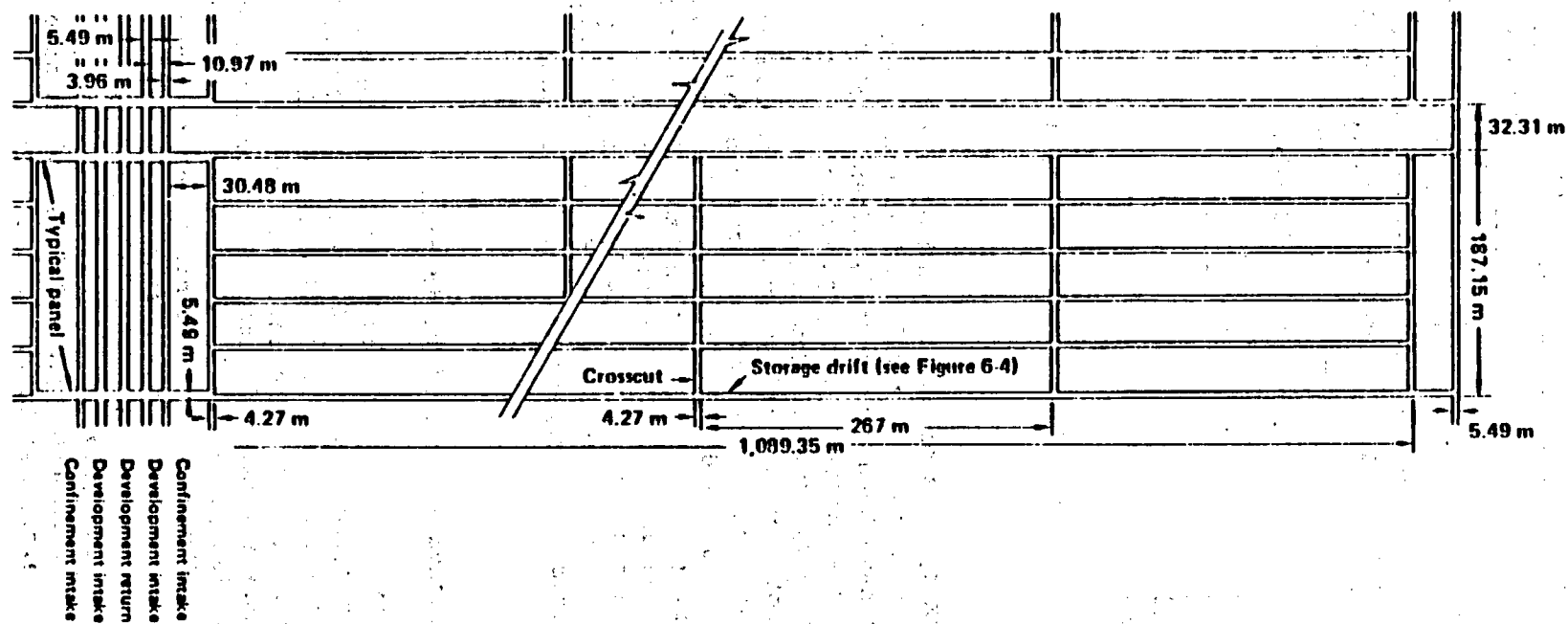
FIGURE 6-3 Typical storage panel in a conceptual design for a repository in basalt. Source: Schmidt (1981).
