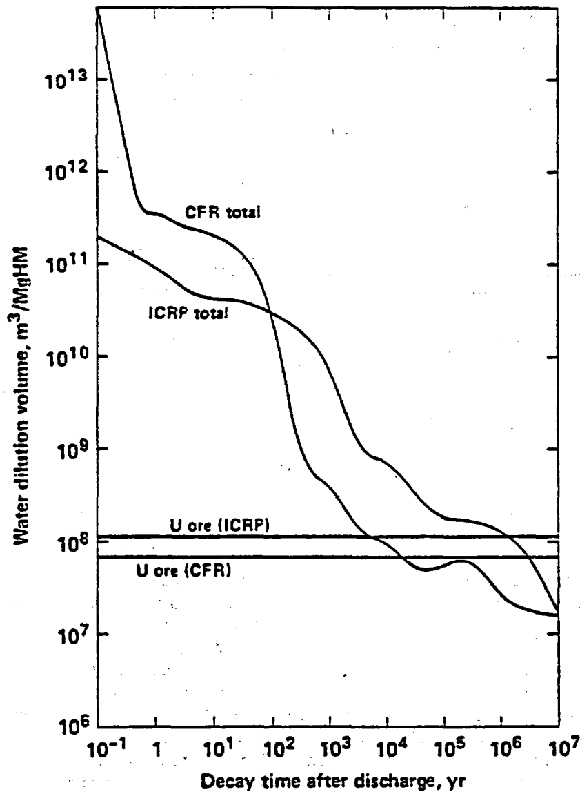
FIGURE 4-5 Water dilution volumes of PWR spent fuel and its parent uranium ore.
