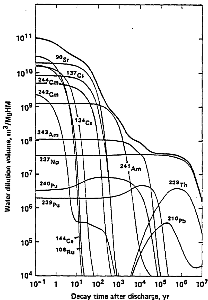
FIGURE 4-6 Water dilution volume of PWR high-level waste.
