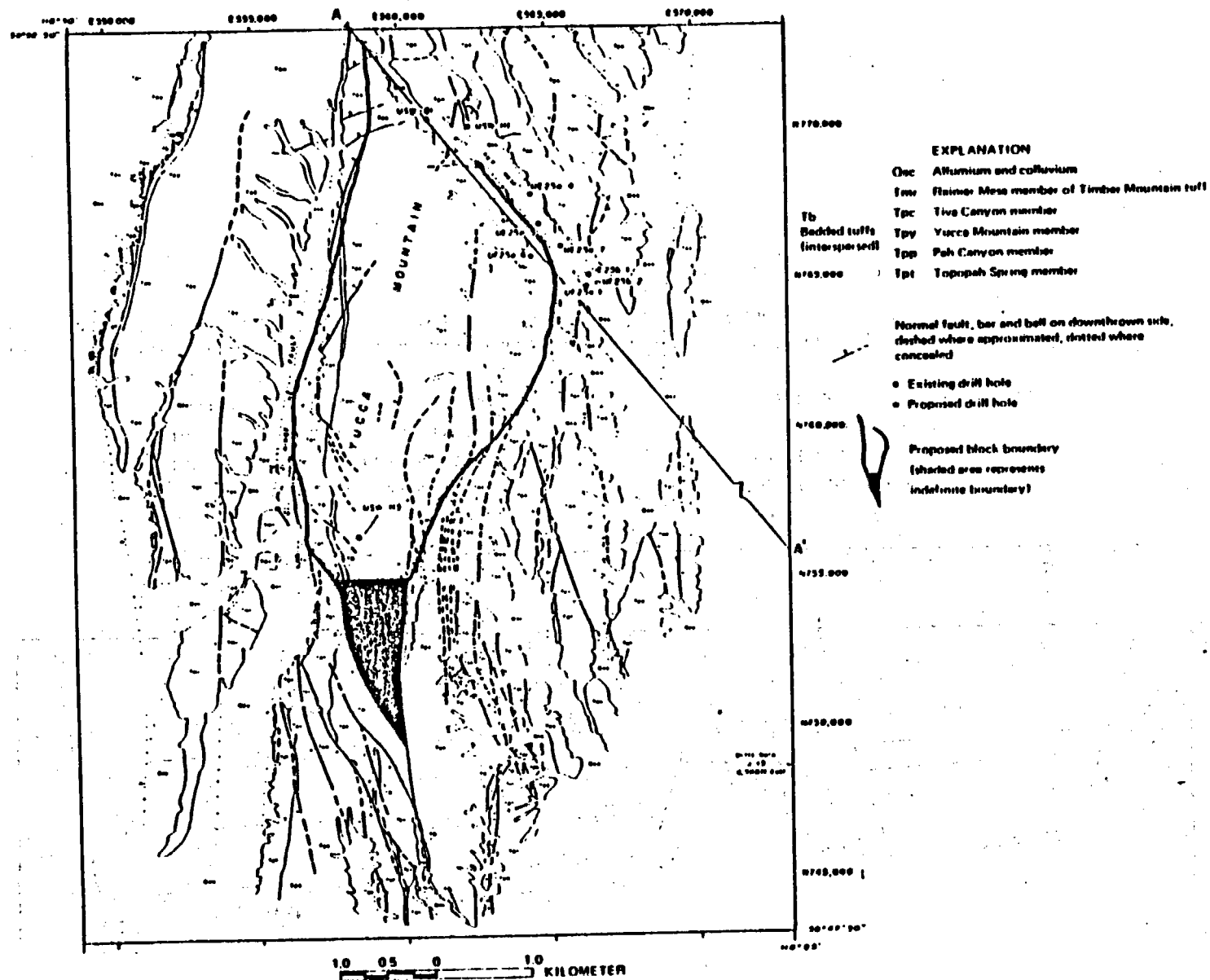
FIGURE 7-7 Generalized geologic map of Yucca Mountains. Source: Courtesy of G. Dixon, U.S. Geological Survey.
