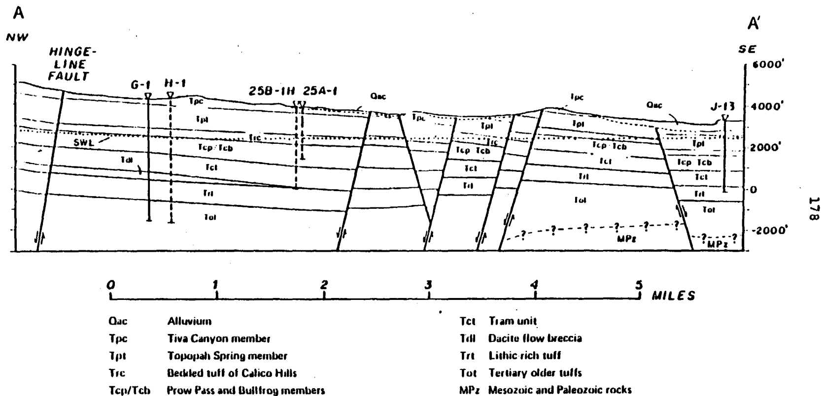
FIGURE 7-8 Cross-section through northern part of Yucca Mountain (section A-A' in Figure 7-7), west-central part of Nevada Test Site, Nevada. Dotted line labelled SWL is static water level. Source: Courtesy of G. Dixon, U.S. Geological Survey.
