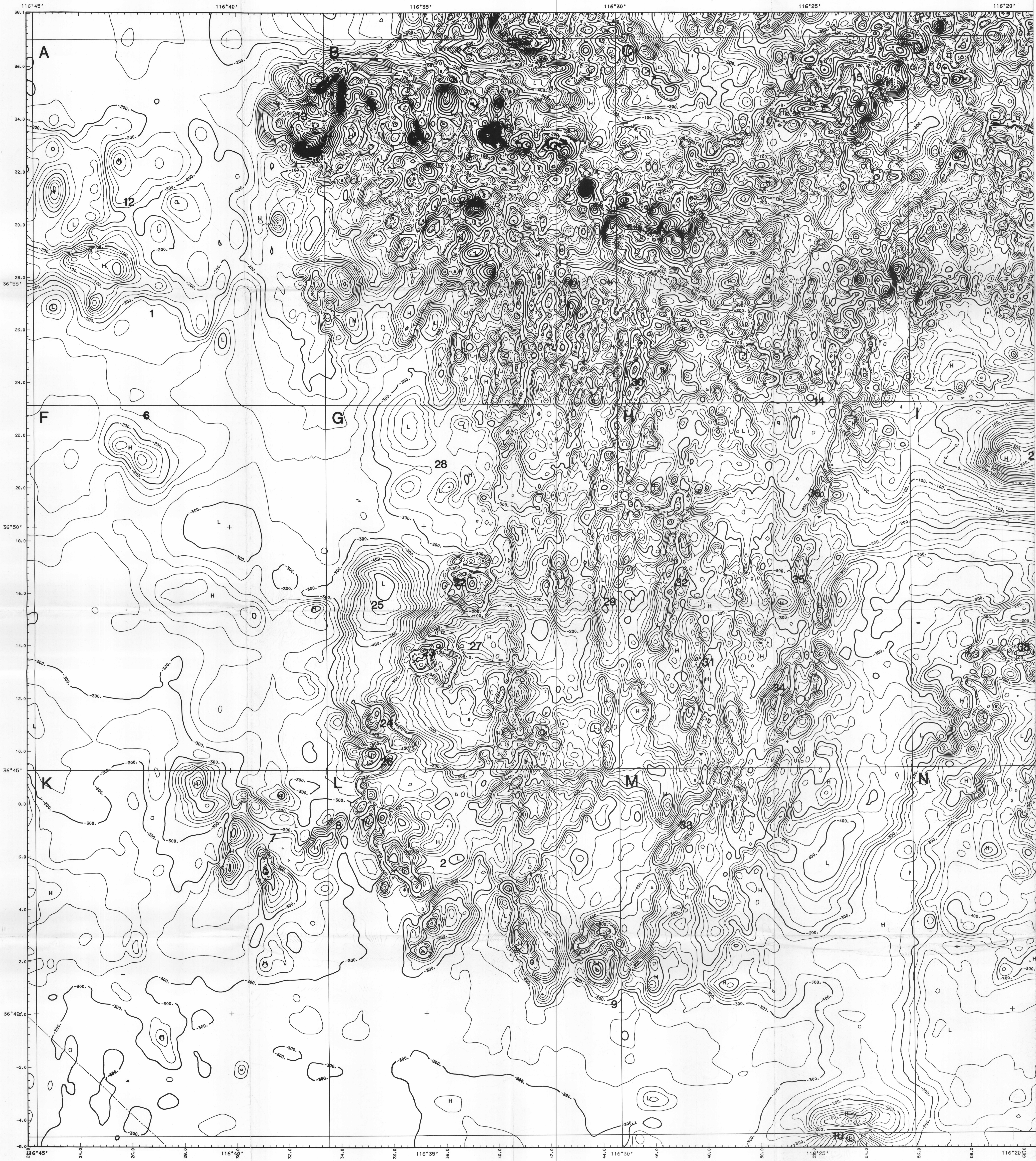
PLATE 1 - AEROMAGNETIC MAP OF YUCCA MOUNTAIN AND SURROUNDING REGIONS
