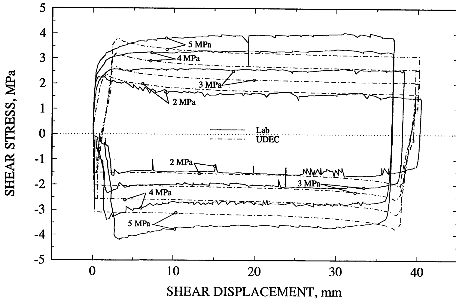
Figure 5-15. UDEC using Barton-Bandis joint model and laboratory test results of shear stress versus shear displacement plot for the same specimen as a function of normal stress for test no. 10
