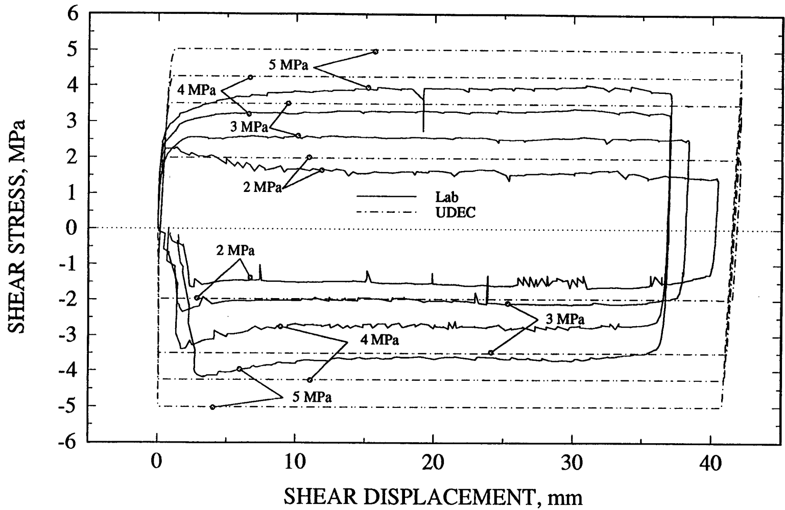
Figure 5-4. UDEC using Mohr-Coulomb joint model and laboratory test results of shear stress versus shear displacement plot for the same joint specimen as a function of normal stress for test no. 10
