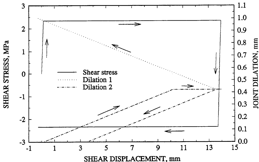
Figure 3-3. Prediction of joint behavior using the Mohr-Coulomb model assuming that shear stiffness = 16.93 GPa, friction angle = 38°, dilation angle = 2.4°, and normal stress = 3 MPa (assuming that the critical shear displacement has been reached)
