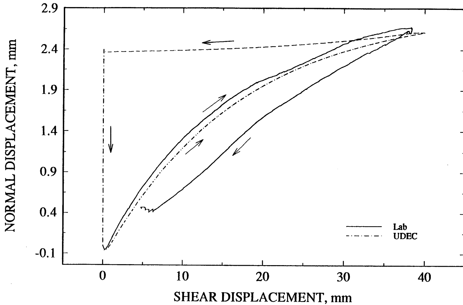
Figure 5-27. UDEC results using Continuously-Yielding joint model and laboratory measurements of joint dilation plot for test no. 7 under normal stress of 5 MPa
