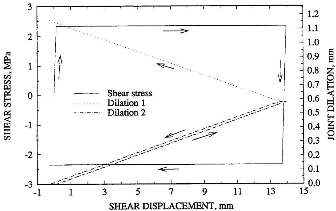
Figure 3-2. Prediction of joint behavior using the Mohr-Coulomb model assuming that shear stiffness = 16.93 GPa, friction angle = 38°, dilation angle = 2.4°, and normal stress = 3 MPa (assuming that the critical shear displacement is not reached)
