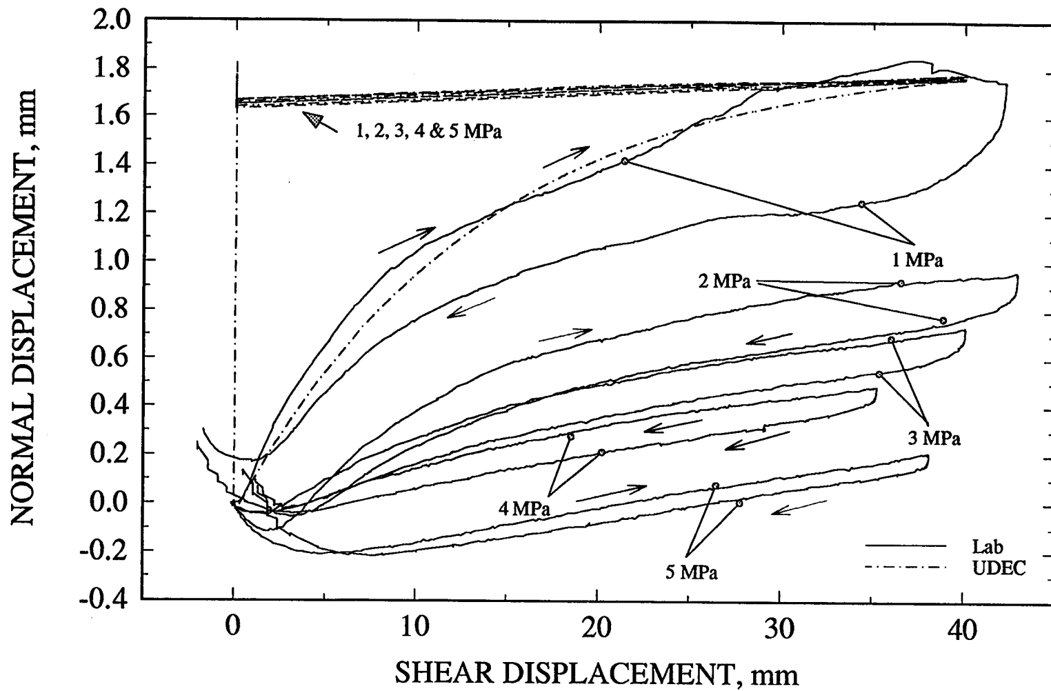
Figure 5-31. UDEC results using Continuously-Yielding joint model and laboratory measurements of joint dilation plot for the same joint specimen as a function of normal stress for test no. 11
