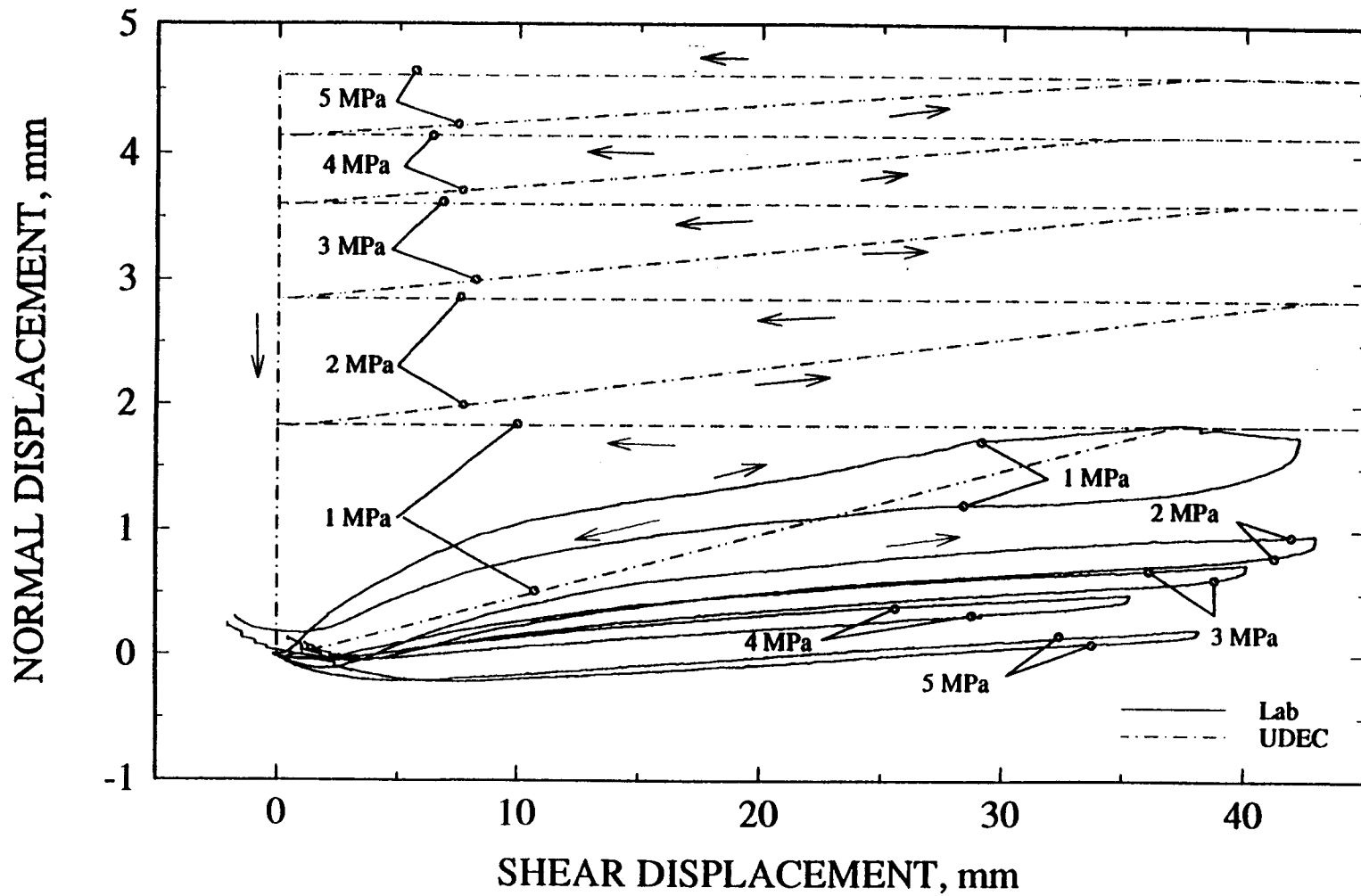
Figure 5-10. UDEC results using Mohr-Coulomb joint model and laboratory measurements of joint dilation plot for the same joint specimen as a function of normal stress for test no. 11
