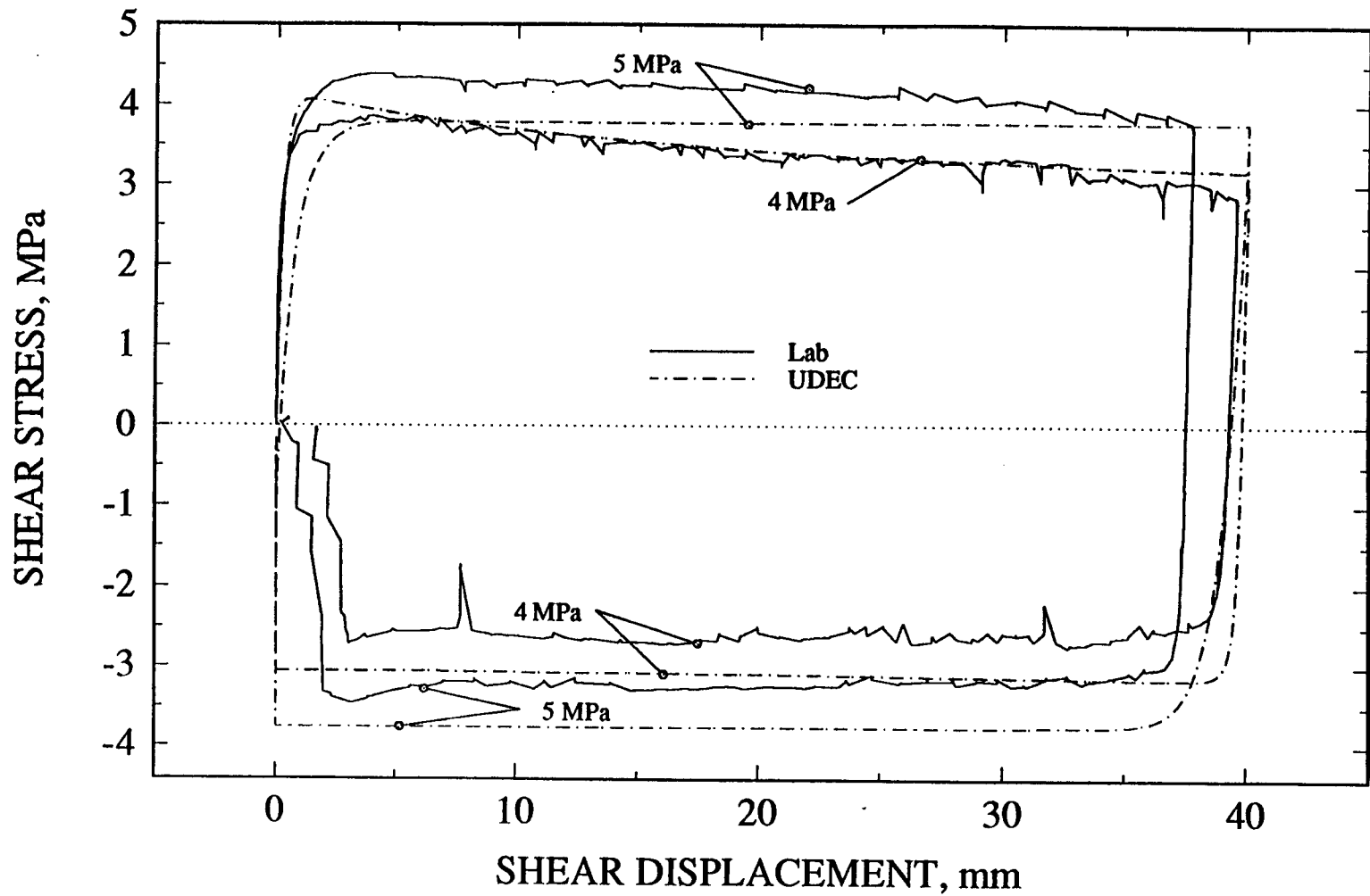
Figure 5-23. UDEC using Continuously-Yielding joint model and laboratory test results of shear stress versus shear displacement plot for the same specimen as a function of normal stress for test no. 8
