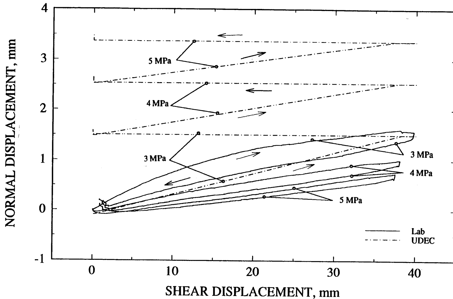
Figure 5-8. UDEC results using Mohr-Coulomb joint model and laboratory measurements of joint dilation plot for the same joint specimen as a function of normal stress for test no. 9
