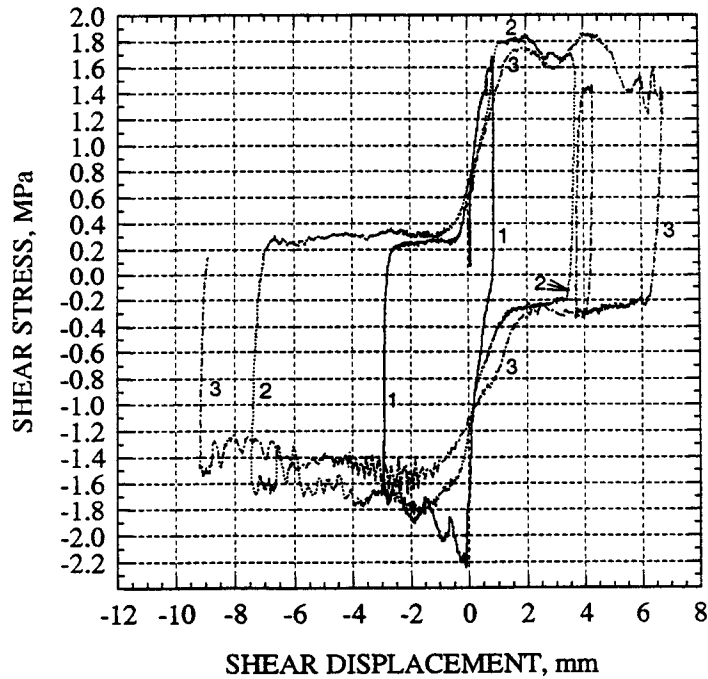
Figure 2-4. Shear stress versus shear displacement curve of a joint under an earthquake load with a maximum input displacement amplitude of 25.4 mm (load cycle numbers are indicated in the figure)
