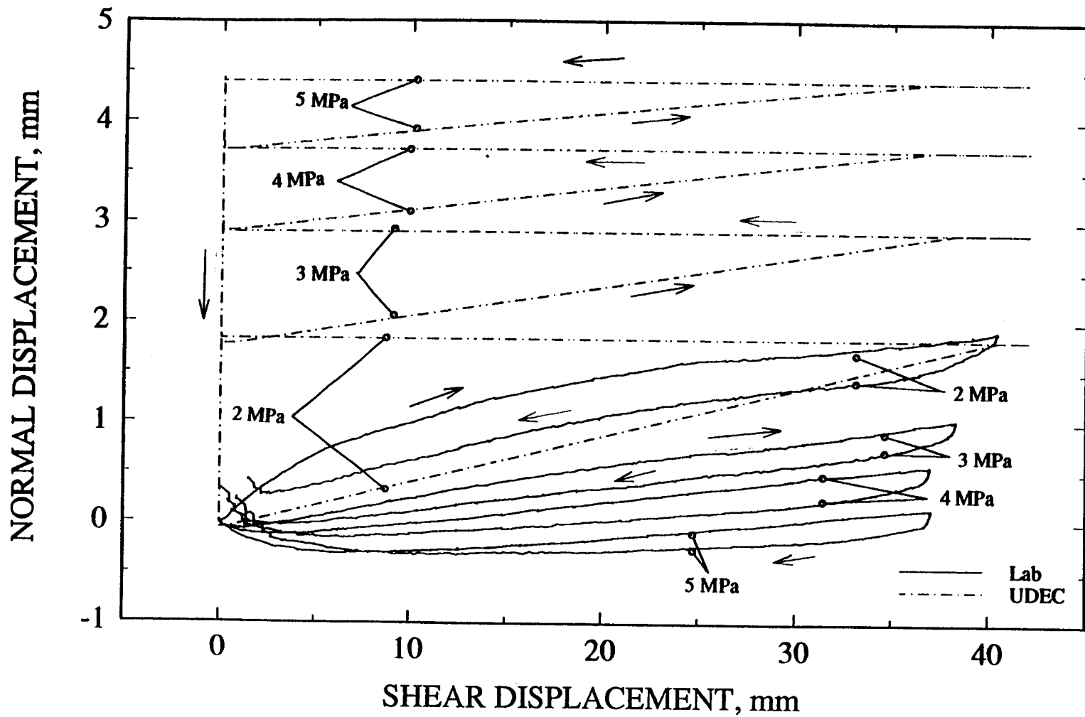
Figure 5-9. UDEC results using Mohr-Coulomb joint model and laboratory measurements of joint dilation plot for the same joint specimen as a function of normal stress for test no. 10
