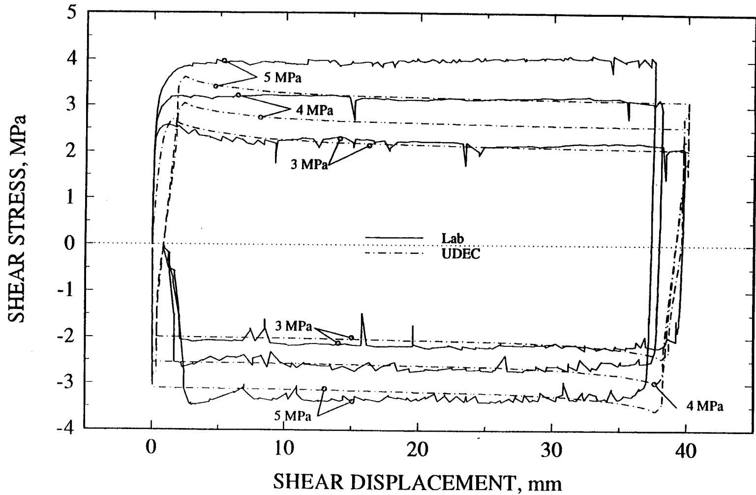
Figure 5-14. UDEC using Barton-Bandis joint model and laboratory test results of shear stress versus shear displacement plot for the same specimen as a function of normal stress for test no. 9
