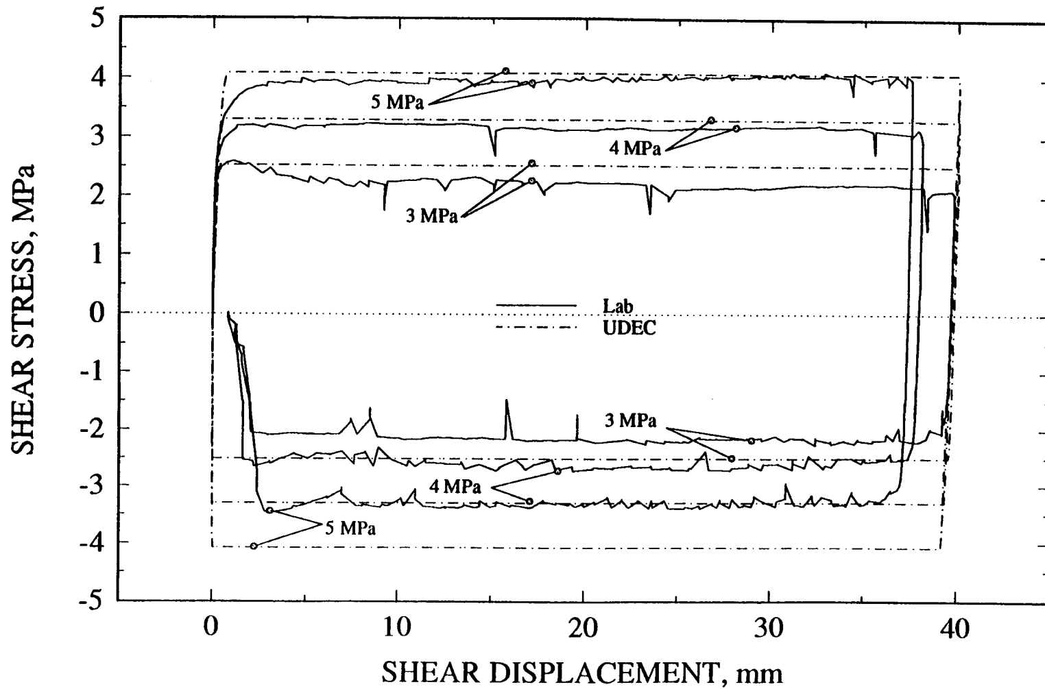
Figure 5-3. UDEC using Mohr-Coulomb joint model and laboratory test results of shear stress versus shear displacement plot for the same joint specimen as a function of normal stress for test no. 9
