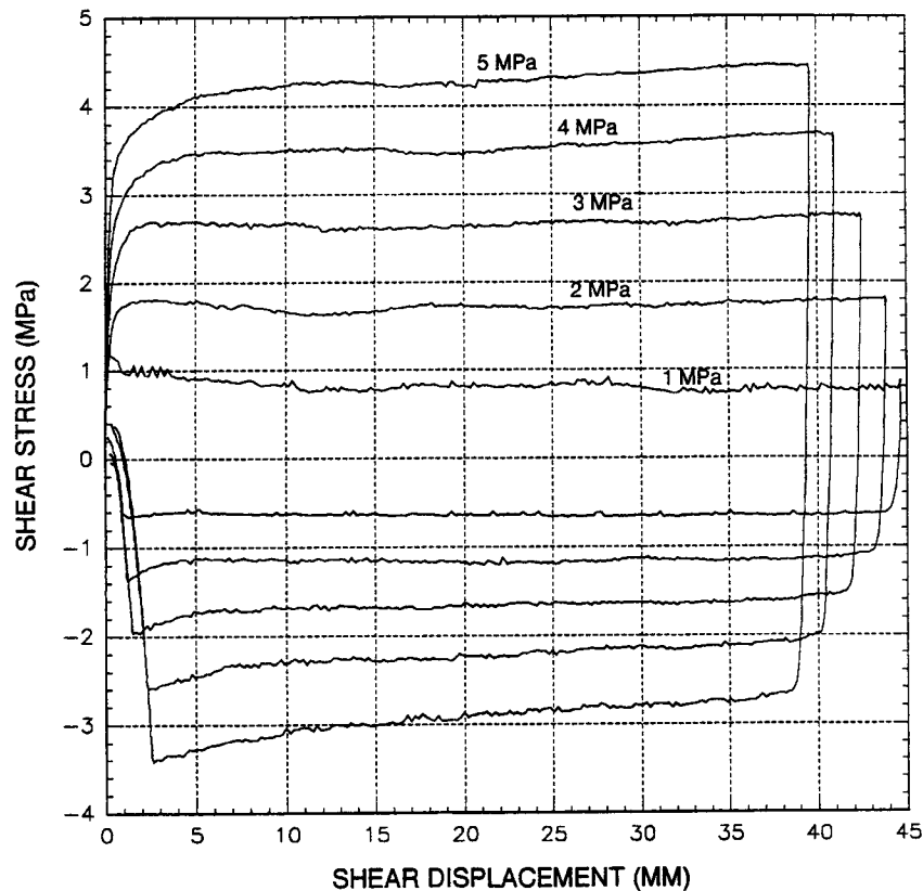
Figure 2-1. Shear stress response of test no. 17 specimen under pseudostatic cyclic loading condition as a function of normal stress
