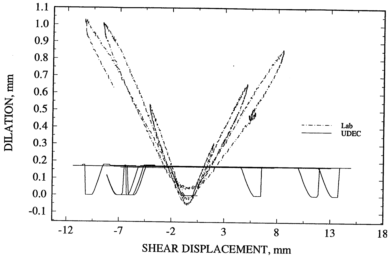
Figure 5-43. Laboratory results and UDEC prediction using Barton-Bandis joint model of joint dilation subjected to an earthquake load
