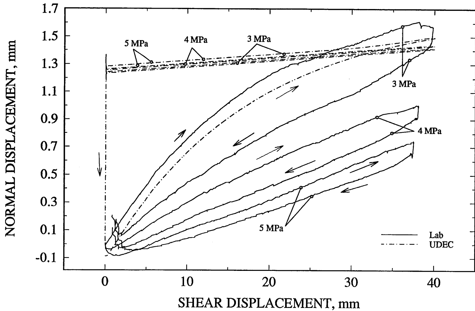
Figure 5-29. UDEC results using Continuously-Yielding joint model and laboratory measurements of joint dilation plot for the same joint specimen as a function of normal stress for test no. 9
