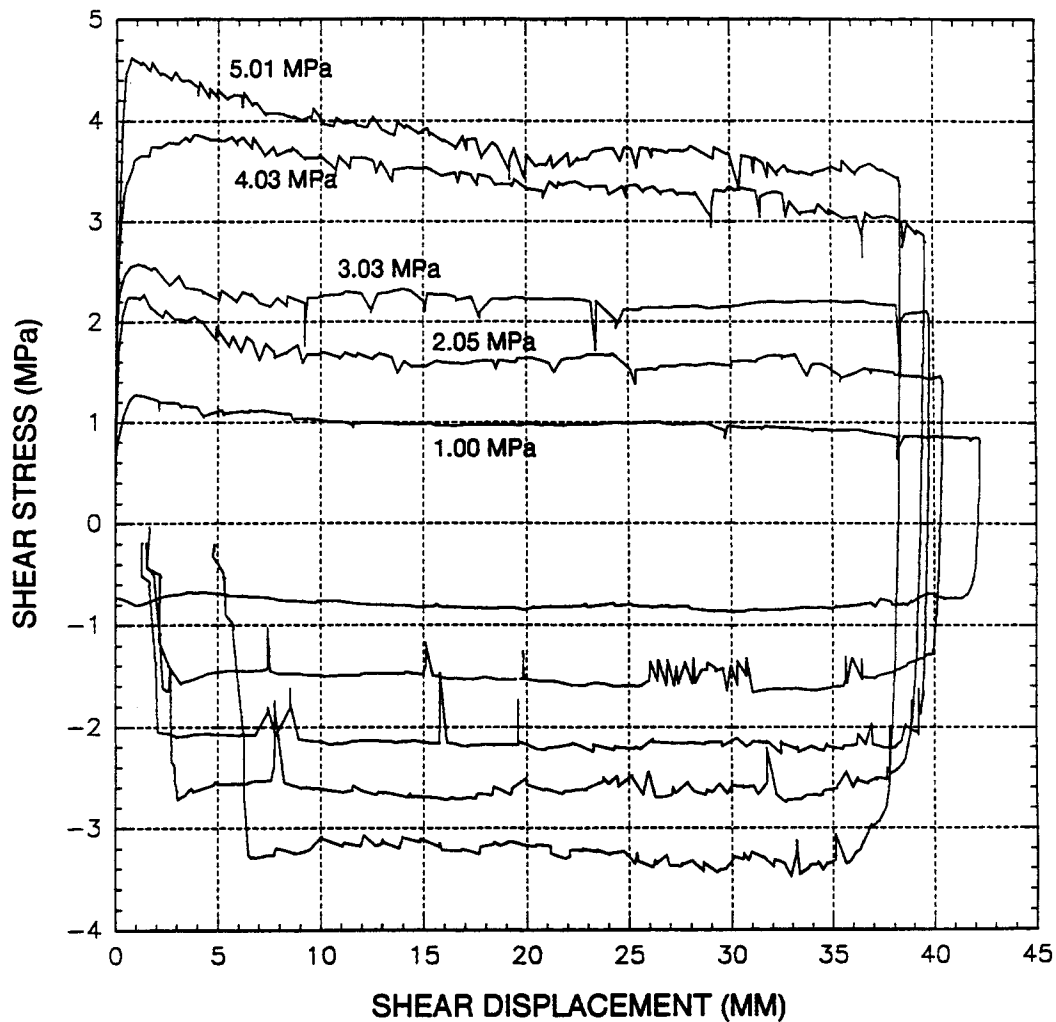
Figure 2-6. Shear stress versus shear displacement response as a function of applied normal load for various joint specimens
