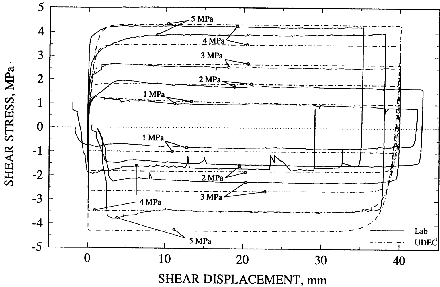
Figure 5-26. UDEC using Continuously-Yielding joint model and laboratory test results of shear stress versus shear displacement plot for the same specimen as a function of normal stress for test no. 11
