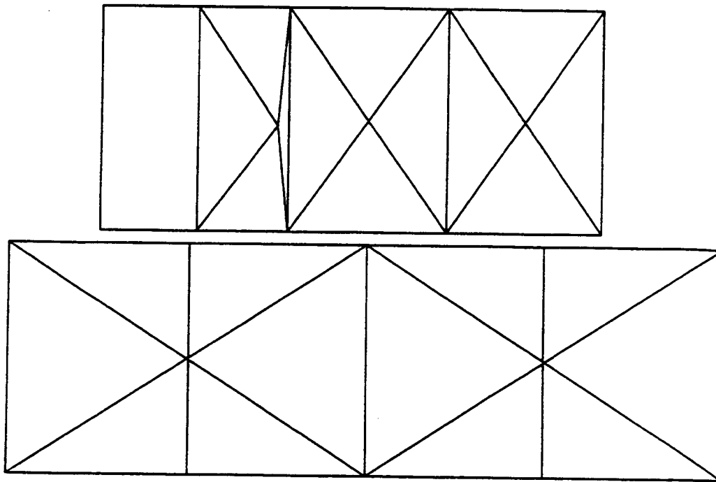
Figure 4-3. Plot showing distorted mesh of the top block due to numerical instability resulting from large number of calculations
