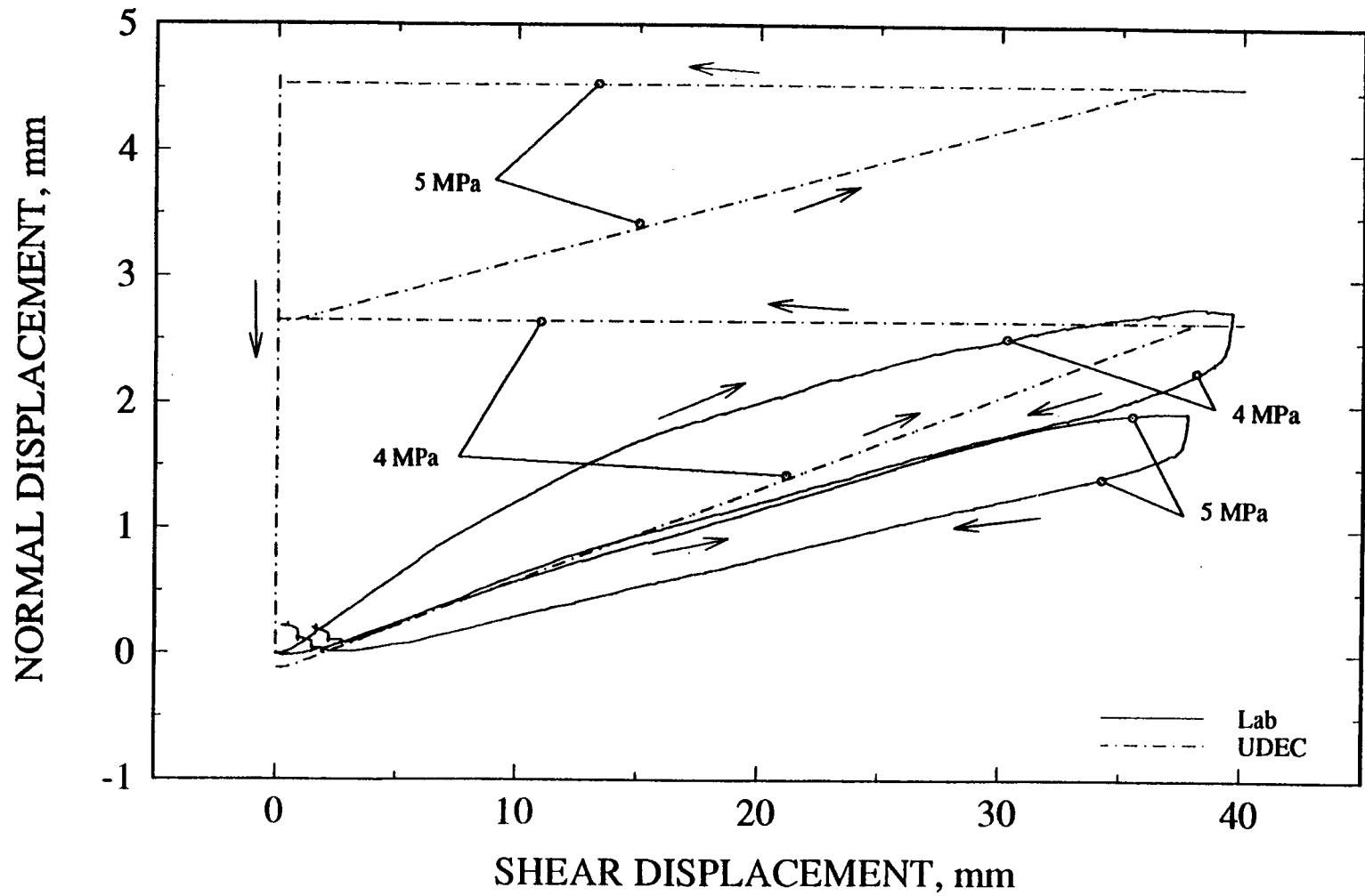
Figure 5-7. UDEC results using Mohr-Coulomb joint model and laboratory measurements of joint dilation plot for the same joint specimen as a function of normal stress for test no. 8
