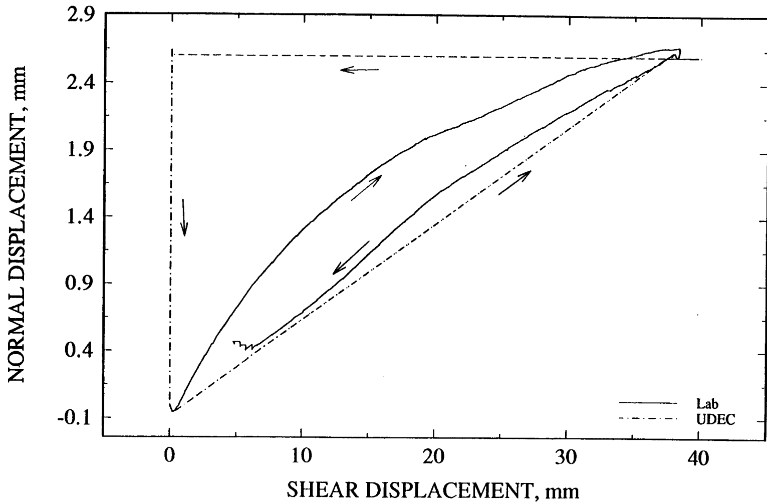
Figure 5-6. UDEC results using Mohr-Coulomb joint model and laboratory measurements of joint dilation for test no. 7 under normal stress of 5 MPa
