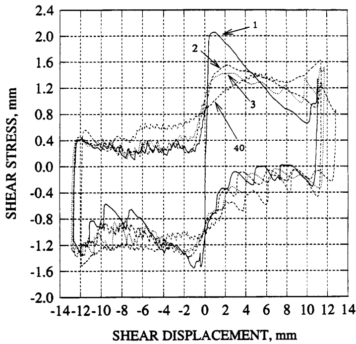
Figure 2-3. Shear stress versus shear displacement curve of a joint under a harmonic load with 1.4-Hz input frequency and 12.7-mm input displacement amplitude (load cycle numbers are indicated in the figure)
