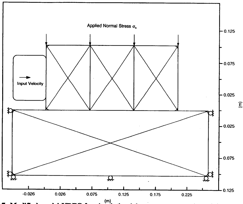
Figure 4-7. Modified model UDEC for simulating laboratory tests on single-joint specimens
