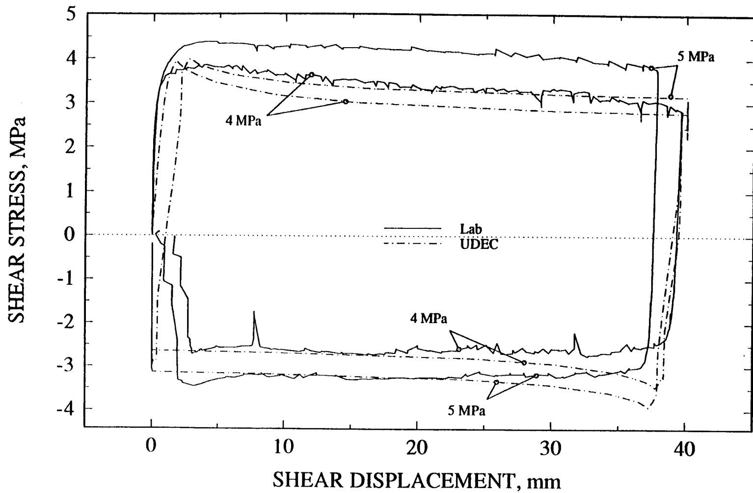
Figure 5-13. UDEC using Barton-Bandis joint model and laboratory test results of shear stress versus shear displacement plot for the same specimen as a function of normal stress for test no. 8
