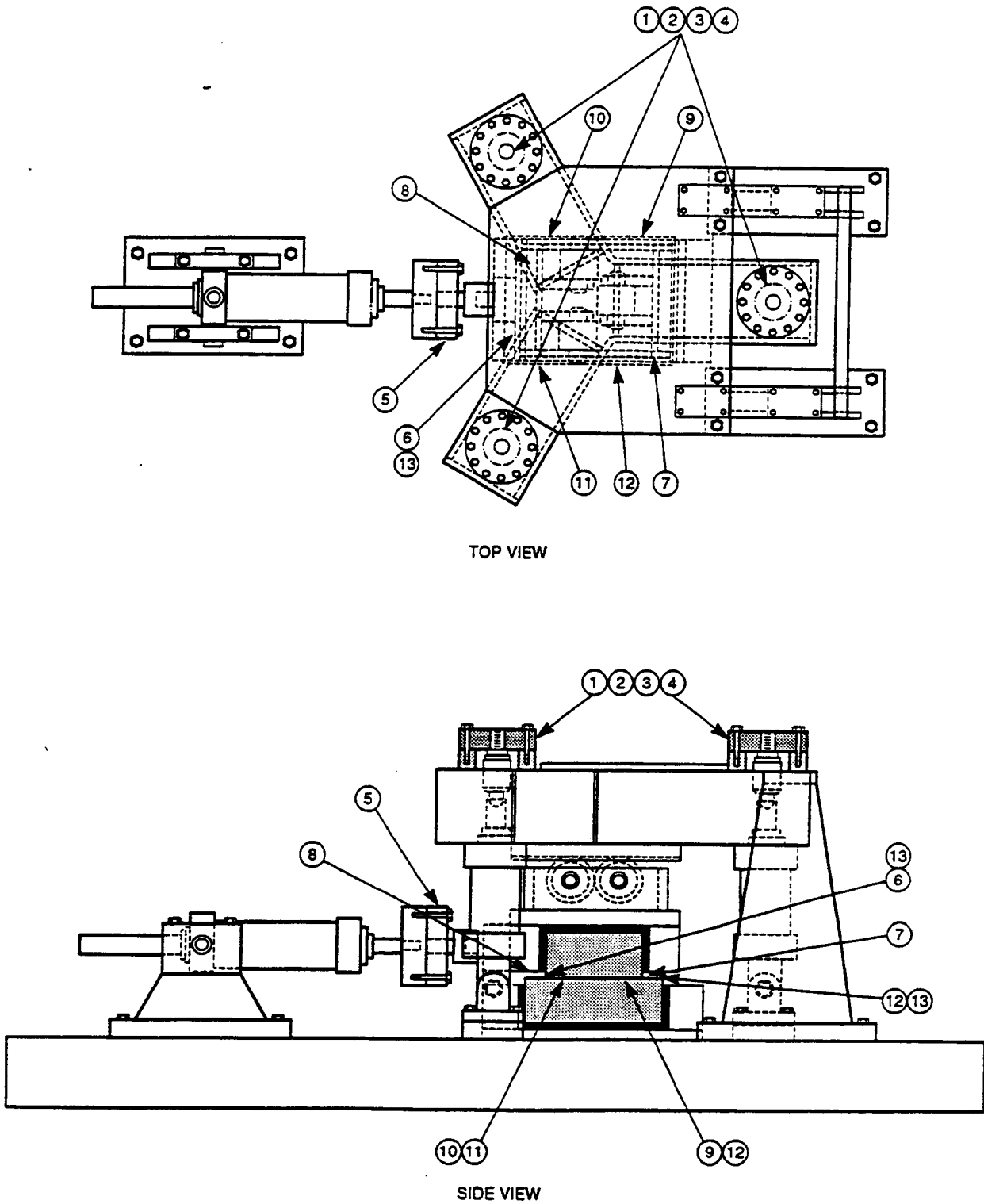
Figure 4-1. Assembly and instrumentation diagram for direct shear test apparatus (numbers in circles refer to location of instrumentation)
