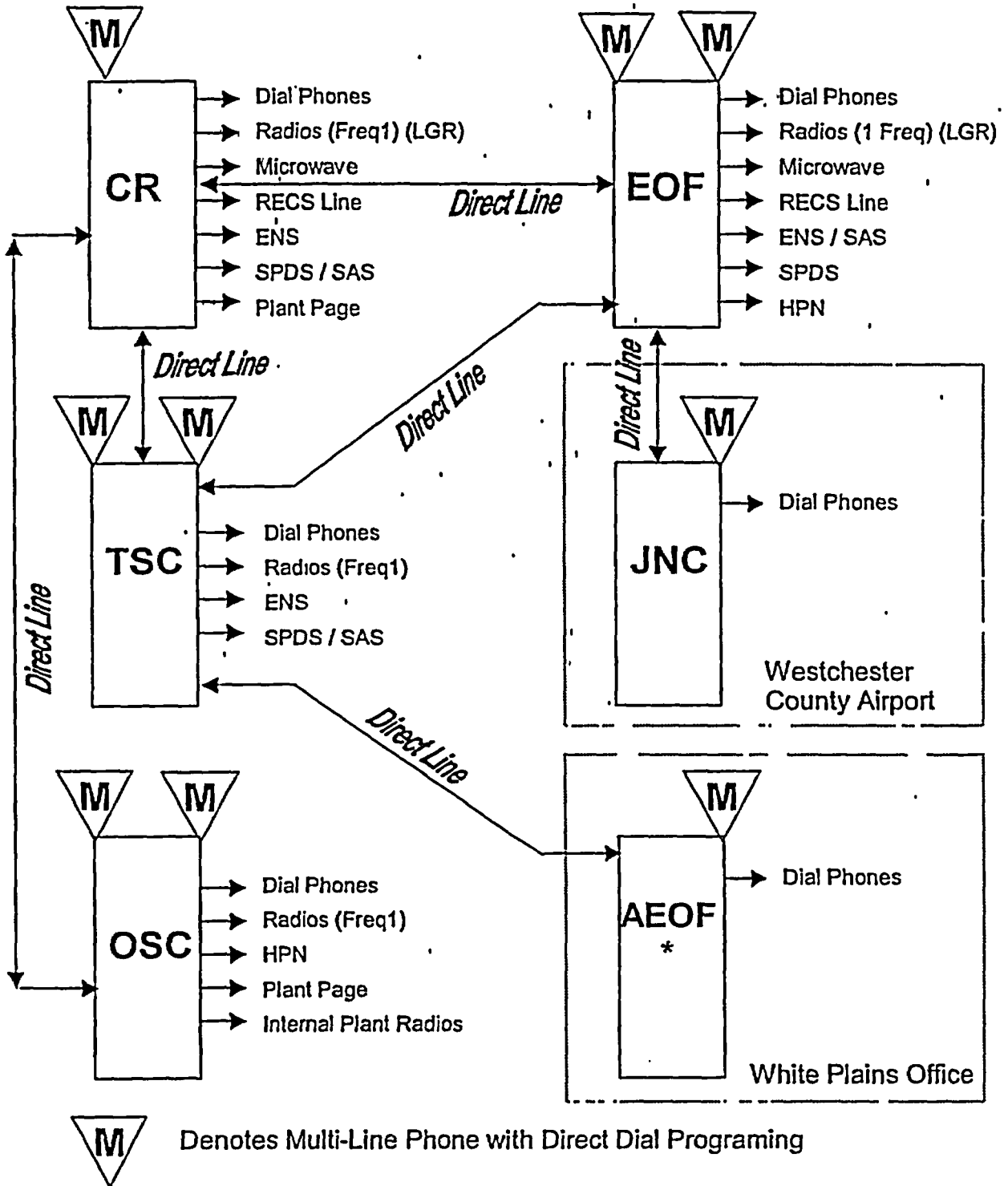
Figure F-1.3 Emergency Facilities Communications Systems
