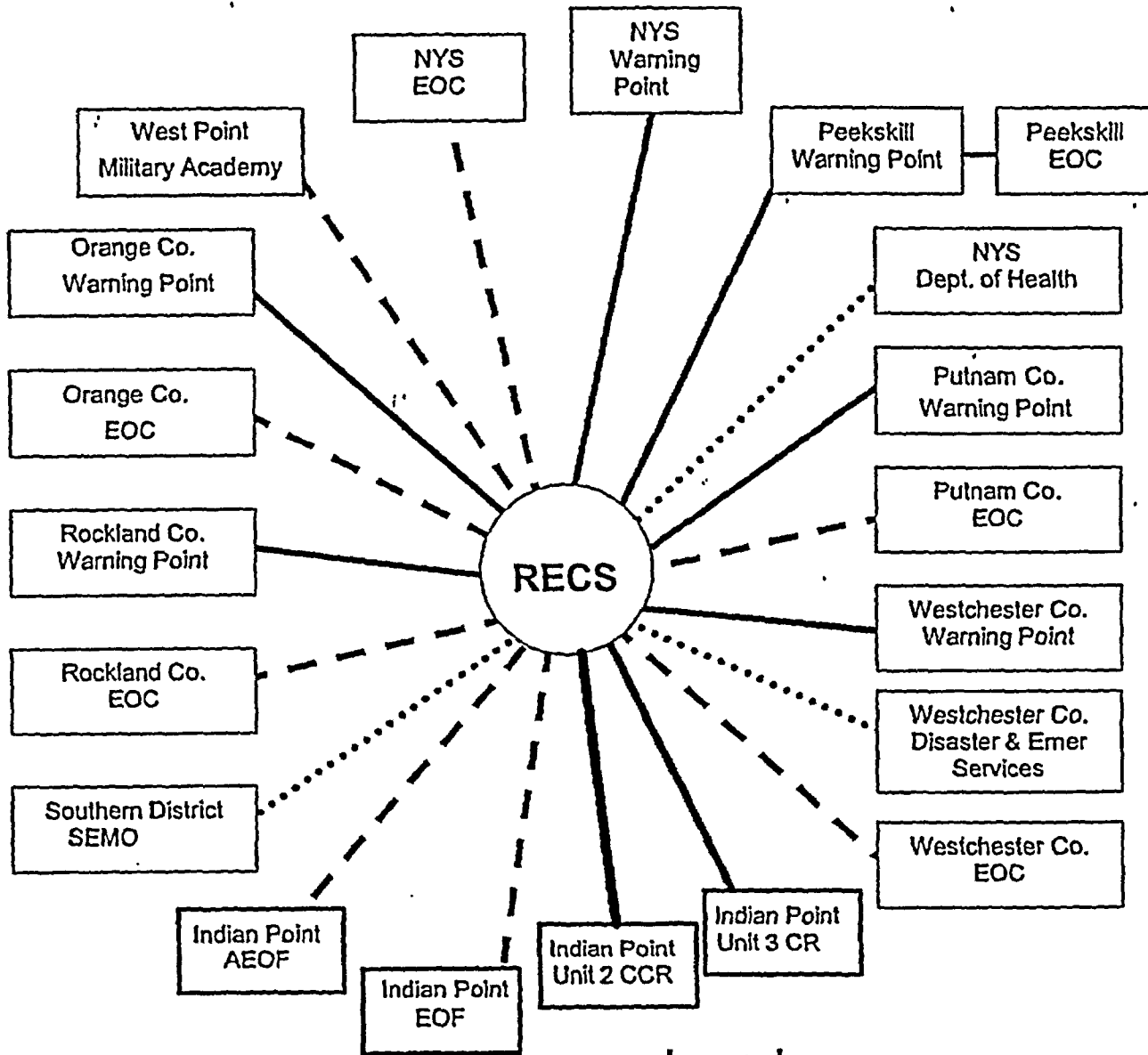
Figure F-1.2 Radiological Emergency Communications System
