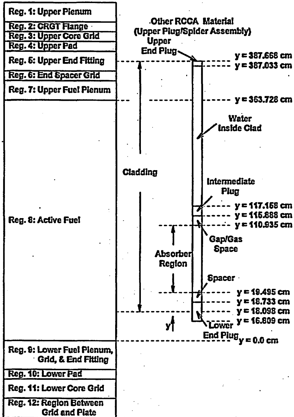
Figure 2-9. Black APSR Axial Dimensions for Mark-B4 Fuel Assembly (0% Withdrawn)
