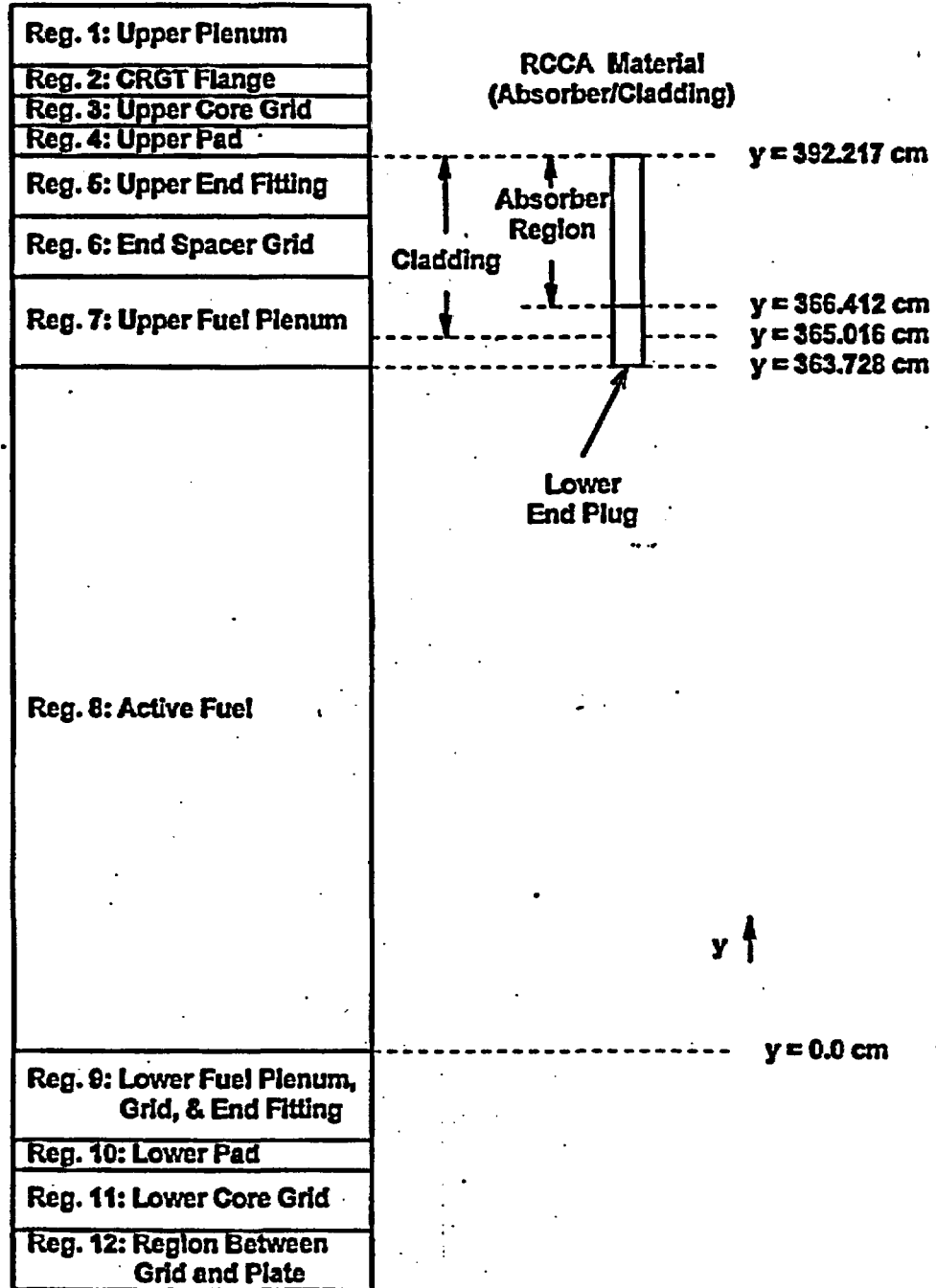
Figure 2-8. RCCA Axial Dimensions for Mark-B4 Fuel Assembly (100% Withdrawn)
