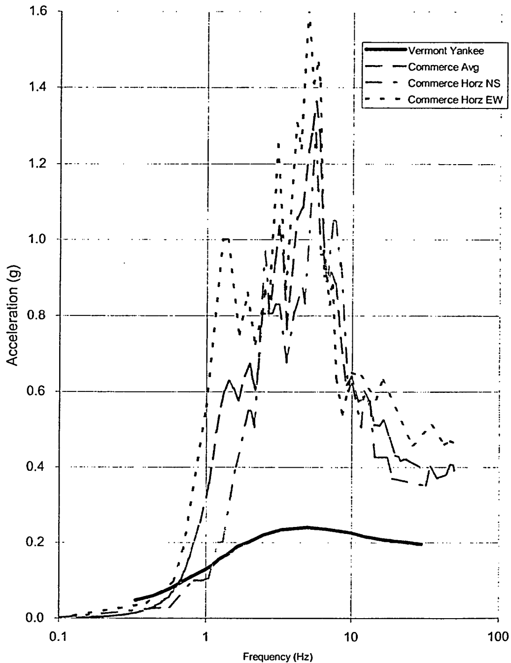
Figure 3-4 Comparison of Commerce Spectra to Vermont Yankee SSE Ground Spectrum
