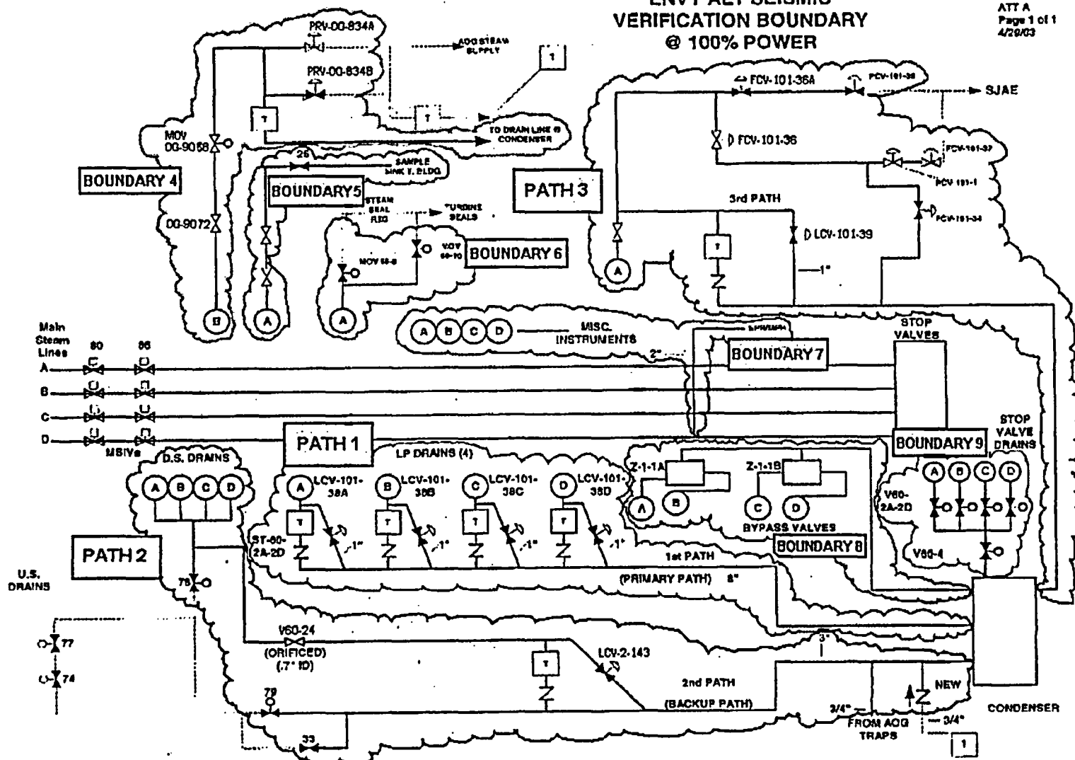
Figure Att.3-1: Path 3 Piping Definition
