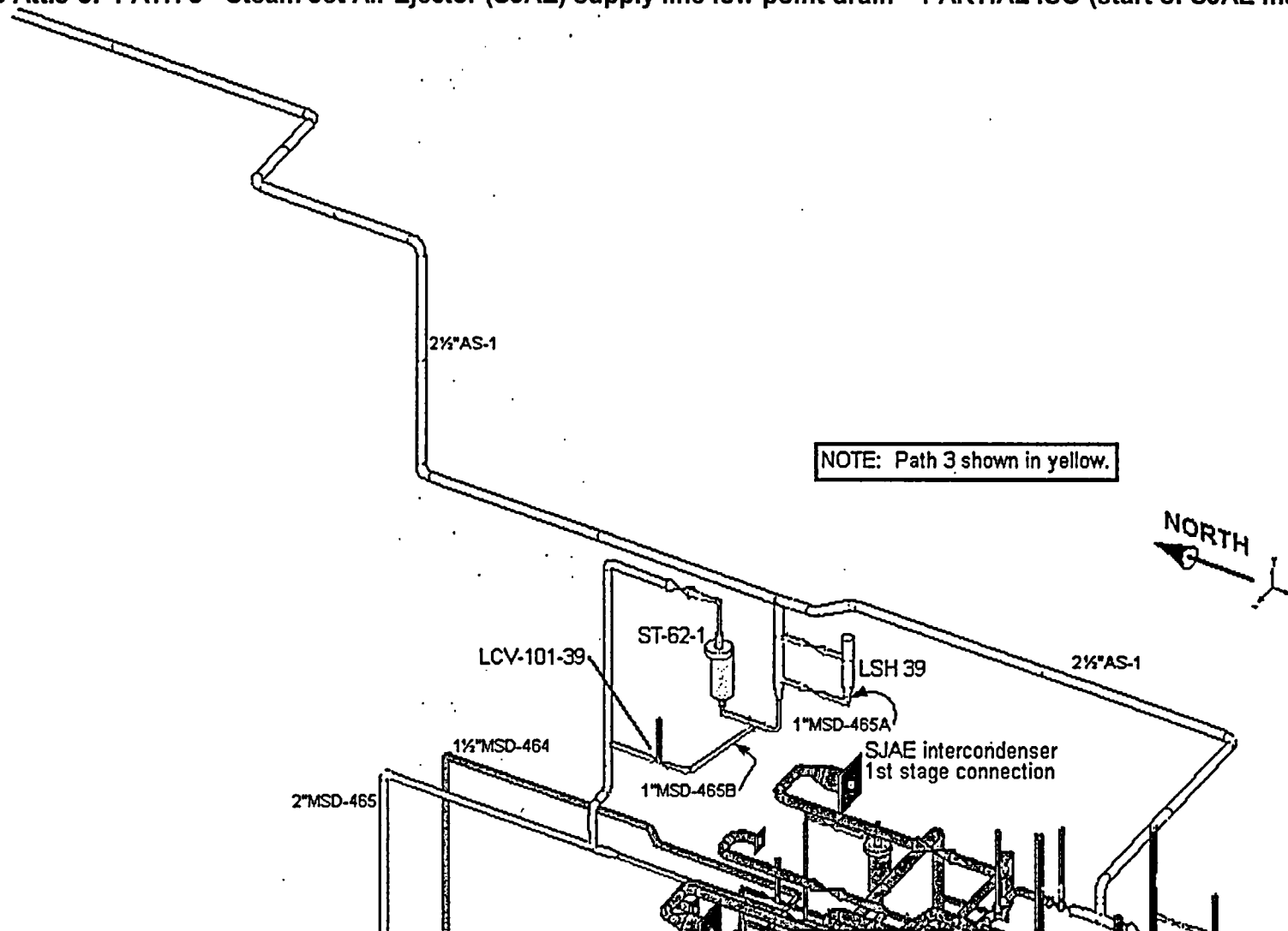
Figure Att.3-5: PATH 3 - Steam Jet Air Ejector (SJAE) supply line low point drain – PARTIAL ISO (start of SJAE manifold)
