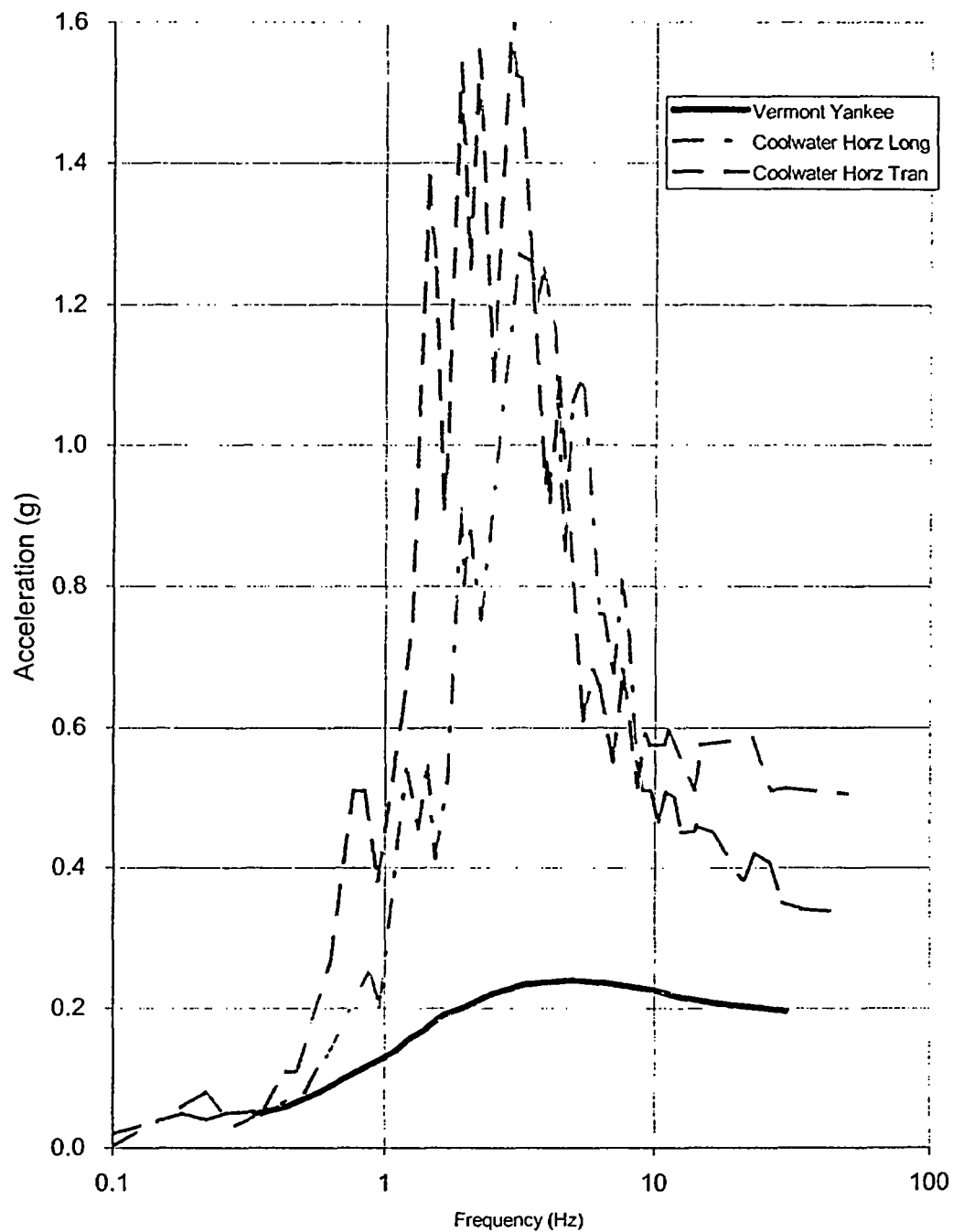
Figure 3-5 Comparison of Coolwater Spectra to Vermont Yankee SSE Ground Spectrum
