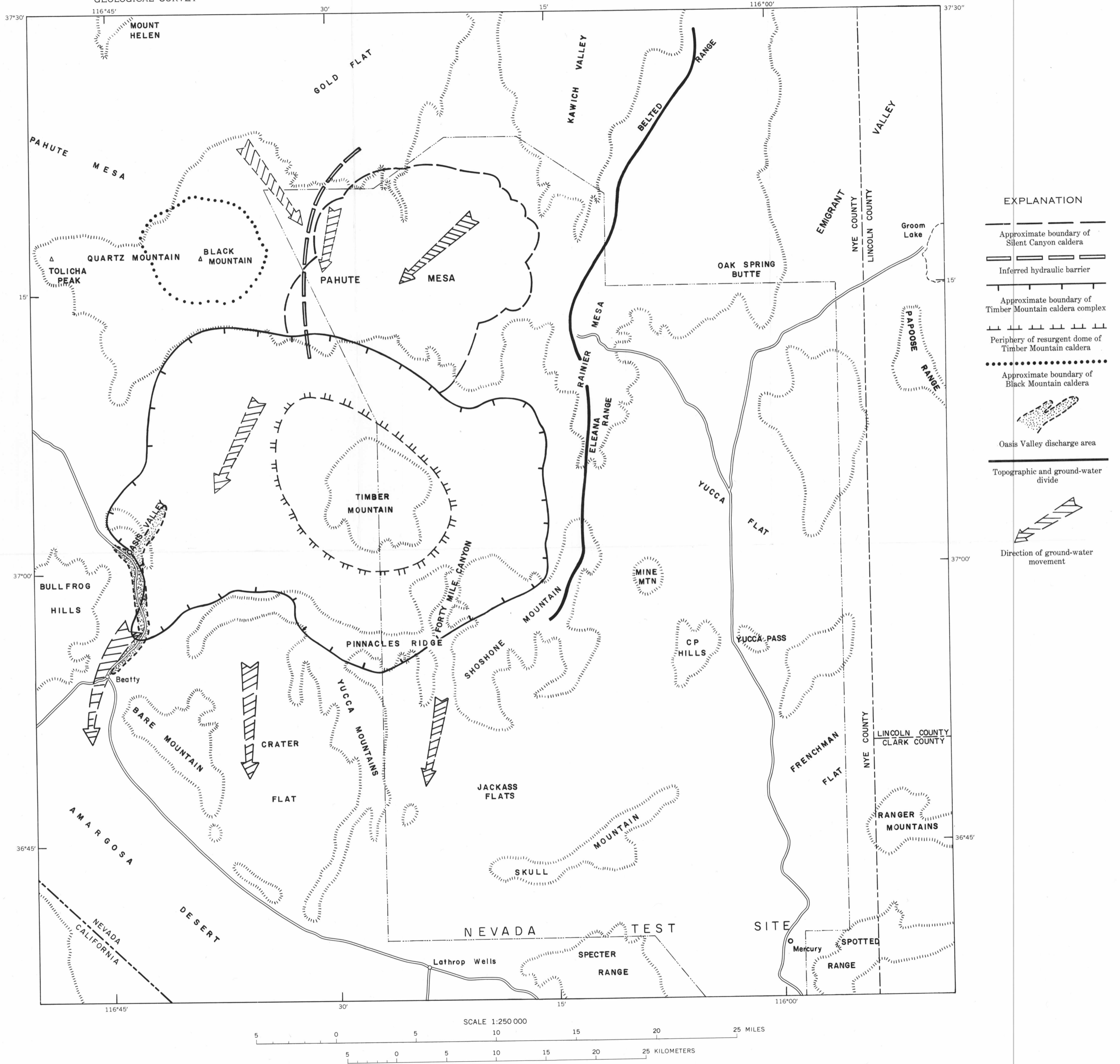
MAP SHOWING DIRECTION OF GROUND-WATER MOVEMENT FROM EASTERN PAHUTE MESA TOWARD DISCHARGE AREAS IN OASIS VALLEY AND AMARGOSA DESERT, NYE COUNTY, NEVADA
