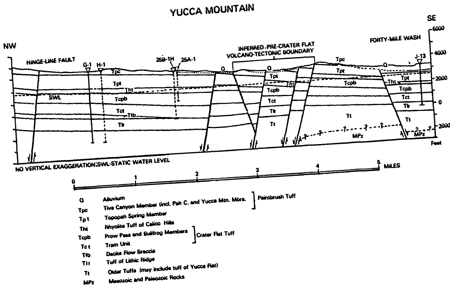
Fig. 8. Geologic cross section between drill holes USW-G1 and J-13 (modified from Maldonado, personal communication, 1981).
