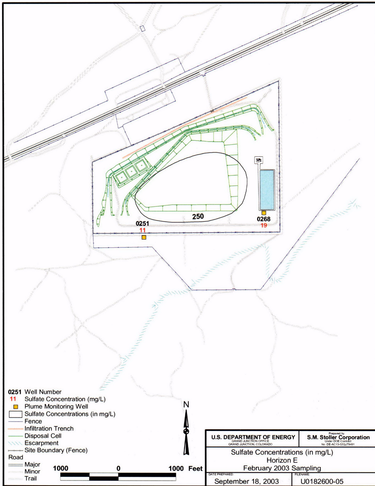
Figure 21b. February 2003 Horizon E Sulfate Ground Water Concentrations
