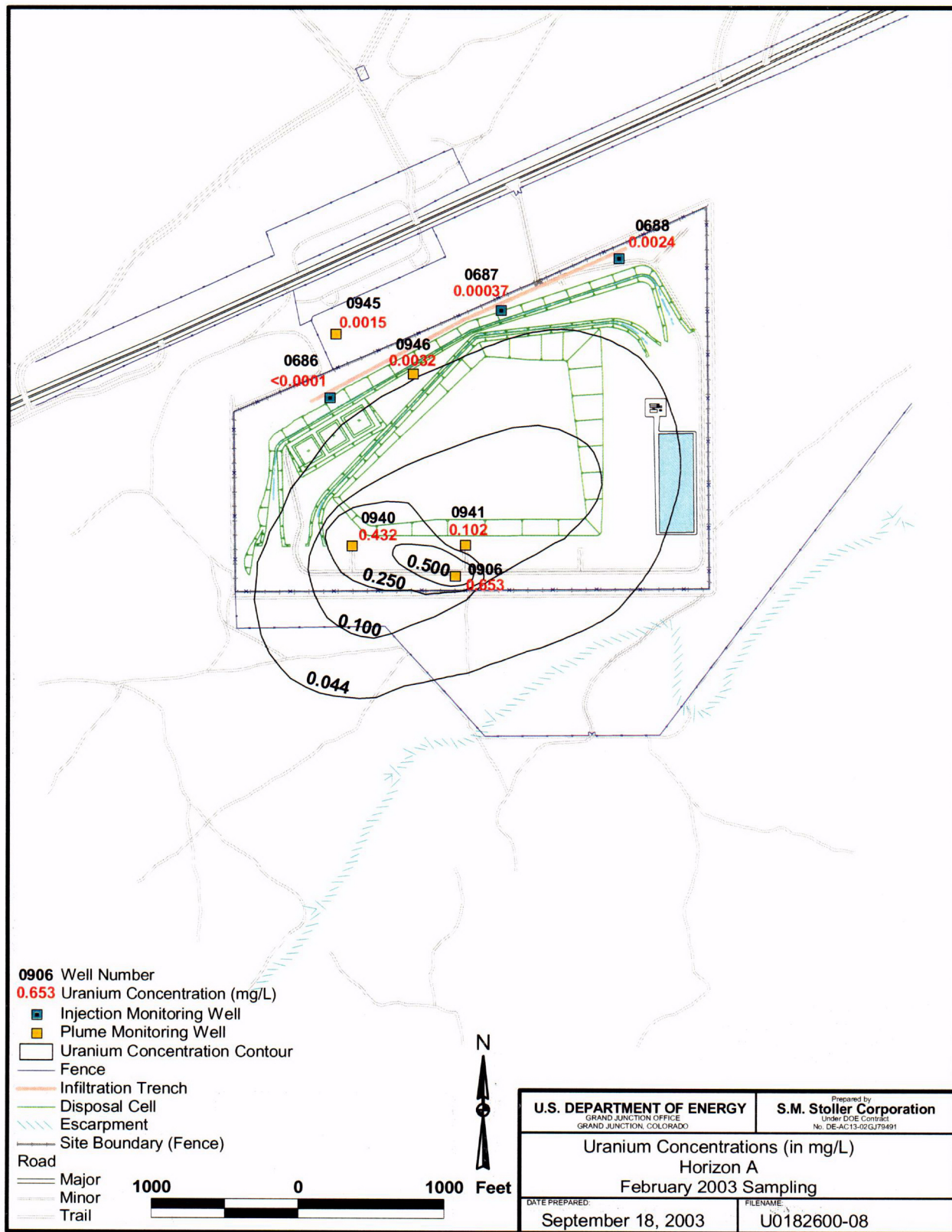
Figure 22b. February 2003 Horizon A Uranium Ground Water Concentrations
