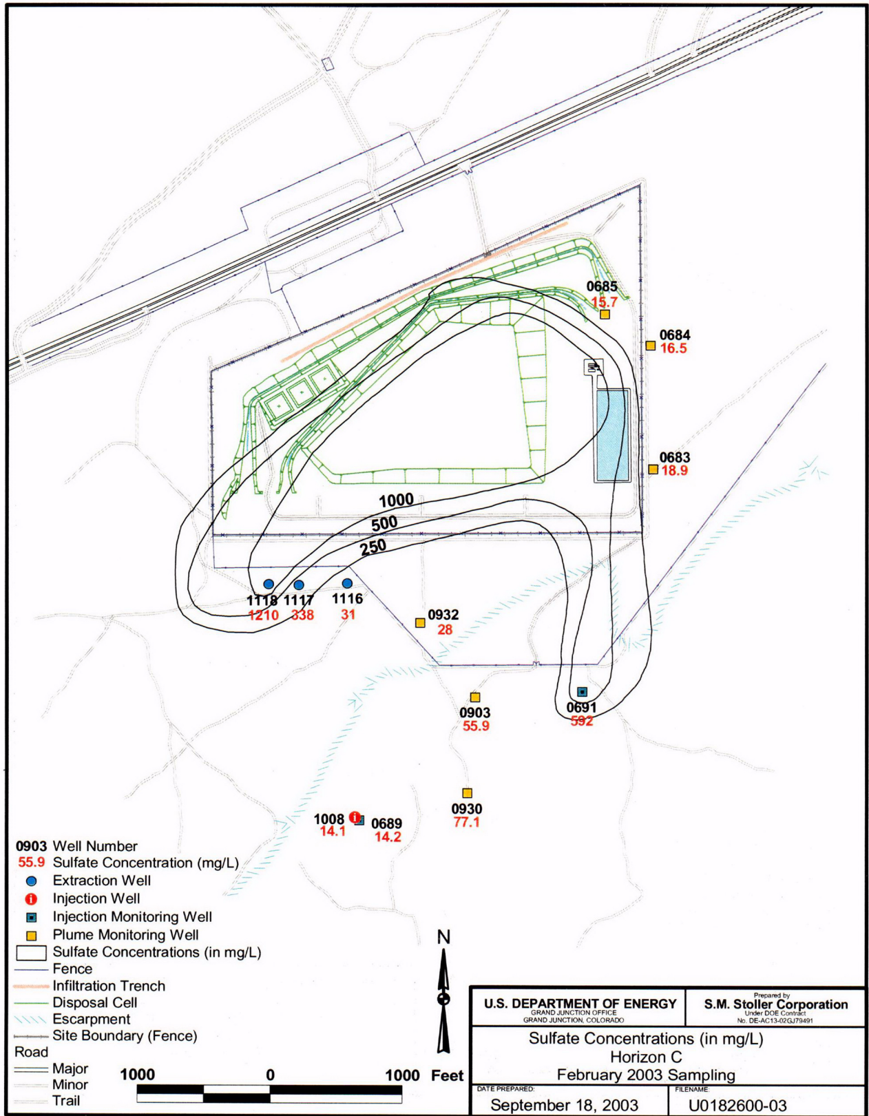
Figure 19b. February 2003 Horizon C Sulfate Ground Water Concentrations
