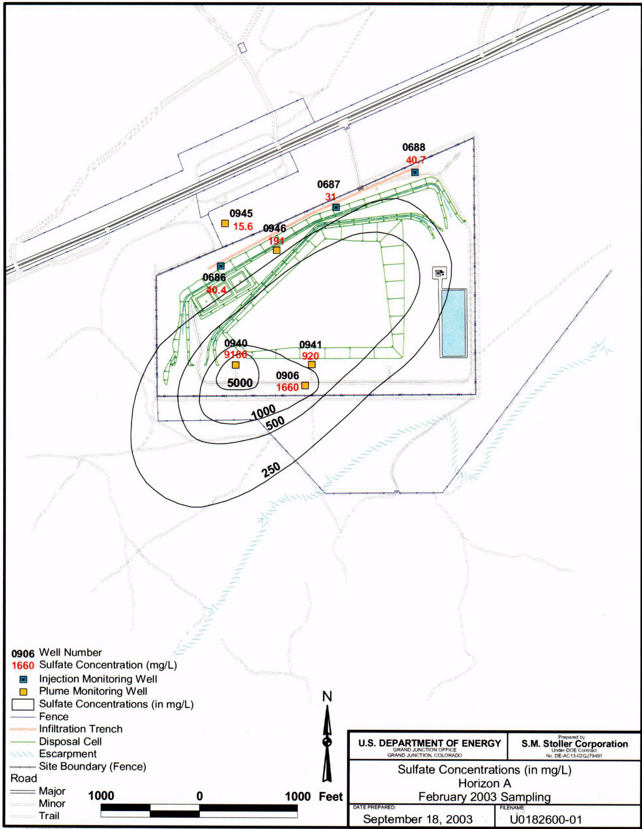
Figure 17b. February 2003 Horizon A Sulfate Ground Water Concentrations
