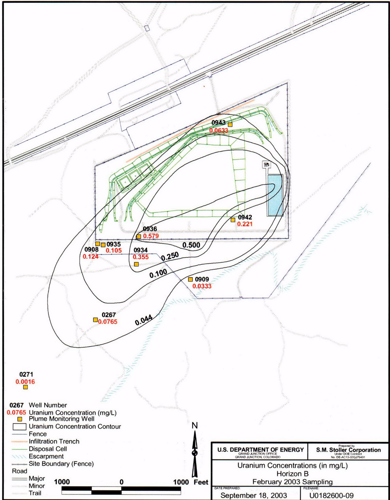
Figure 23b. February 2003 Horizon B Uranium Concentrations
