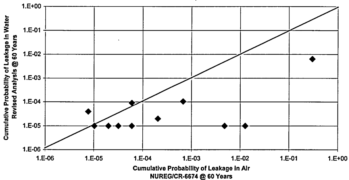
Figure 14. Comparison of 60-Year Cumulative Probabilities of Leakage in Environment for the Revised Analysis and NUREG/CR-6674 in Air.
