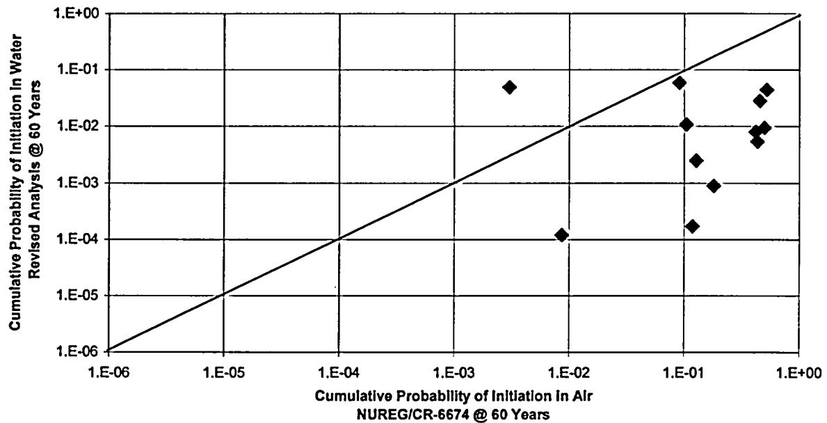
Figure 13. Comparison of 60-Year Cumulative Probabilities of Initiation in Environment for Revised Analysis and NUREG/CR-6674 in Air.
